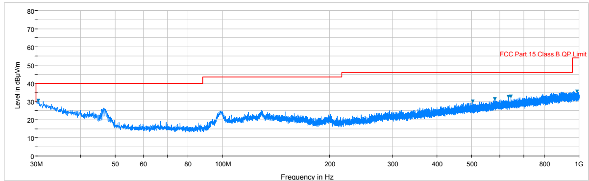
Plot 7-48. Radiated Spurious Plot below 1GHz (Pol. H)
