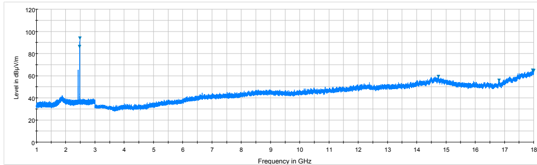
Plot 7-42. Radiated Spurious Plot above 1GHz (BT – Ch. 39, Ant. Pol. H)
