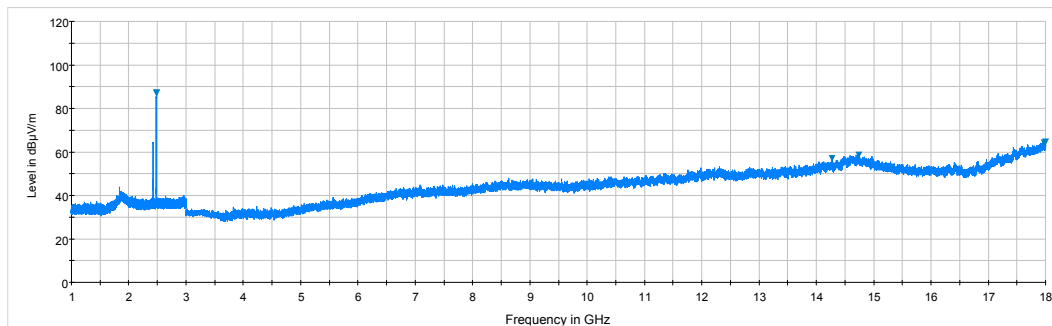
Plot 7-43. Radiated Spurious Plot above 1GHz (BT – Ch. 39, Ant. Pol. V)
