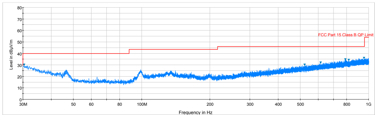
Plot 7-49. Radiated Spurious Plot below 1GHz (Pol. V)
