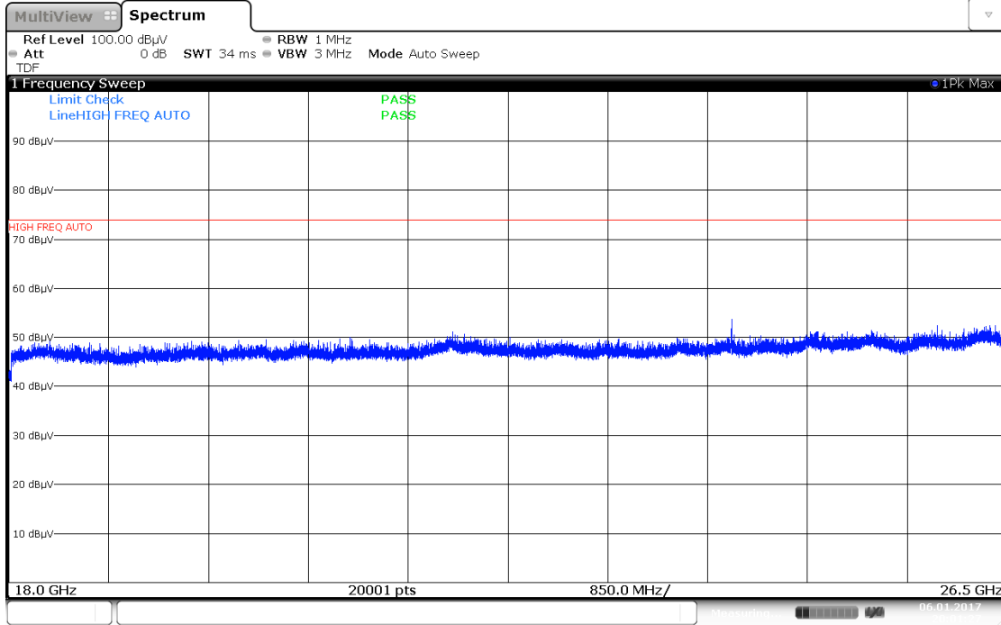
Plot 7-44. Radiated Spurious Plot above 18GHz (Pol. H)
