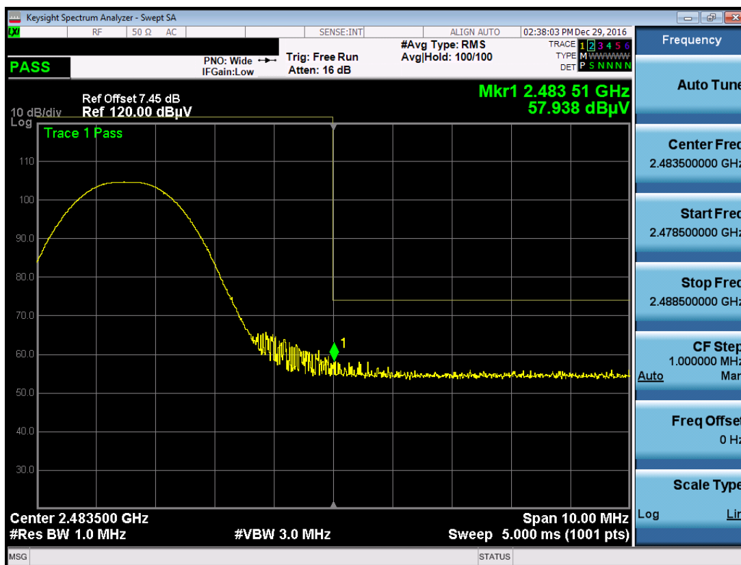
Plot 7-47. Radiated Restricted Upper Band Edge Measurement (Peak)
