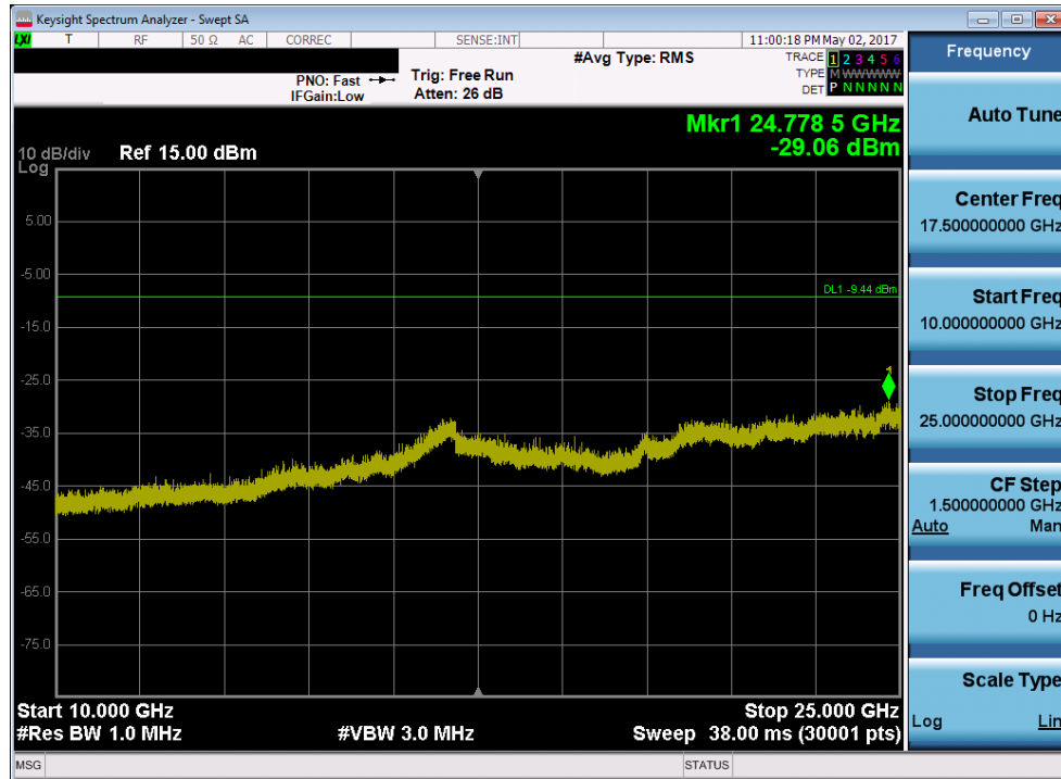
Plot 7-41. Conducted Spurious Plot (Bluetooth, 3Mbps – Ch. 78)
