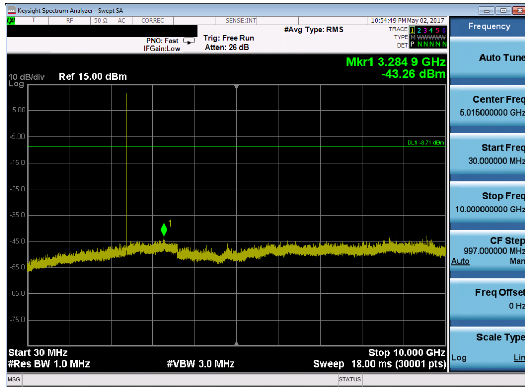
Plot 7-36. Conducted Spurious Plot (Bluetooth, 3Mbps – Ch. 0)
