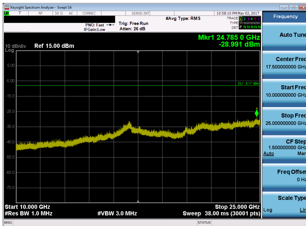
Plot 7-39. Conducted Spurious Plot (Bluetooth, 3Mbps – Ch. 39)
