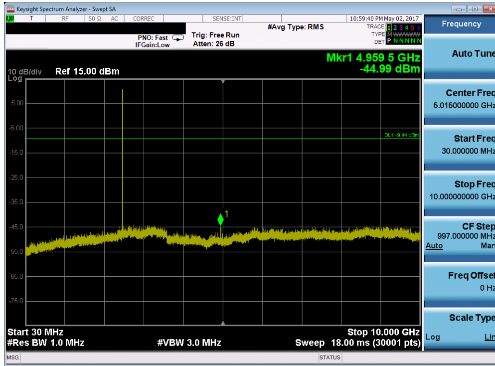
Plot 7-40. Conducted Spurious Plot (Bluetooth, 3Mbps – Ch. 78)
