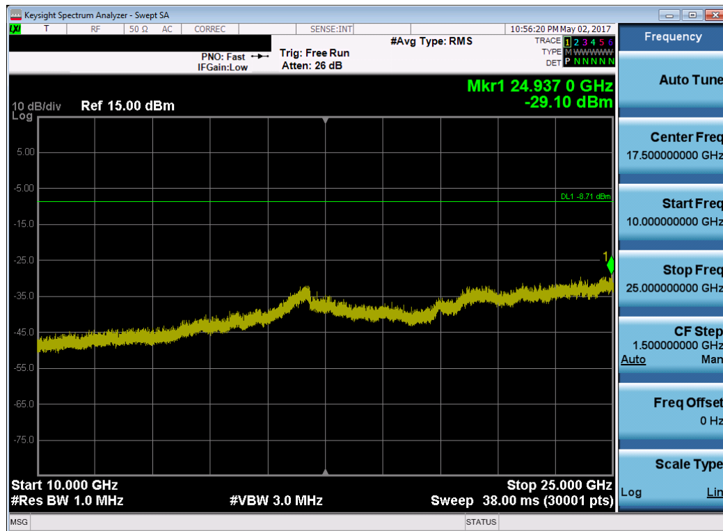
Plot 7-37. Conducted Spurious Plot (Bluetooth, 3Mbps – Ch. 0)
