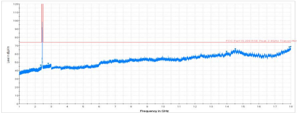
Plot 7-40. Radiated Spurious Plot above 1GHz (802.11b – Ch. 6, Ant. Pol. V)
