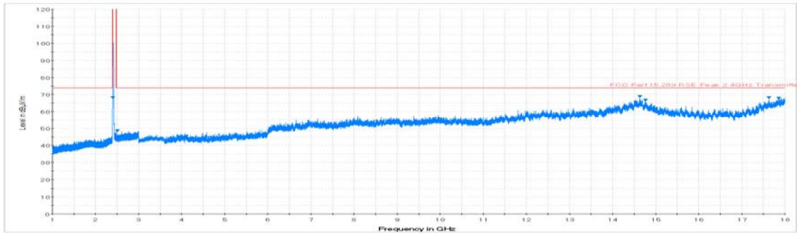
Plot 7-37. Radiated Spurious Plot above 1GHz (802.11b – Ch. 1, Ant. Pol. H)
