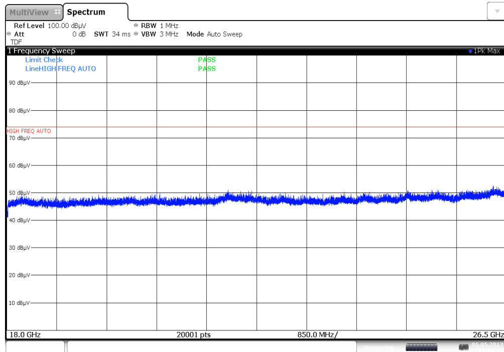
Plot 7-44. Radiated Spurious Plot above 18GHz (Pol. V)
