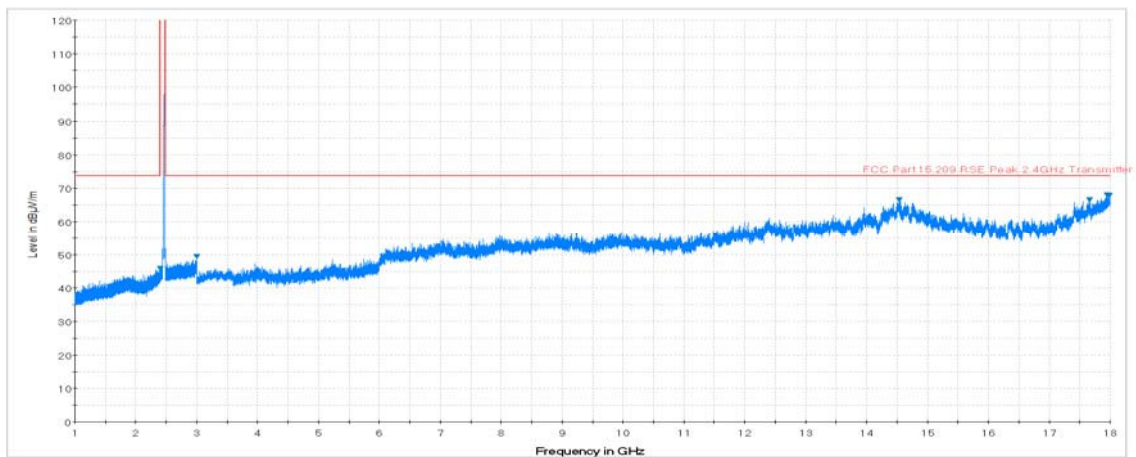
Plot 7-42. Radiated Spurious Plot above 1GHz (802.11b – Ch. 11, Ant. Pol. V)
