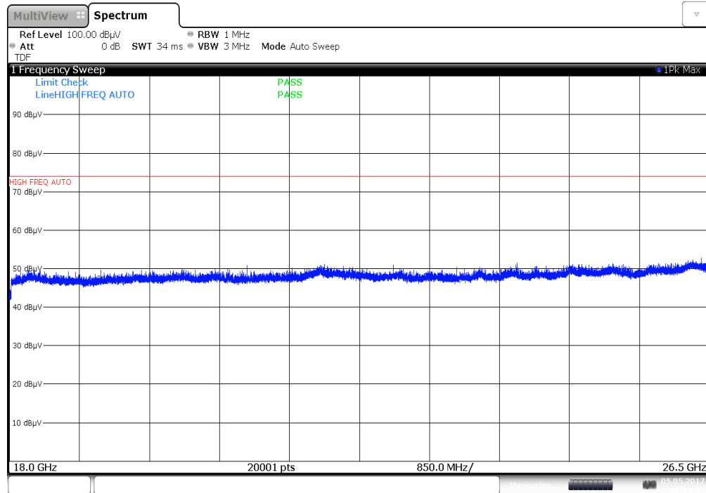
Plot 7-43. Radiated Spurious Plot above 18GHz (Pol. H)
