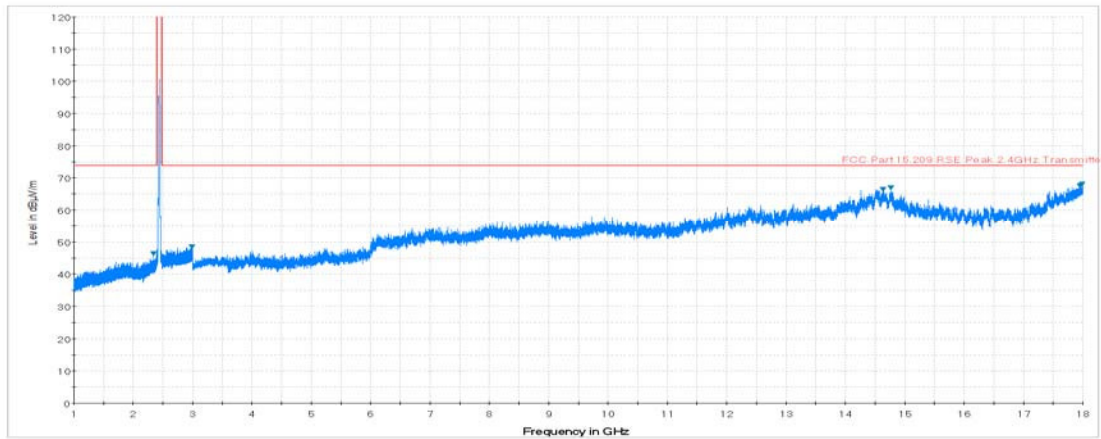
Plot 7-39. Radiated Spurious Plot above 1GHz (802.11b – Ch. 6, Ant. Pol. H)
