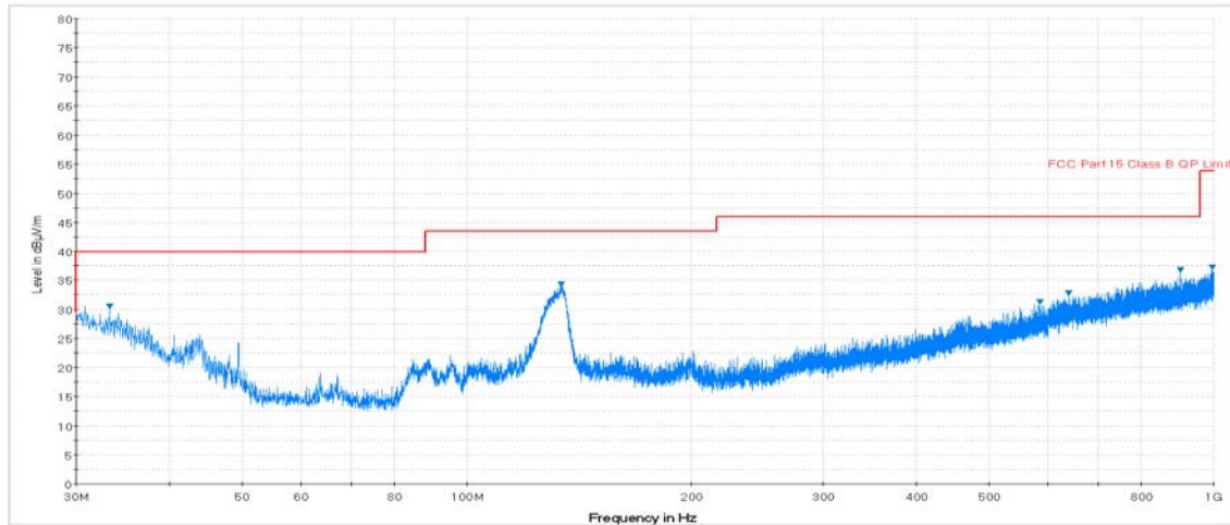
Plot 7-51. Radiated Spurious Plot below 1GHz (Pol. H)
