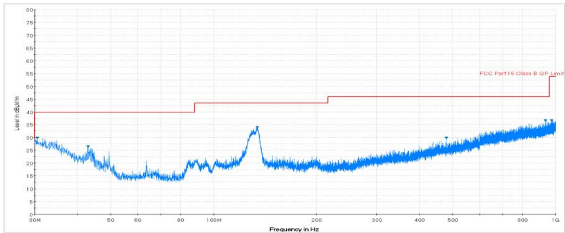
Plot 7-52. Radiated Spurious Plot below 1GHz (Pol. V)
