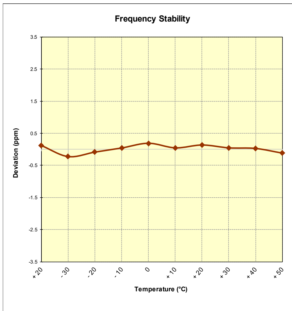
Figure 7-12. Frequency Stability Graph (PCS WCDMA Mode – Ch. 9400)
