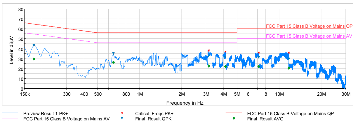
Plot 7-21. Line Conducted Plot with Bluetooth LE (N)
