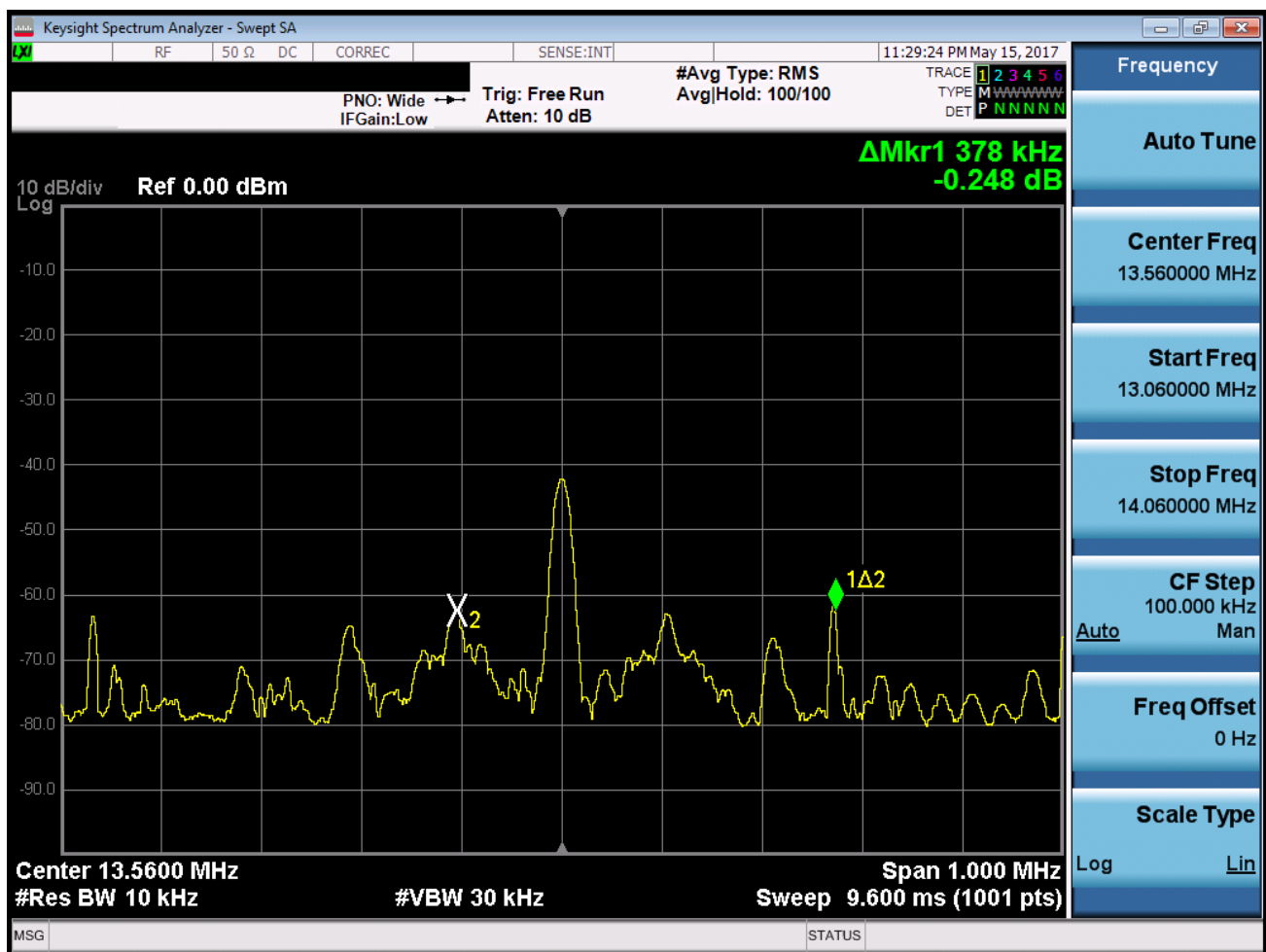
Figure 7-2. 20dB Bandwidth Plot
