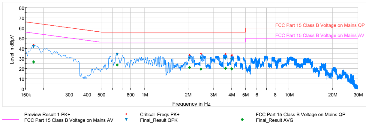
Plot 7-53. Line Conducted Plot with 802.11b (L1)
