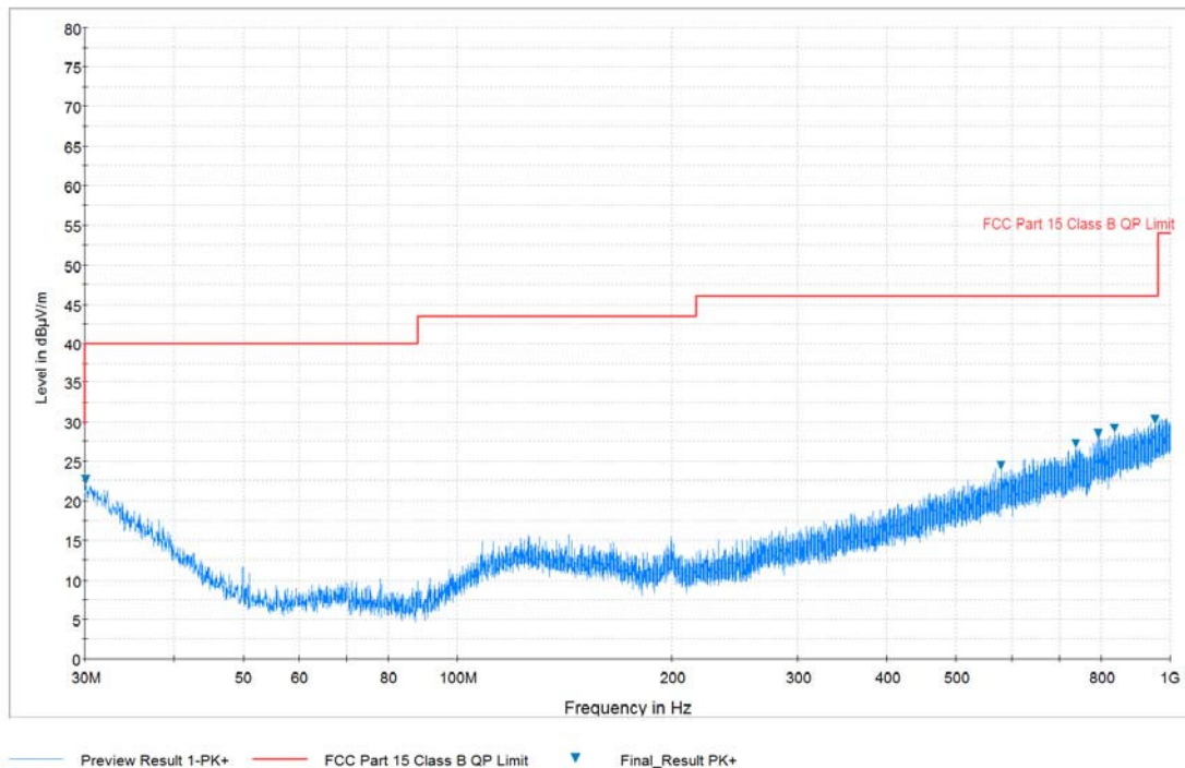
Plot 7-52. Radiated Spurious Plot below 1GHz (Pol. V)
