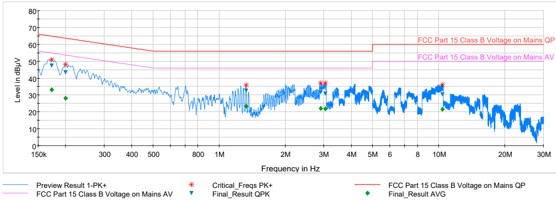
Plot 7-54. Line Conducted Plot with 802.11b (N)
