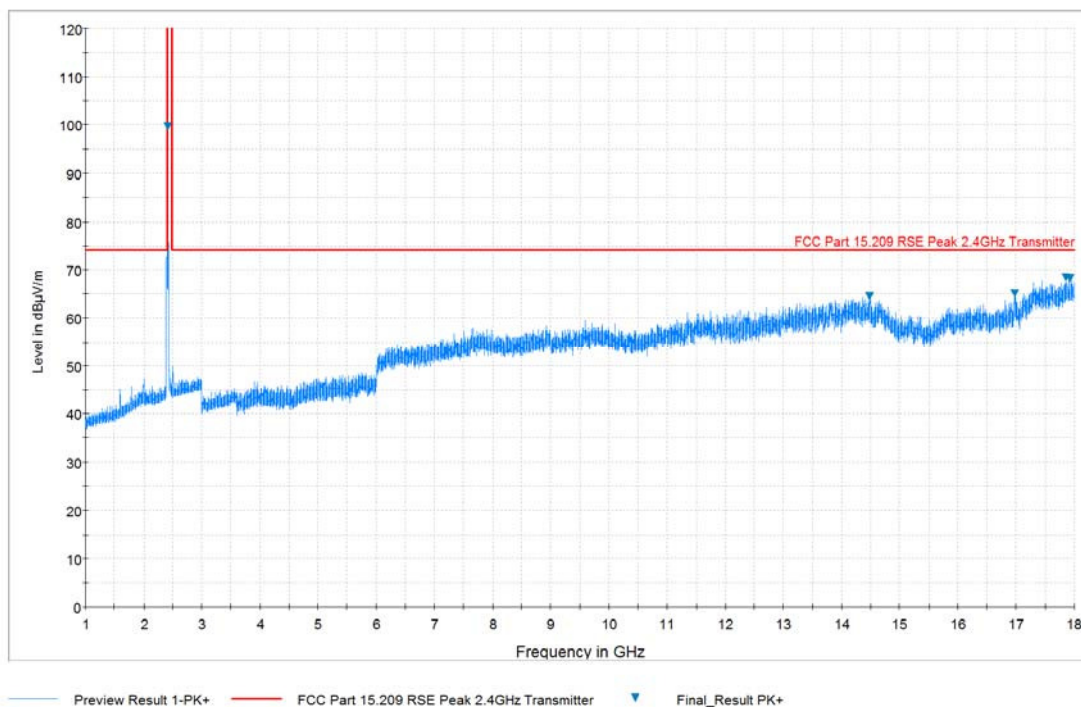
Plot 7-31. Radiated Spurious Plot above 1GHz (802.11b – Ch. 1, Ant. Pol. H)
