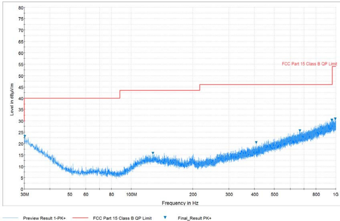
Plot 7-51. Radiated Spurious Plot below 1GHz (Pol. H)
