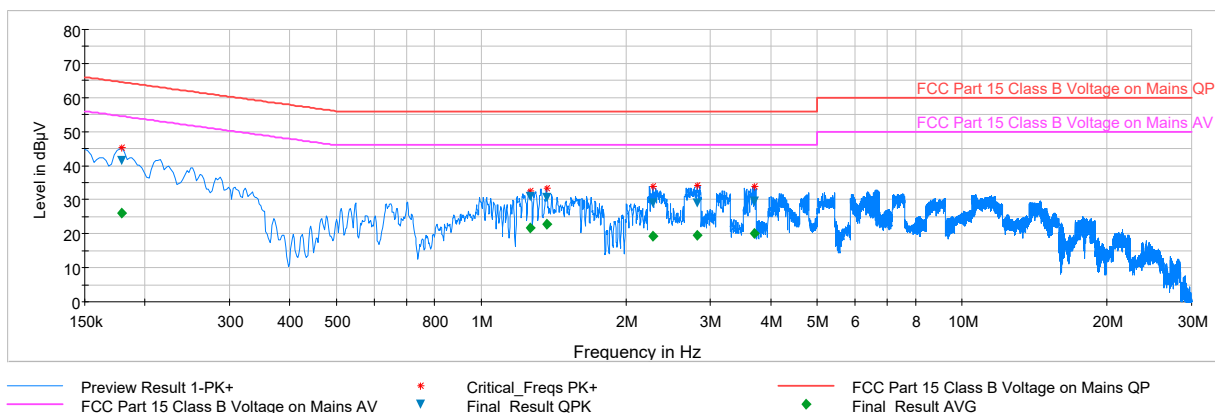
Plot 7-20. Line Conducted Plot with Bluetooth LE (L1)
