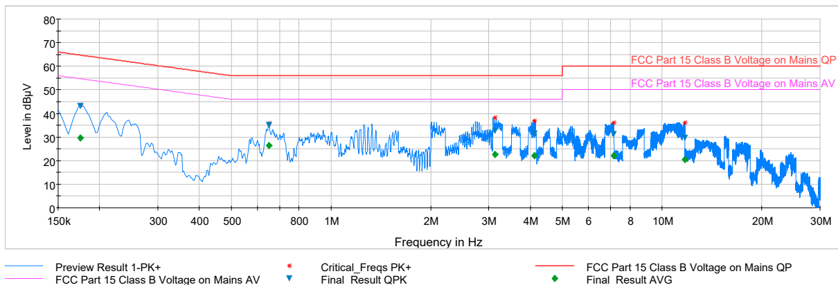
Plot 7-21. Line Conducted Plot with Bluetooth LE (N)
