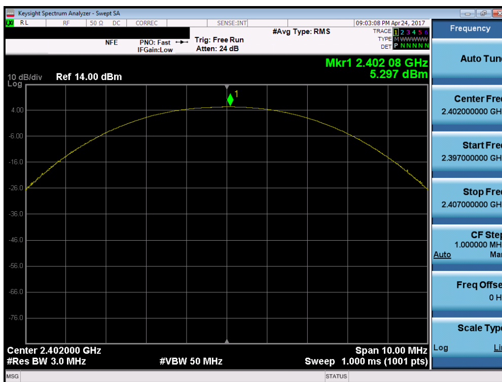
Plot 7-4. Peak Power Plot (Bluetooth (LE), 1Mbps - Ch. 0)
