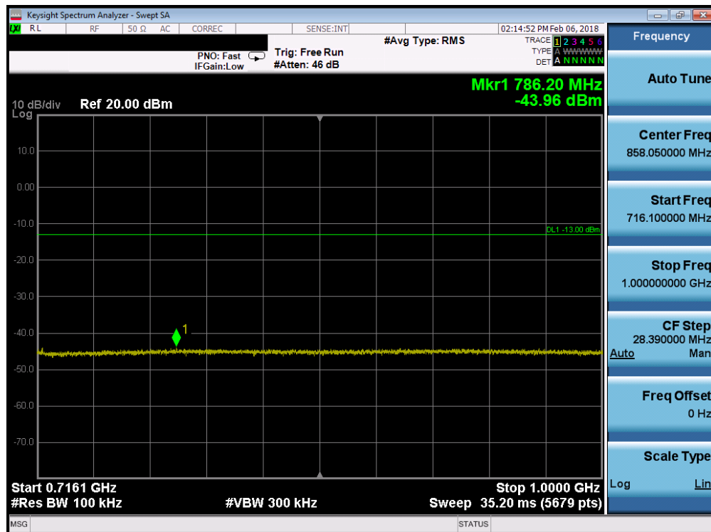
Plot 7-56. Conducted Spurious Plot (Band 12 - 10.0MHz QPSK - RB Size 1, RB Offset 0 - High Channel)
