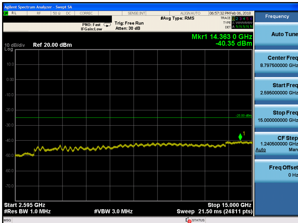
Plot 7-92. Conducted Spurious Plot (Band 7 - 10.0MHz QPSK - RB Size 1, RB Offset 0 - High Channel)
