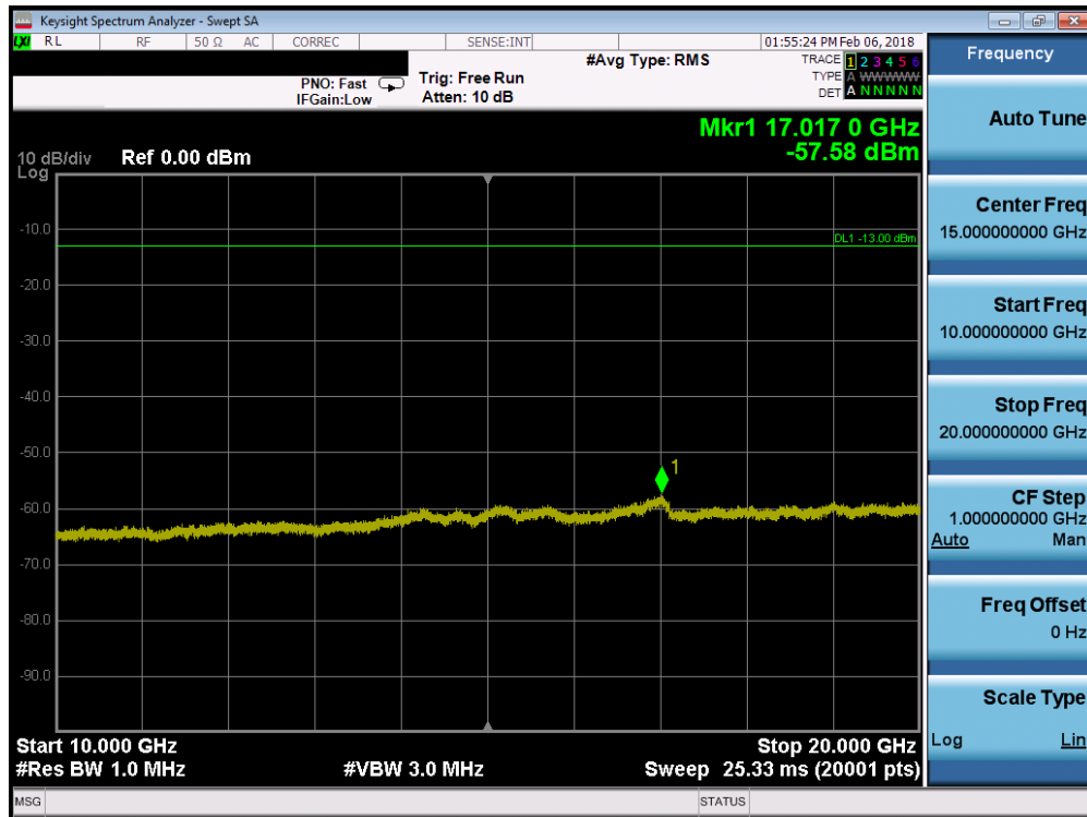
Plot 7-84. Conducted Spurious Plot (Band 2 - 5.0MHz QPSK - RB Size 1, RB Offset 0 - High Channel)
