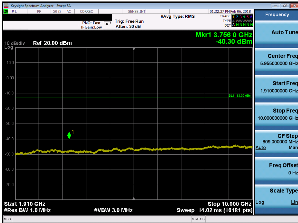
Plot 7-80. Conducted Spurious Plot (Band 2 - 5.0MHz QPSK - RB Size 1, RB Offset 0 - Mid Channel)
