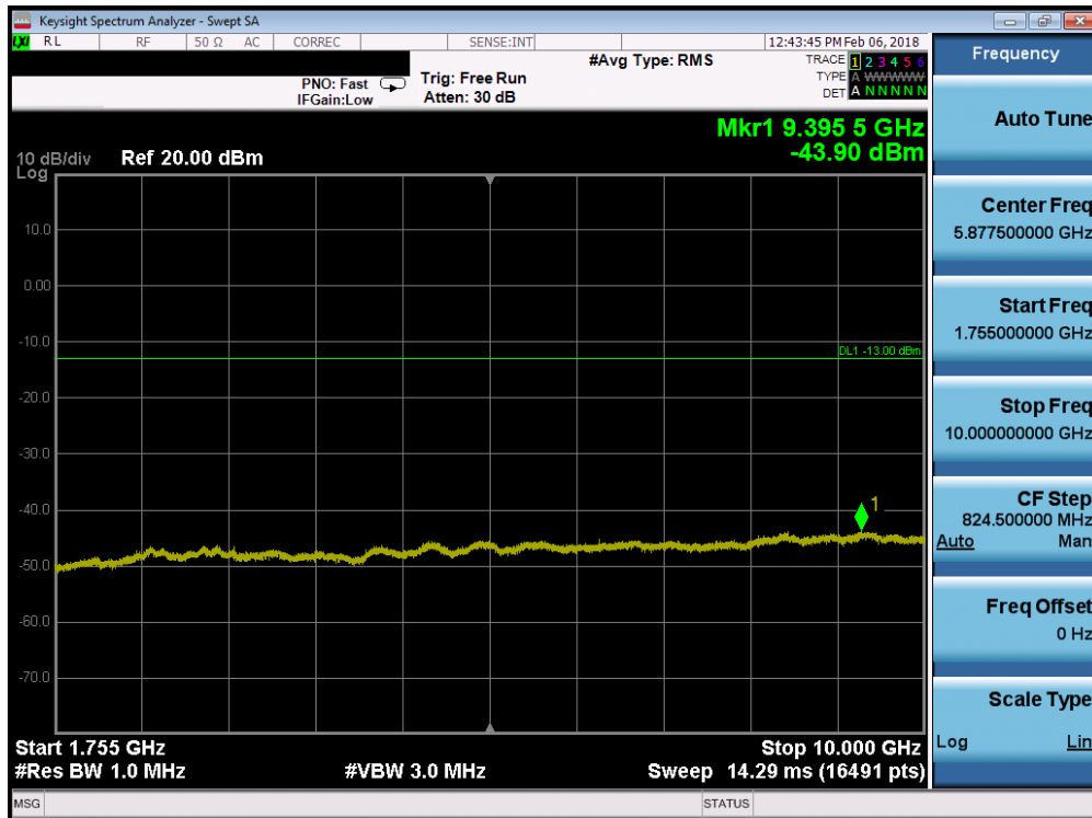
Plot 7-71. Conducted Spurious Plot (Band 4 - 10.0MHz QPSK - RB Size 1, RB Offset 0 - Mid Channel)
