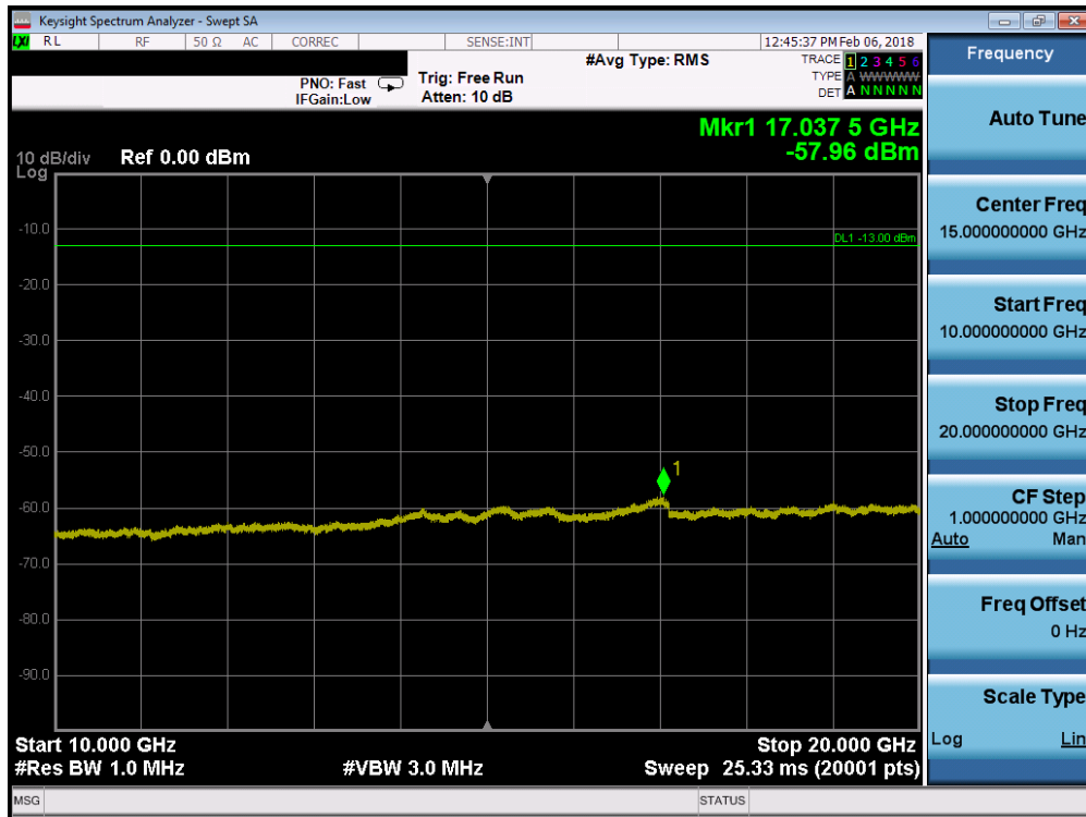
Plot 7-69. Conducted Spurious Plot (Band 4 - 10.0MHz QPSK - RB Size 1, RB Offset 0 - Low Channel)
