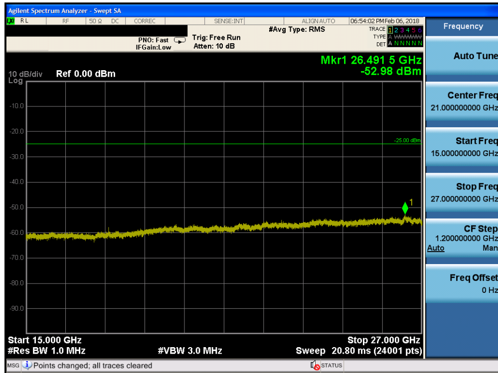
Plot 7-87. Conducted Spurious Plot (Band 7 - 10.0MHz QPSK - RB Size 1, RB Offset 0 - Low Channel)
