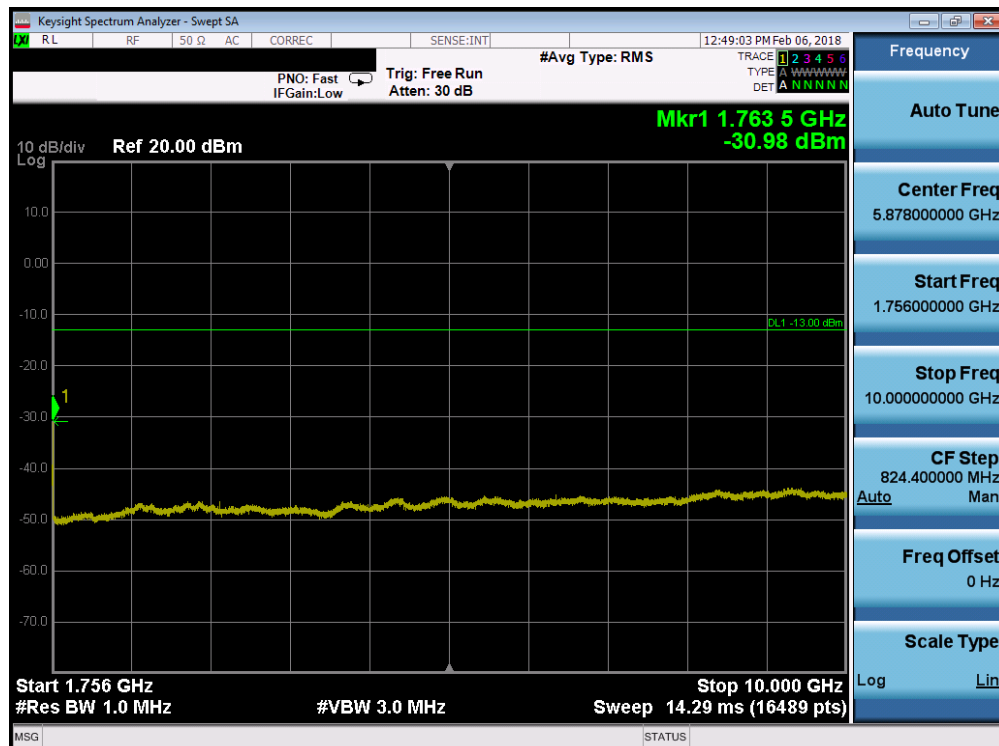
Plot 7-74. Conducted Spurious Plot (Band 4 - 10.0MHz QPSK - RB Size 1, RB Offset 0 - High Channel)
