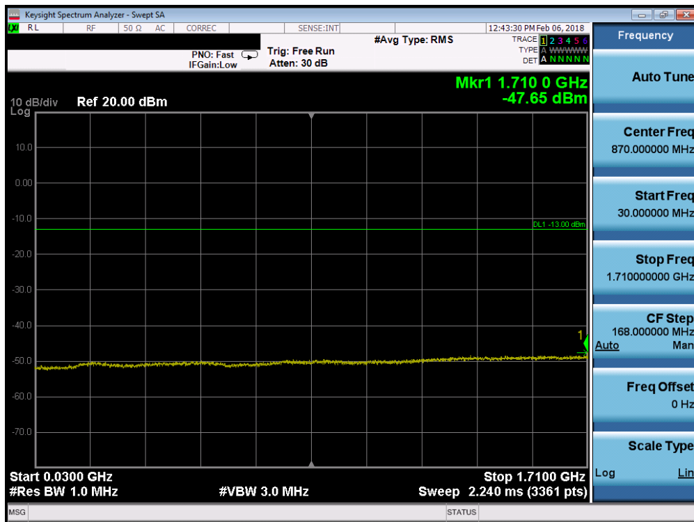
Plot 7-70. Conducted Spurious Plot (Band 4 - 10.0MHz QPSK - RB Size 1, RB Offset 0 - Mid Channel)
