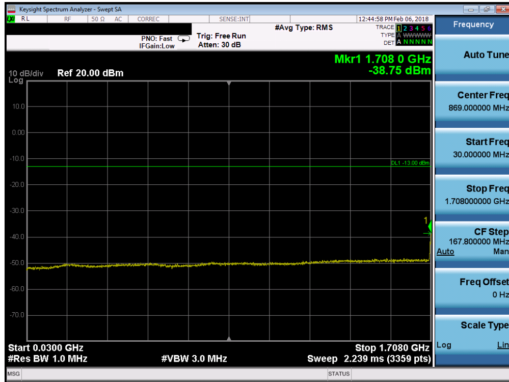
Plot 7-67. Conducted Spurious Plot (Band 4 - 10.0MHz QPSK - RB Size 1, RB Offset 0 - Low Channel)
