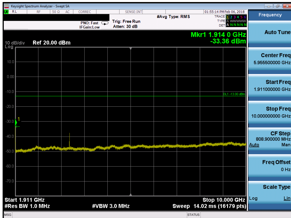
Plot 7-83. Conducted Spurious Plot (Band 2 - 5.0MHz QPSK - RB Size 1, RB Offset 0 - High Channel)
