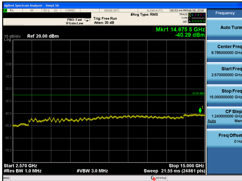
Plot 7-86. Conducted Spurious Plot (Band 7 - 10.0MHz QPSK - RB Size 1, RB Offset 0 - Low Channel)
