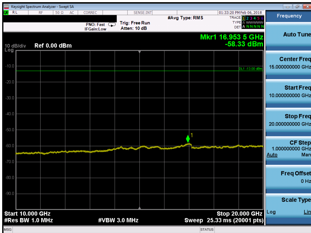
Plot 7-81. Conducted Spurious Plot (Band 2 - 5.0MHz QPSK - RB Size 1, RB Offset 0 - Mid Channel)
