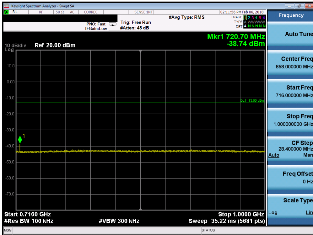
Plot 7-53. Conducted Spurious Plot (Band 12 - 10.0MHz QPSK - RB Size 1, RB Offset 0 - Mid Channel)
