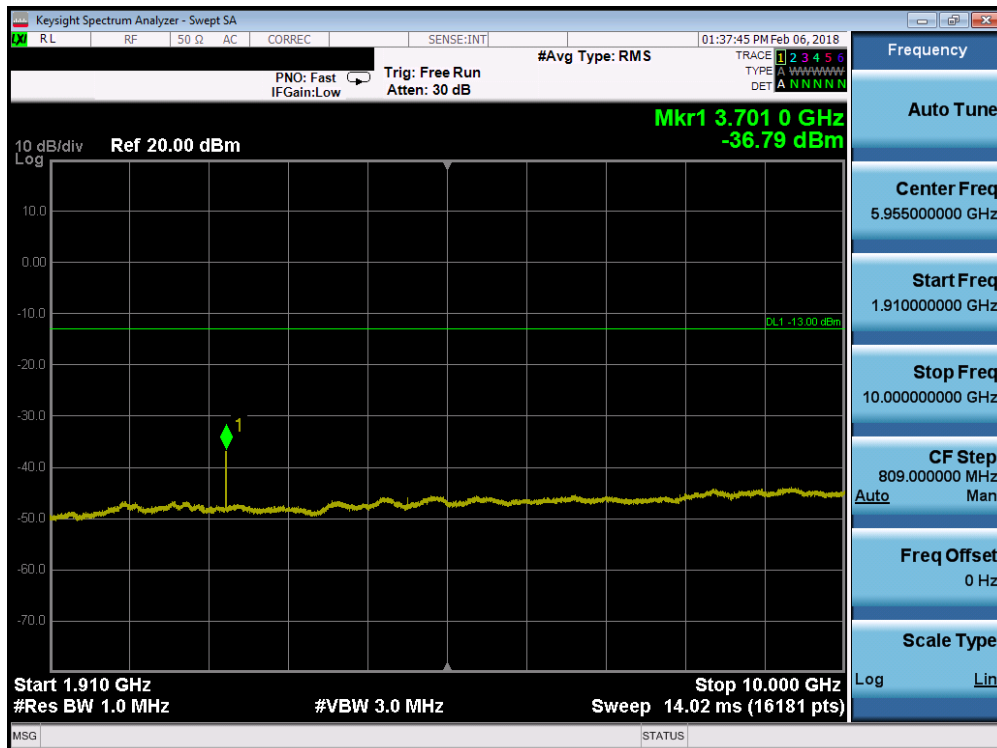
Plot 7-77. Conducted Spurious Plot (Band 2 - 5.0MHz QPSK - RB Size 1, RB Offset 0 - Low Channel)
