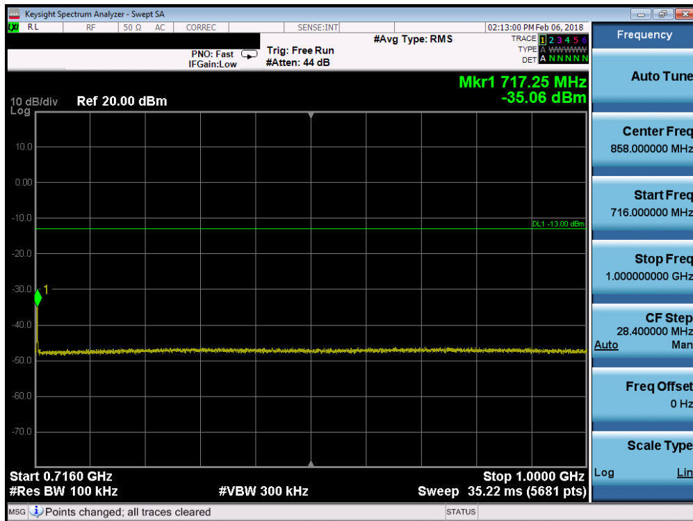
Plot 7-50. Conducted Spurious Plot (Band 12 - 10.0MHz QPSK - RB Size 1, RB Offset 0 - Low Channel)
