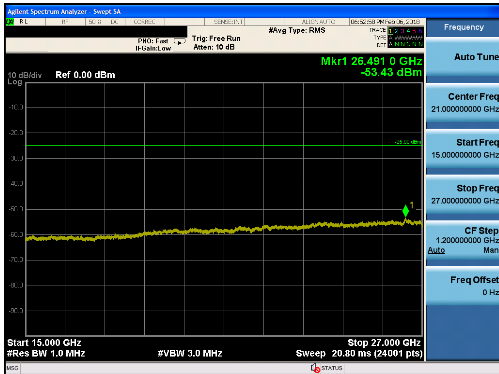
Plot 7-90. Conducted Spurious Plot (Band 7 - 10.0MHz QPSK - RB Size 1, RB Offset 0 - Mid Channel)
