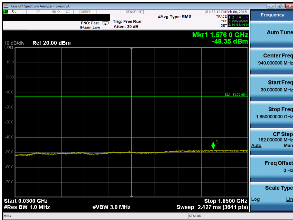
Plot 7-79. Conducted Spurious Plot (Band 2 - 5.0MHz QPSK - RB Size 1, RB Offset 0 - Mid Channel)
