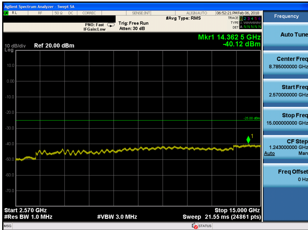
Plot 7-89. Conducted Spurious Plot (Band 7 - 10.0MHz QPSK - RB Size 1, RB Offset 0 - Mid Channel)
