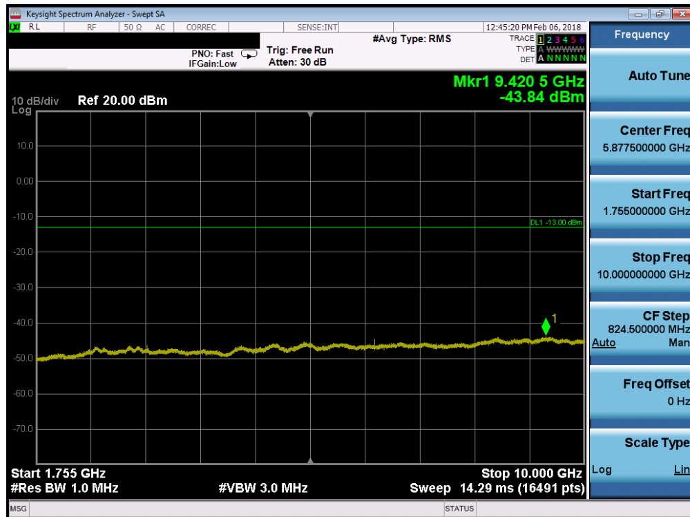
Plot 7-68. Conducted Spurious Plot (Band 4 - 10.0MHz QPSK - RB Size 1, RB Offset 0 - Low Channel)
