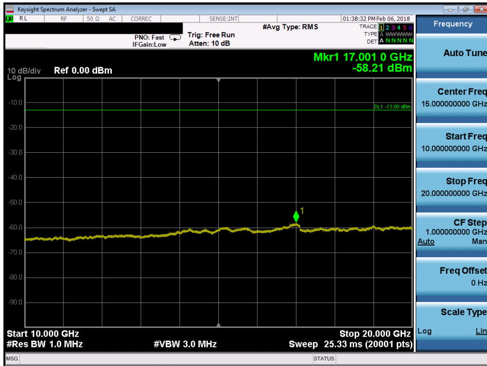
Plot 7-78. Conducted Spurious Plot (Band 2 - 5.0MHz QPSK - RB Size 1, RB Offset 0 - Low Channel)
