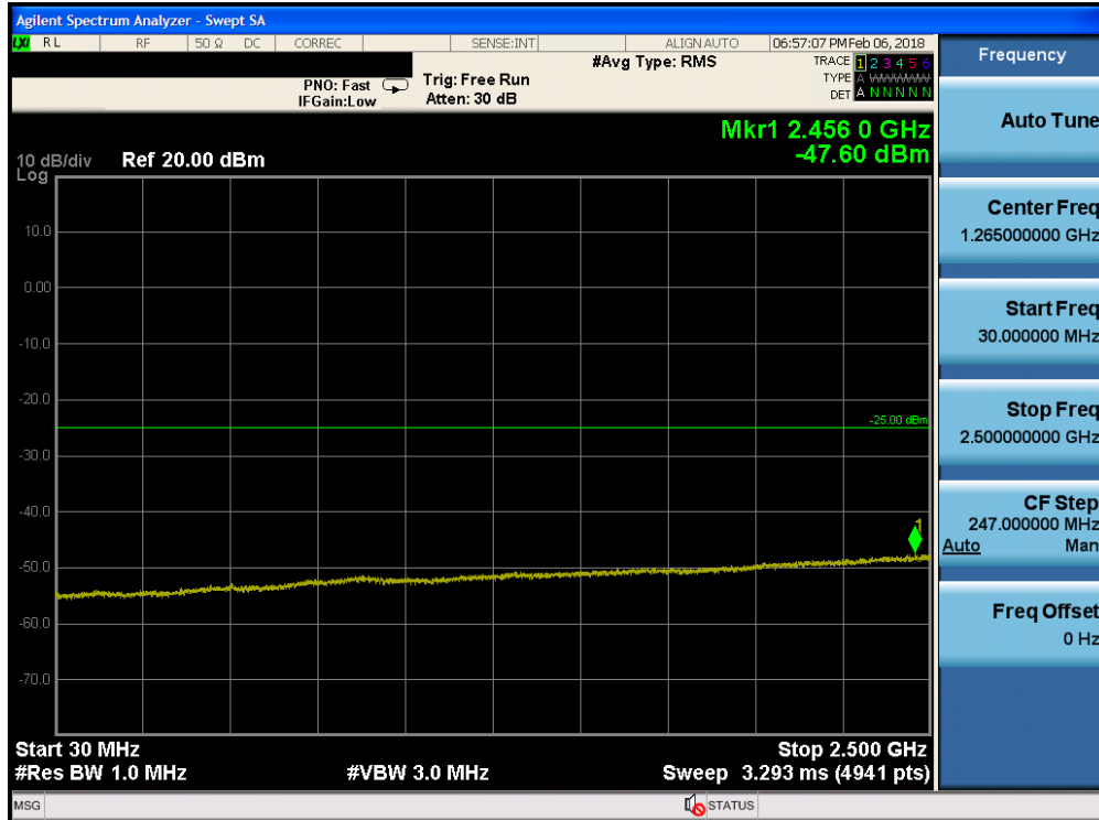
Plot 7-91. Conducted Spurious Plot (Band 7 - 10.0MHz QPSK - RB Size 1, RB Offset 0 - High Channel)
