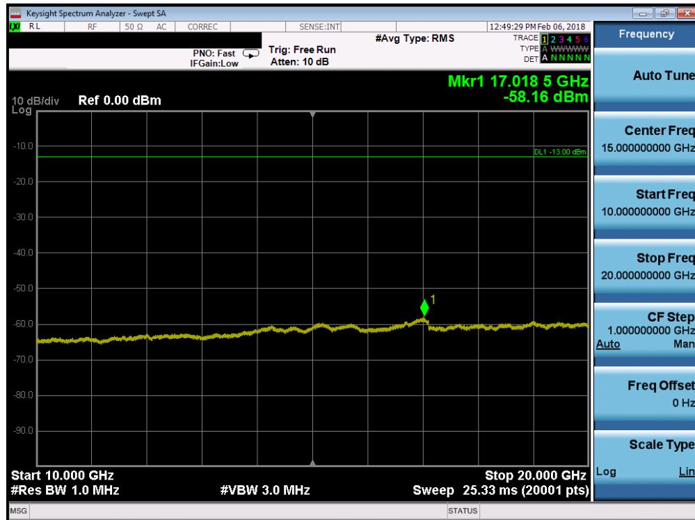
Plot 7-75. Conducted Spurious Plot (Band 4 - 10.0MHz QPSK - RB Size 1, RB Offset 0 - High Channel)
