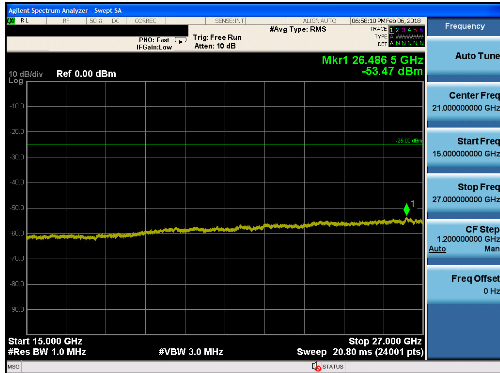
Plot 7-93. Conducted Spurious Plot (Band 7 - 10.0MHz QPSK - RB Size 1, RB Offset 0 - High Channel)
