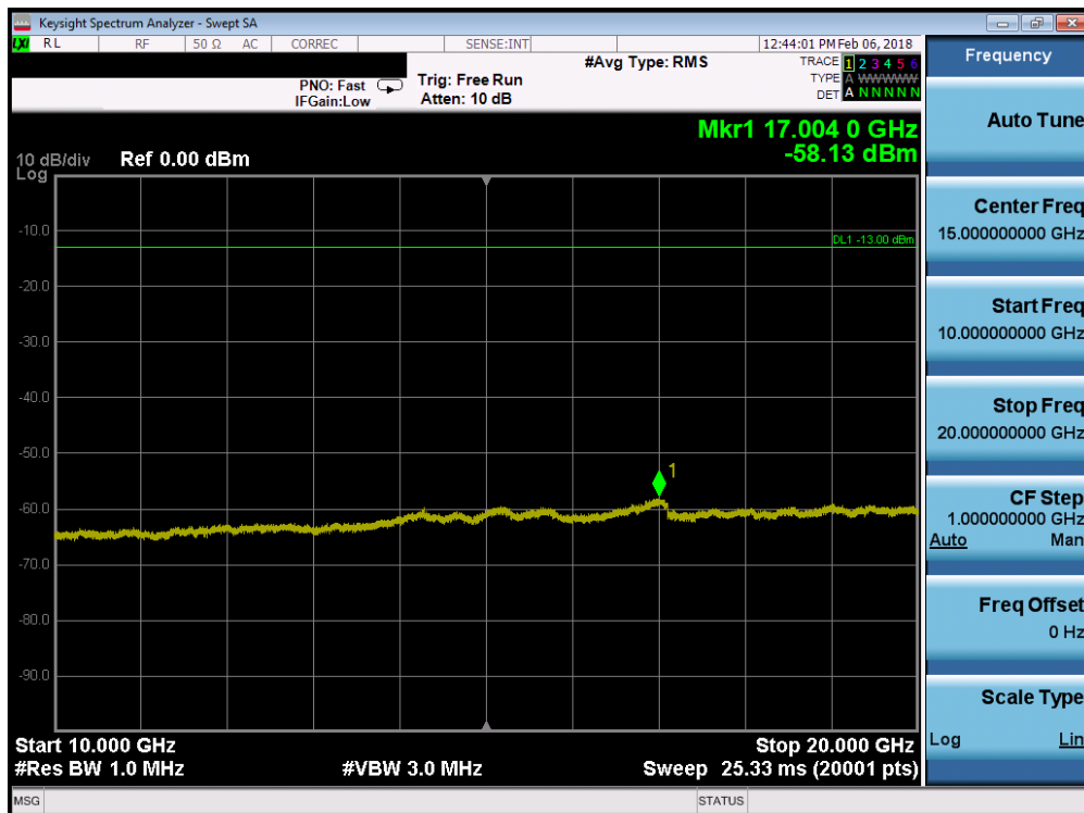
Plot 7-72. Conducted Spurious Plot (Band 4 - 10.0MHz QPSK - RB Size 1, RB Offset 0 - Mid Channel)
