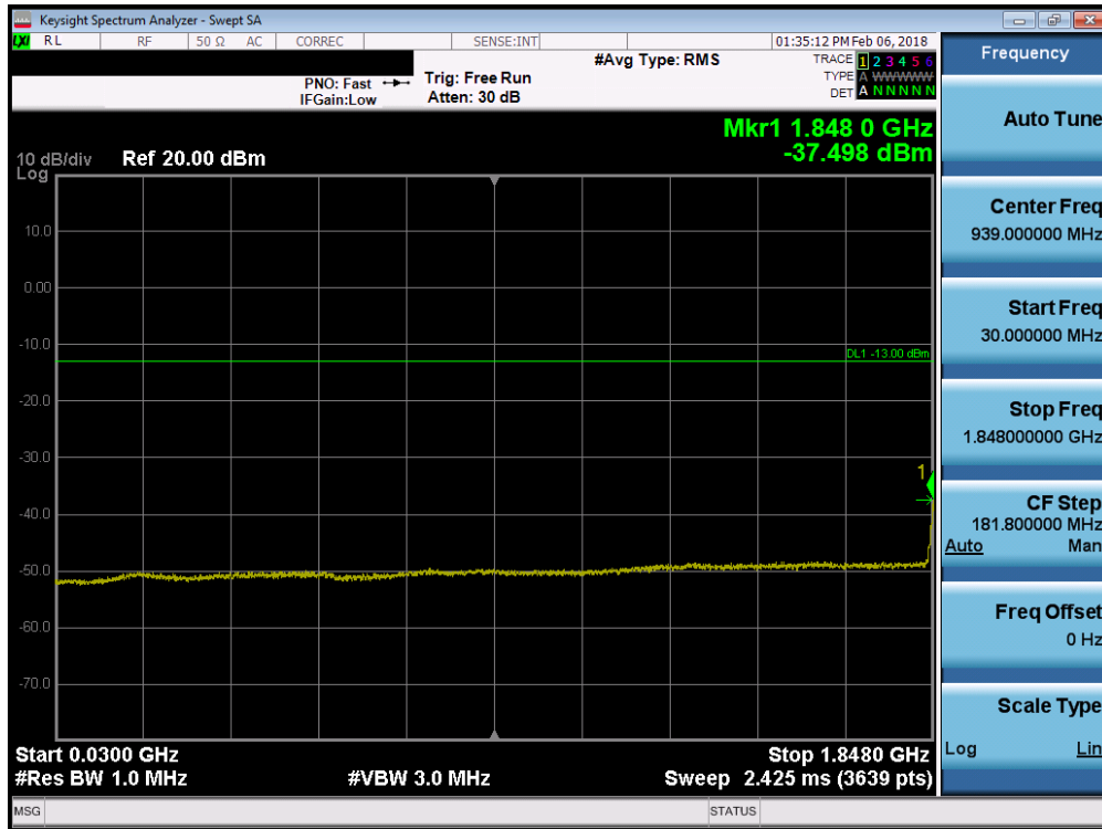
Plot 7-76. Conducted Spurious Plot (Band 2 - 5.0MHz QPSK - RB Size 1, RB Offset 0 - Low Channel)
