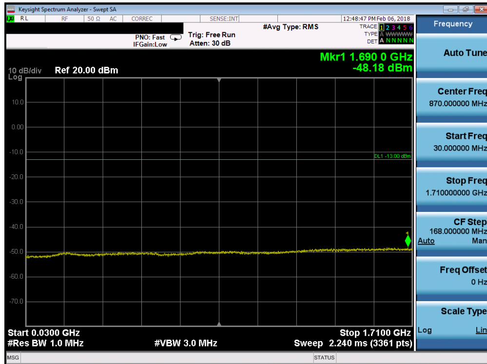
Plot 7-73. Conducted Spurious Plot (Band 4 - 10.0MHz QPSK - RB Size 1, RB Offset 0 - High Channel)
