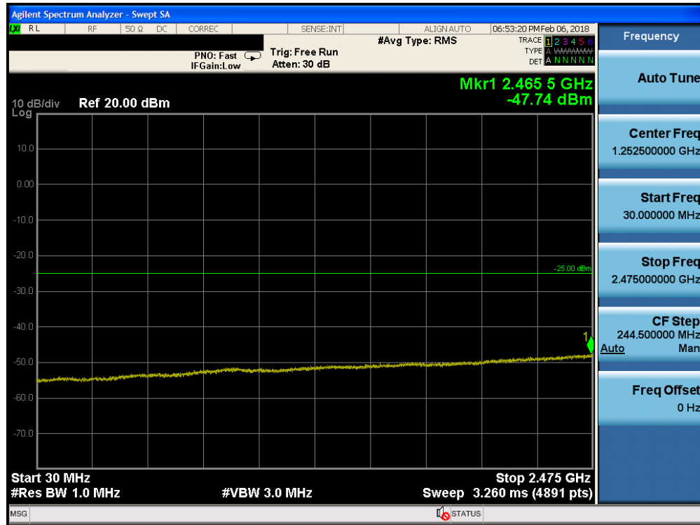
Plot 7-85. Conducted Spurious Plot (Band 7 - 10.0MHz QPSK - RB Size 1, RB Offset 0 - Low Channel)
