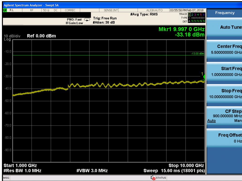
Plot 7-13. Conducted Spurious Plot (LTE B14 – 5.0MHz QPSK – RB Size 1, RB Offset 0 – High Channel)
