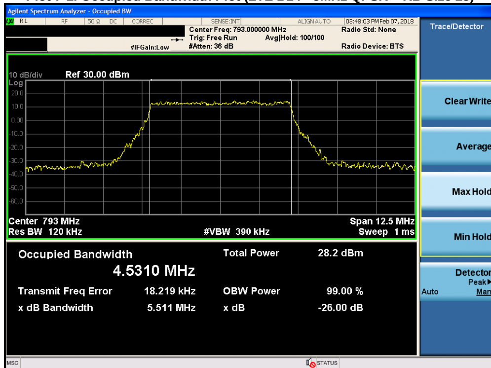
Plot 7-2. Occupied Bandwidth Plot (LTE B14 - 5MHz 16-QAM – RB Size 25)
