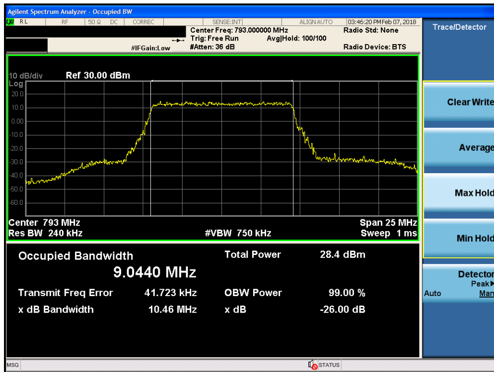
Plot 7-4. Occupied Bandwidth Plot (LTE B14 - 10MHz 16-QAM – RB Size 50)
