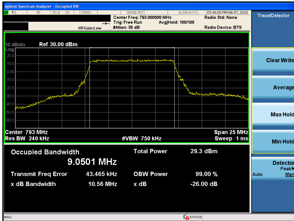
Plot 7-3. Occupied Bandwidth Plot (LTE B14 - 10MHz QPSK – RB Size 50)
