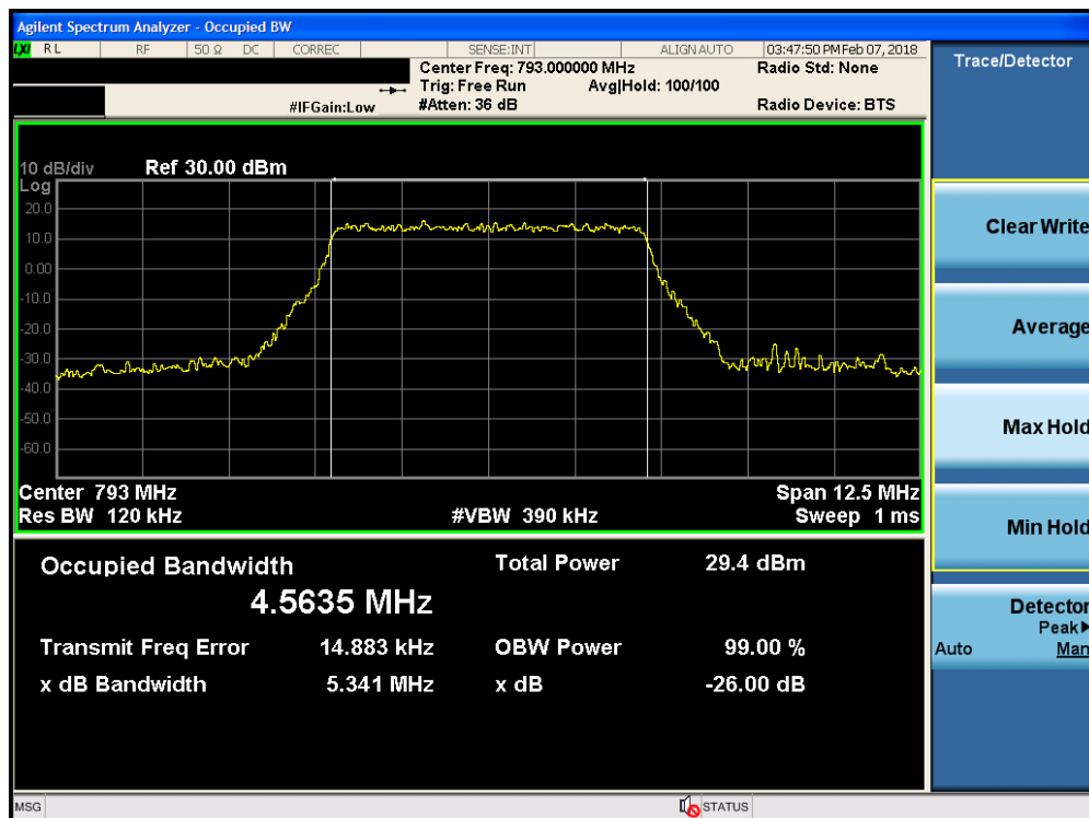
Plot 7-1. Occupied Bandwidth Plot (LTE B14 - 5MHz QPSK – RB Size 25)
