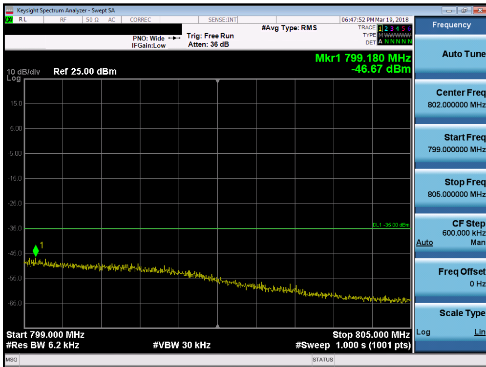
Plot 7-17. Upper Emission Mask Band Edge Plot (LTE B14 - 5MHz QPSK – RB Size 25)
