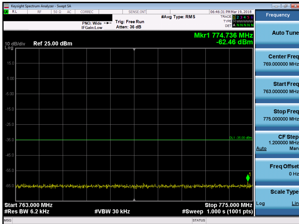
Plot 7-15. Lower Emission Mask Band Edge Plot (LTE B14 - 5MHz QPSK – RB Size 25)
