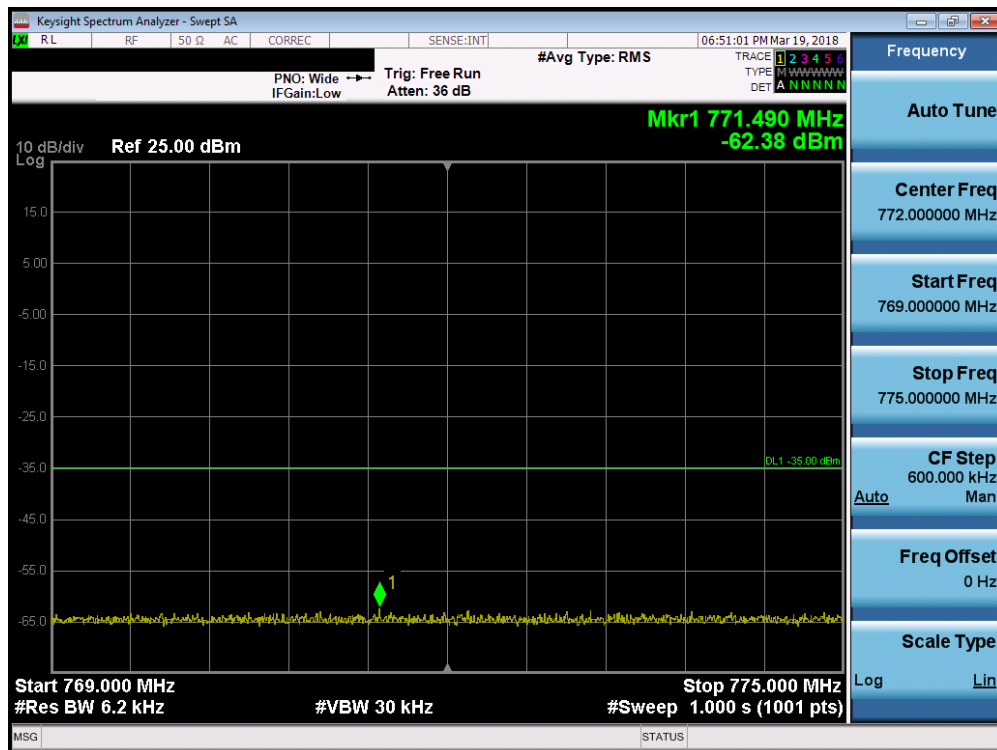
Plot 7-19. Lower Emission Mask Band Edge Plot (LTE B14 - 10MHz QPSK – RB Size 50)
