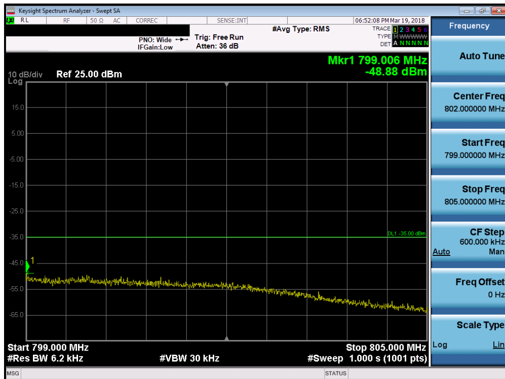
Plot 7-21. Upper Emission Mask Band Edge Plot (LTE B14 - 10MHz QPSK – RB Size 50)
