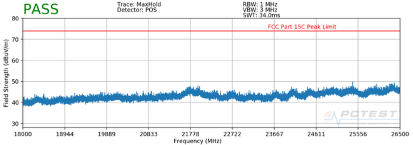
Plot 7-48. Radiated Spurious Plot above 18GHz (Ant. Pol. H)
