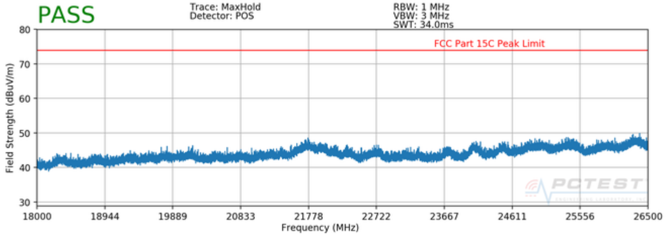
Plot 7-49. Radiated Spurious Plot above 18GHz (Ant. Pol. V)
