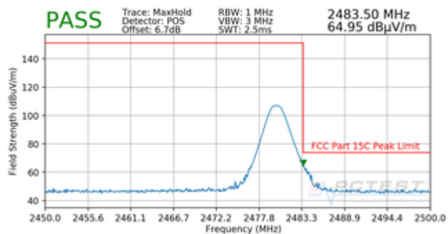
Plot 7-51. Radiated Restricted Upper Band Edge Measurement (Peak)
