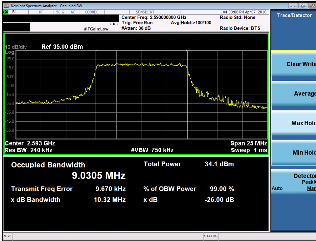
Plot 7-45. Occupied Bandwidth Plot (Band 41 - 10.0MHz QPSK - Full RB Configuration)
