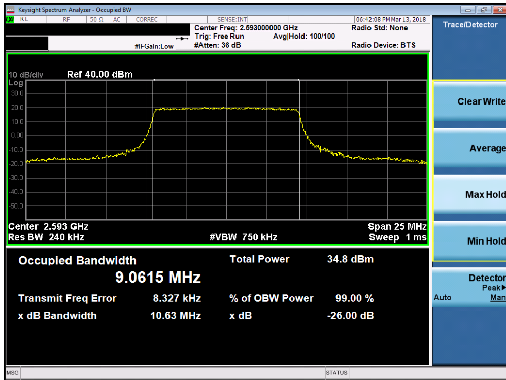
Plot 7-53. Occupied Bandwidth Plot (Band 41 - 10.0MHz QPSK - Full RB Configuration)
