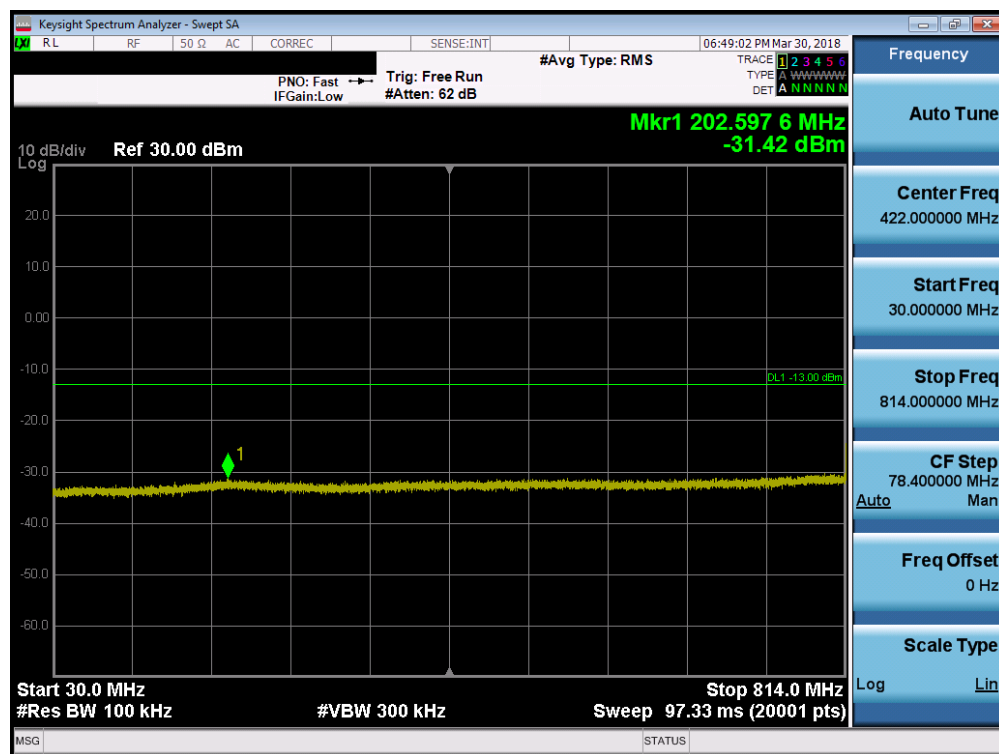
Plot 7-18. Conducted Spurious Plot ( LTE B26 - 15MHz QPSK – RB Size 1, RB Offset 0 – Mid Channel)
