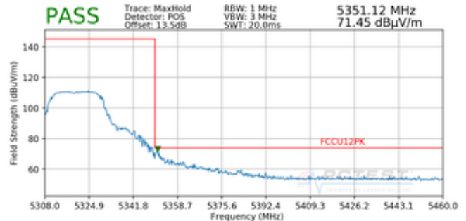
Plot 7-77. Radiated Upper Band Edge Plot (Peak – UNII Band 2A)
