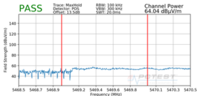
Plot 7-86. Radiated Lower Band Edge Plot (Peak – UNII Band 2C)
