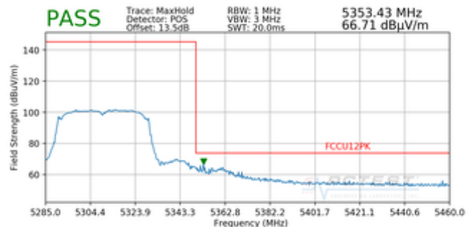
Plot 7-84. Radiated Upper Band Edge Plot (Peak – UNII Band 2A)
