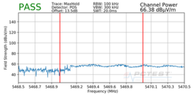
Plot 7-79. Radiated Lower Band Edge Plot (Peak – UNII Band 2C)
