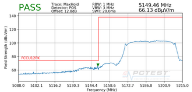
Plot 7-82. Radiated Lower Band Edge Plot (Peak – UNII Band 1)
