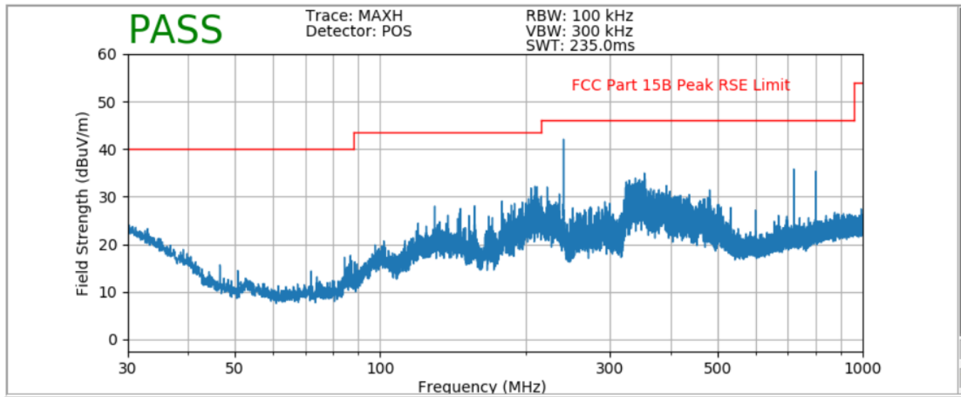
Plot 7-1. Radiated Spurious Plot below 1GHz
