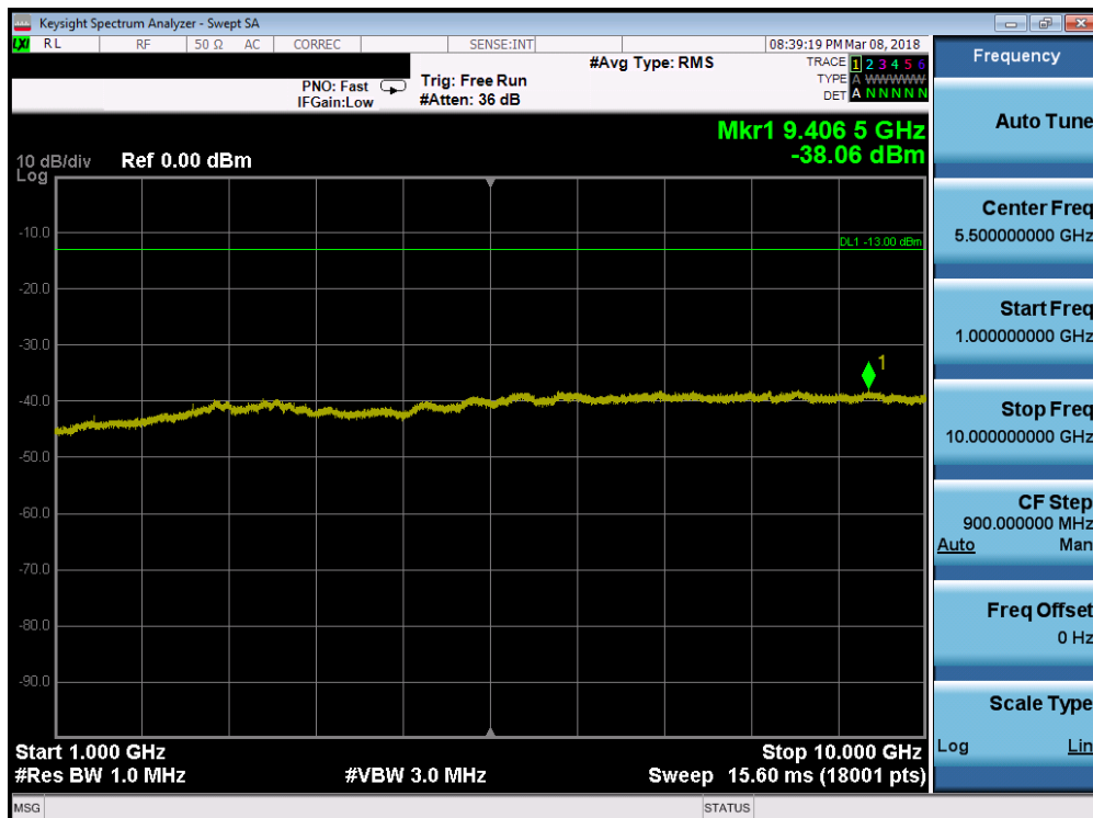
Plot 7-71. Conducted Spurious Plot (Band 12 - 10.0MHz QPSK - RB Size 1, RB Offset 0 - Mid Channel)
