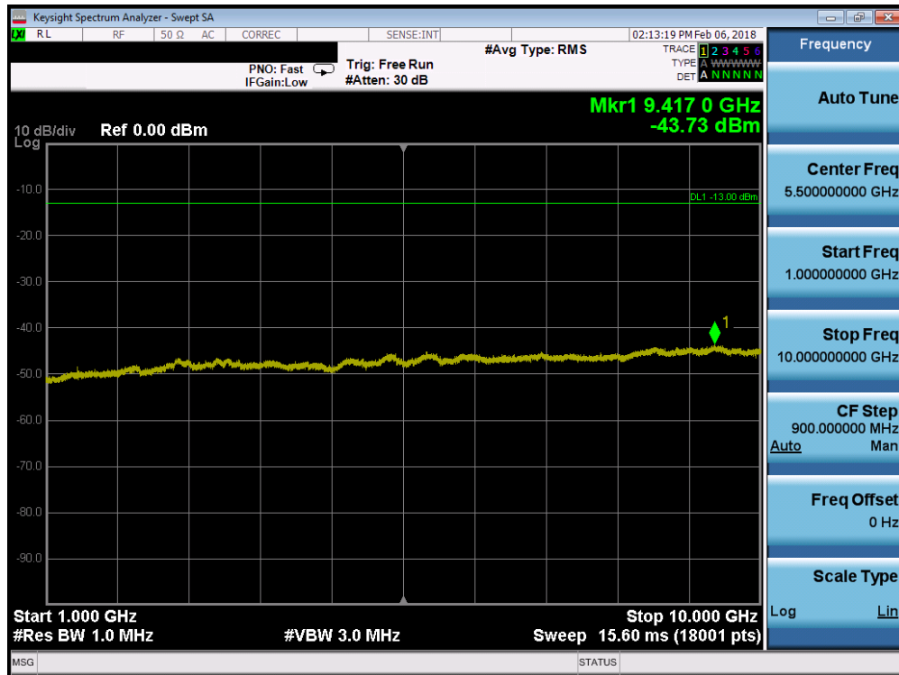
Plot 7-68. Conducted Spurious Plot (Band 12 - 10.0MHz QPSK - RB Size 1, RB Offset 0 - Low Channel)
