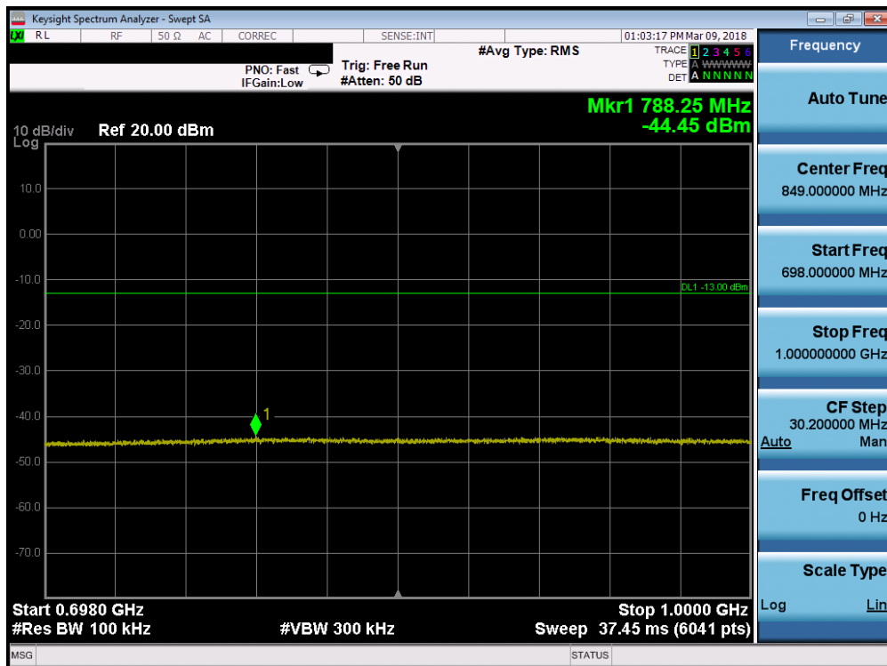
Plot 7-58. Conducted Spurious Plot (Band 71 - 5.0MHz QPSK - RB Size 1, RB Offset 0 - Low Channel)
