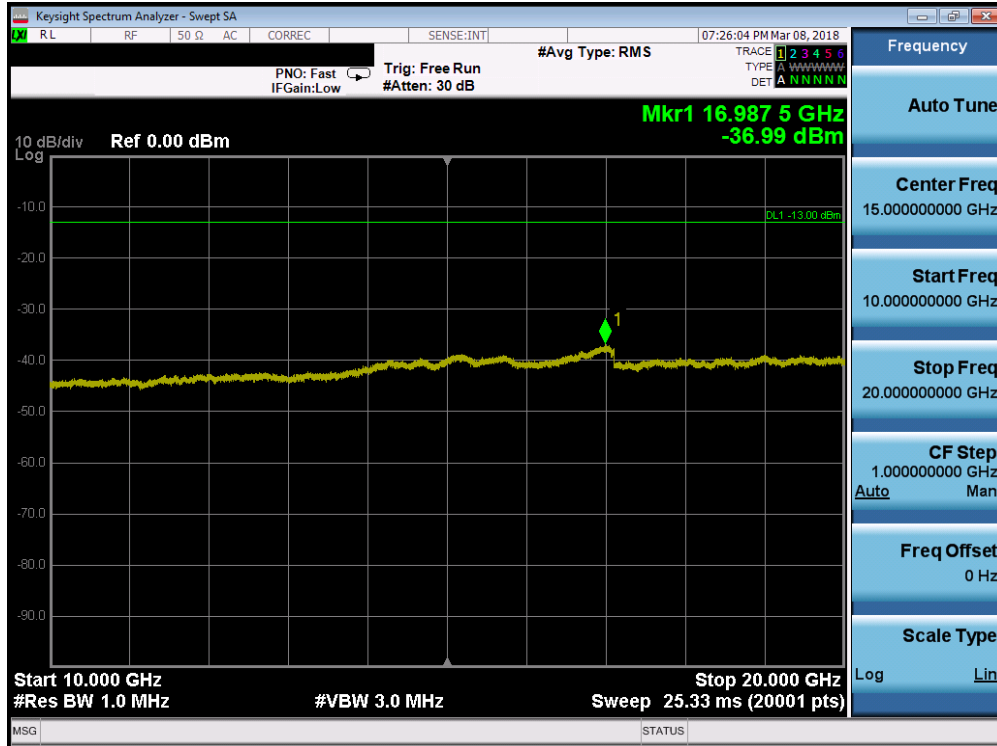
Plot 7-101. Conducted Spurious Plot (Band 2 - 10.0MHz QPSK - RB Size 1, RB Offset 0 - High Channel)
