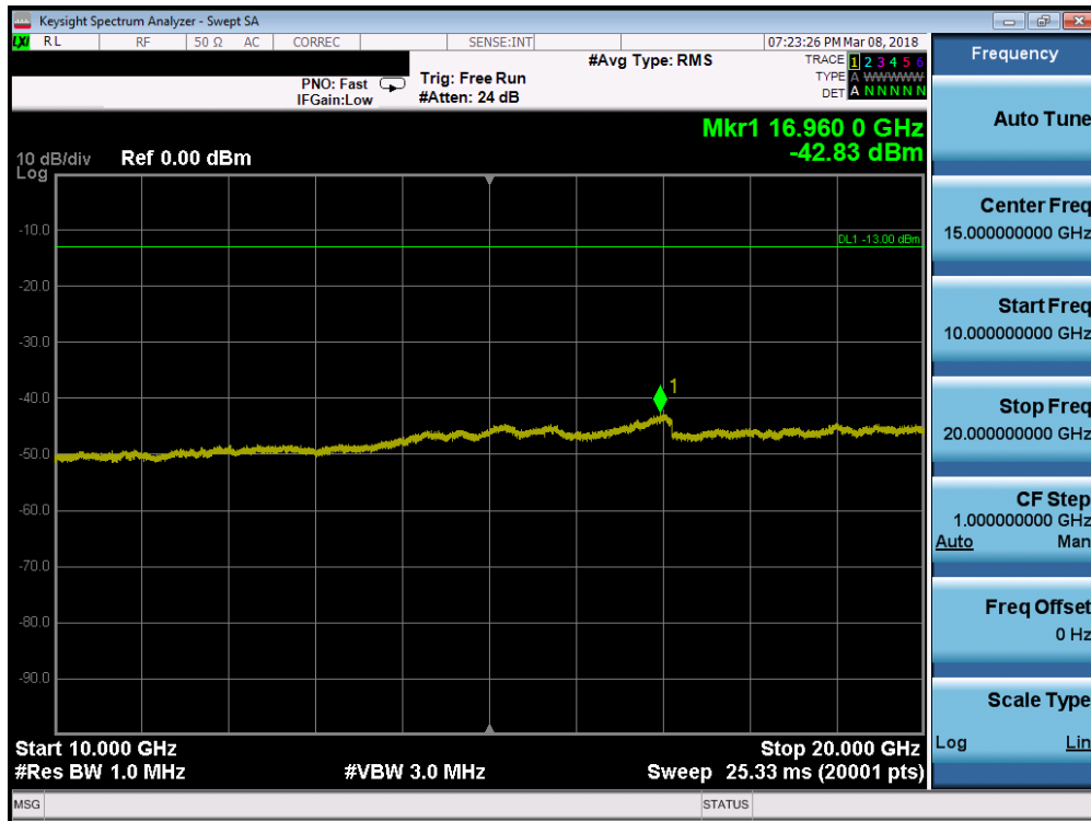
Plot 7-95. Conducted Spurious Plot (Band 2 - 10.0MHz QPSK - RB Size 1, RB Offset 0 - Low Channel)
