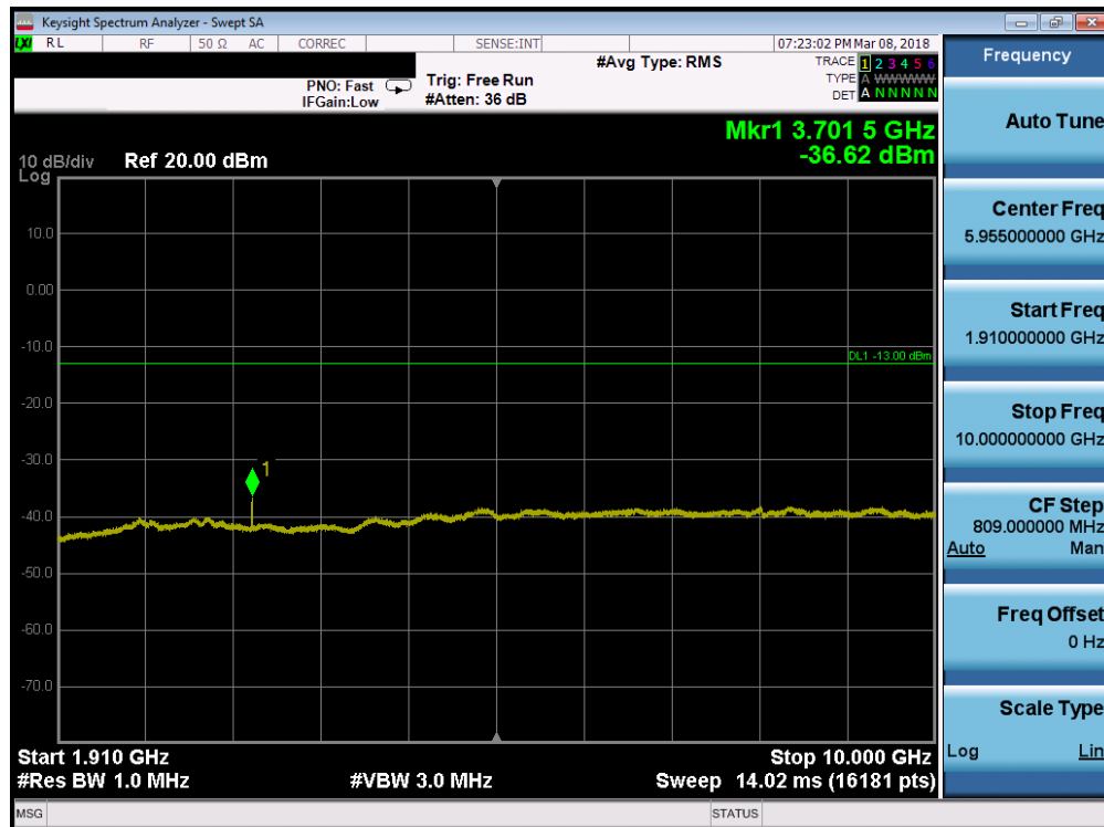
Plot 7-94. Conducted Spurious Plot (Band 2 - 10.0MHz QPSK - RB Size 1, RB Offset 0 - Low Channel)
