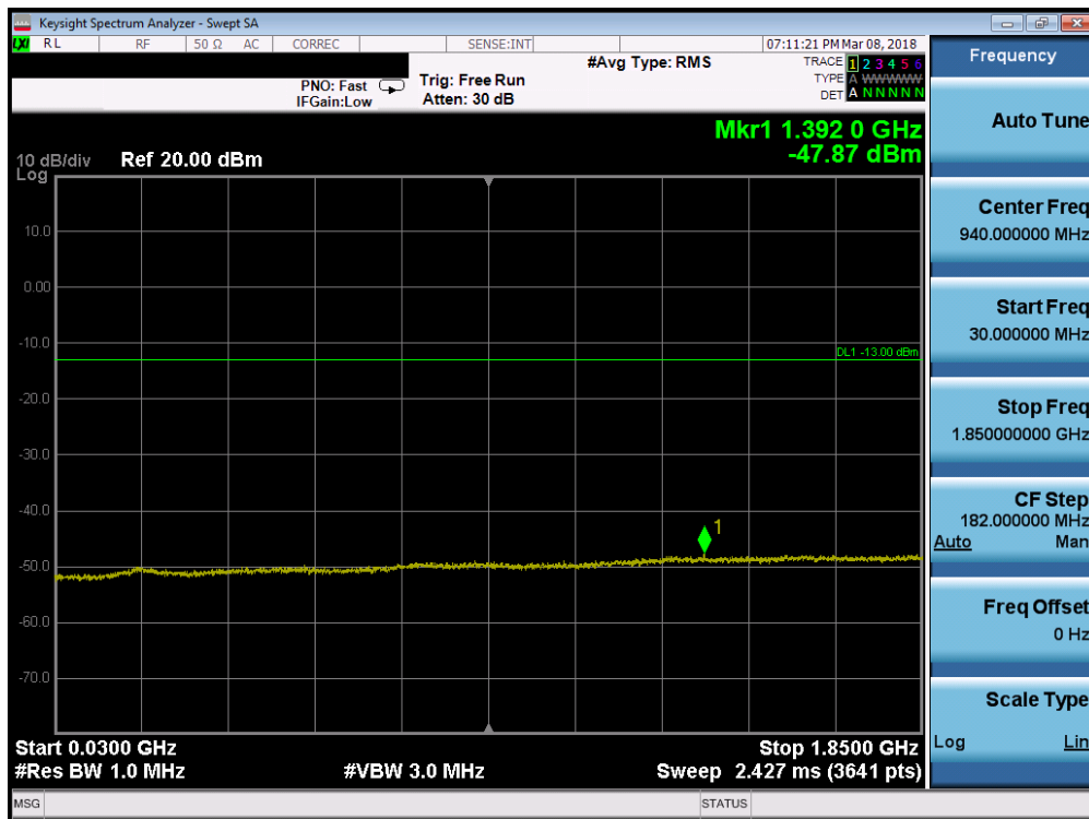
Plot 7-96. Conducted Spurious Plot (Band 2 - 10.0MHz QPSK - RB Size 1, RB Offset 0 - Mid Channel)
