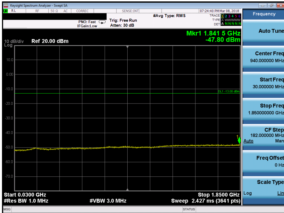
Plot 7-99. Conducted Spurious Plot (Band 2 - 10.0MHz QPSK - RB Size 1, RB Offset 0 - High Channel)
