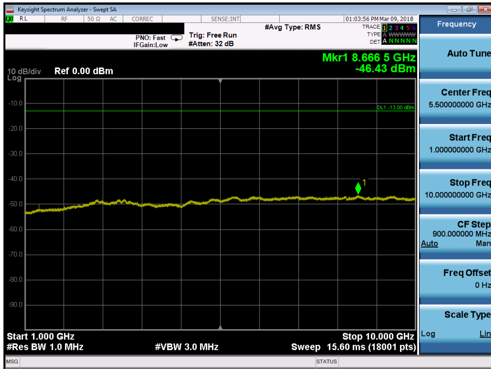
Plot 7-59. Conducted Spurious Plot (Band 71 - 5.0MHz QPSK - RB Size 1, RB Offset 0 - Low Channel)
