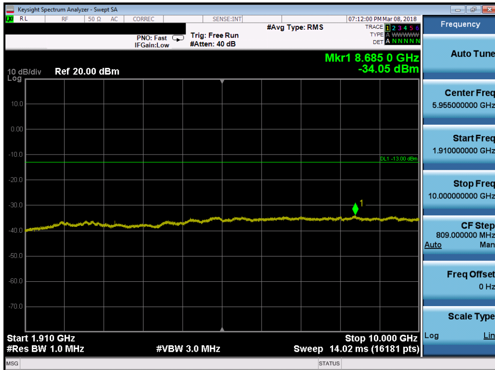
Plot 7-97. Conducted Spurious Plot (Band 2 - 10.0MHz QPSK - RB Size 1, RB Offset 0 - Mid Channel)
