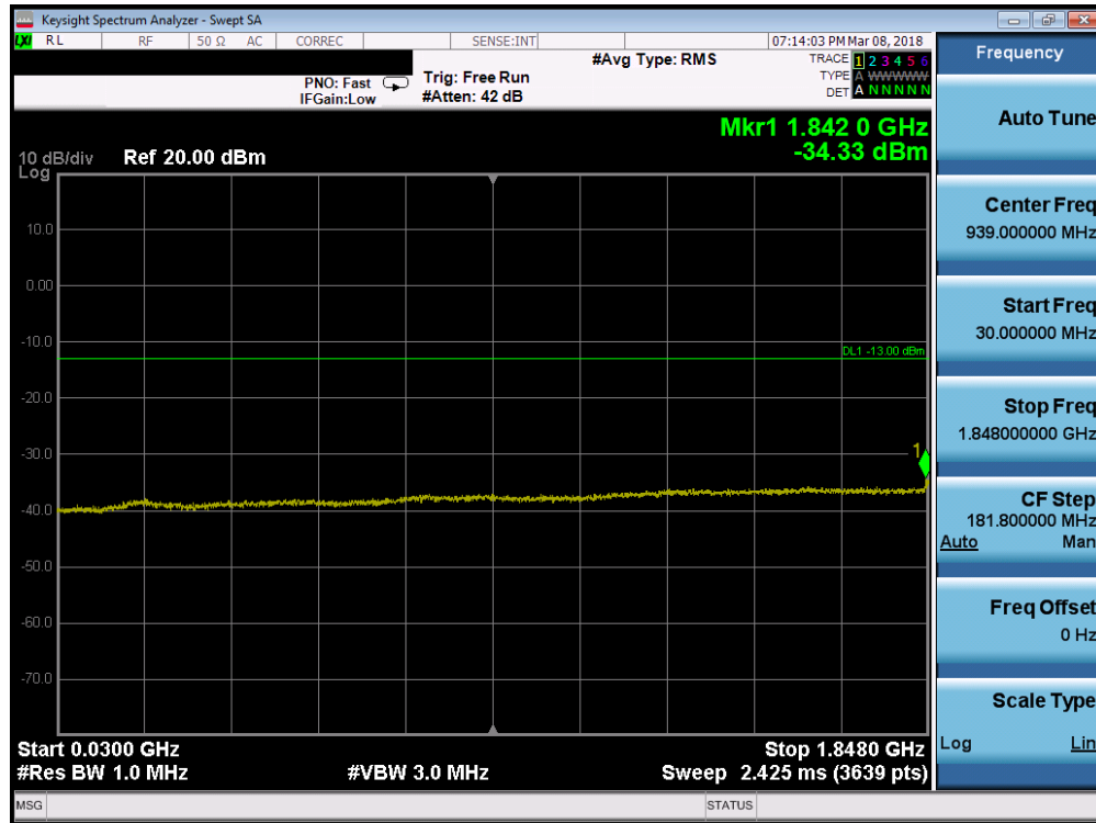
Plot 7-93. Conducted Spurious Plot (Band 2 - 10.0MHz QPSK - RB Size 1, RB Offset 0 - Low Channel)
