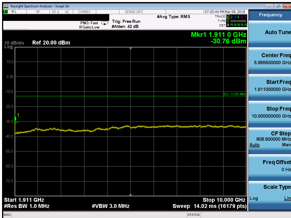
Plot 7-100. Conducted Spurious Plot (Band 2 - 10.0MHz QPSK - RB Size 1, RB Offset 0 - High Channel)
