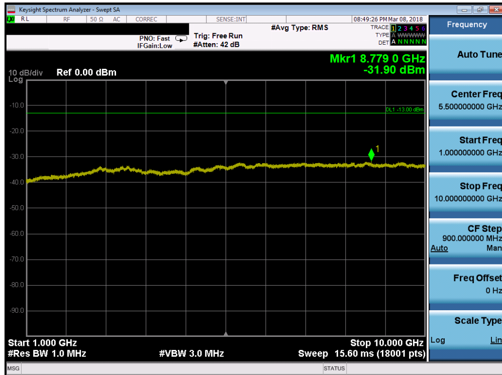
Plot 7-74. Conducted Spurious Plot (Band 12 - 10.0MHz QPSK - RB Size 1, RB Offset 0 - High Channel)
