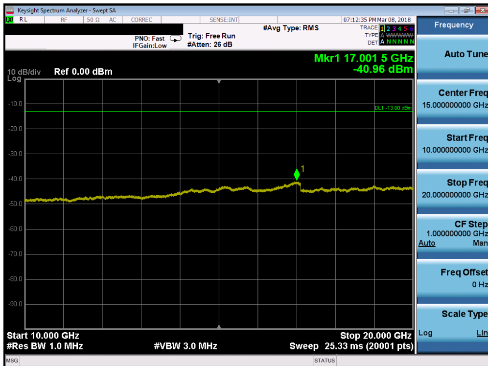
Plot 7-98. Conducted Spurious Plot (Band 2 - 10.0MHz QPSK - RB Size 1, RB Offset 0 - Mid Channel)
