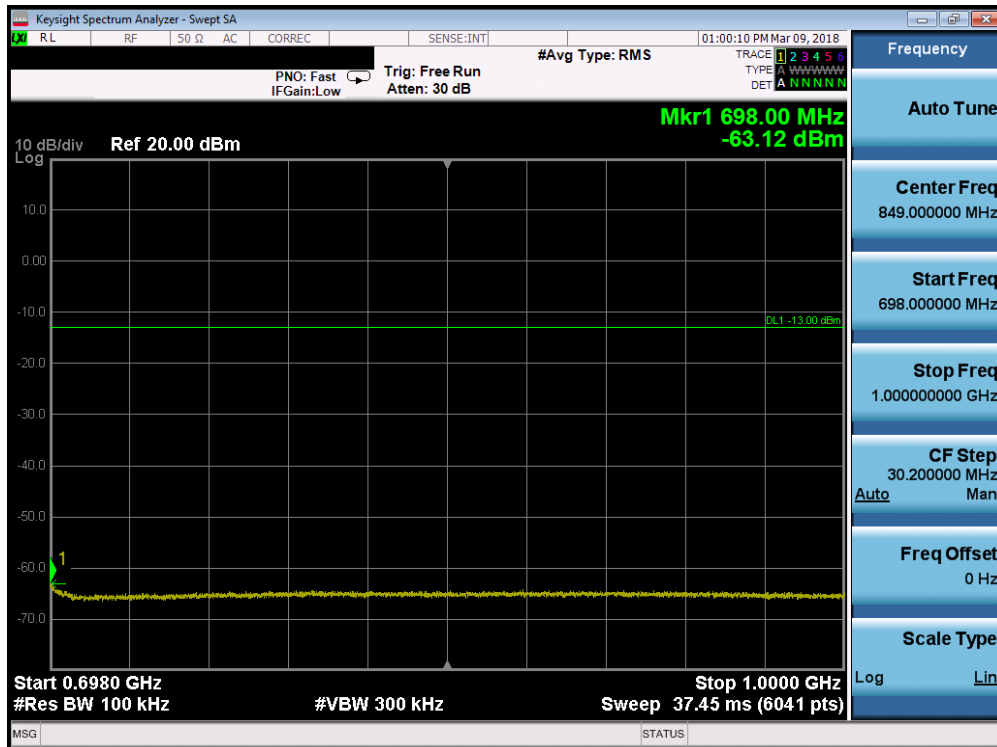
Plot 7-61. Conducted Spurious Plot (Band 71 - 5.0MHz QPSK - RB Size 1, RB Offset 0 - Mid Channel)
