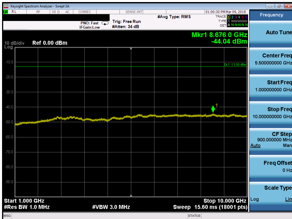
Plot 7-62. Conducted Spurious Plot (Band 71 - 5.0MHz QPSK - RB Size 1, RB Offset 0 - Mid Channel)
