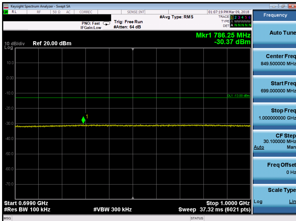
Plot 7-64. Conducted Spurious Plot (Band 71 - 5.0MHz QPSK - RB Size 1, RB Offset 0 - High Channel)
