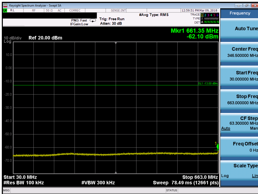
Plot 7-60. Conducted Spurious Plot (Band 71 - 5.0MHz QPSK - RB Size 1, RB Offset 0 - Mid Channel)
