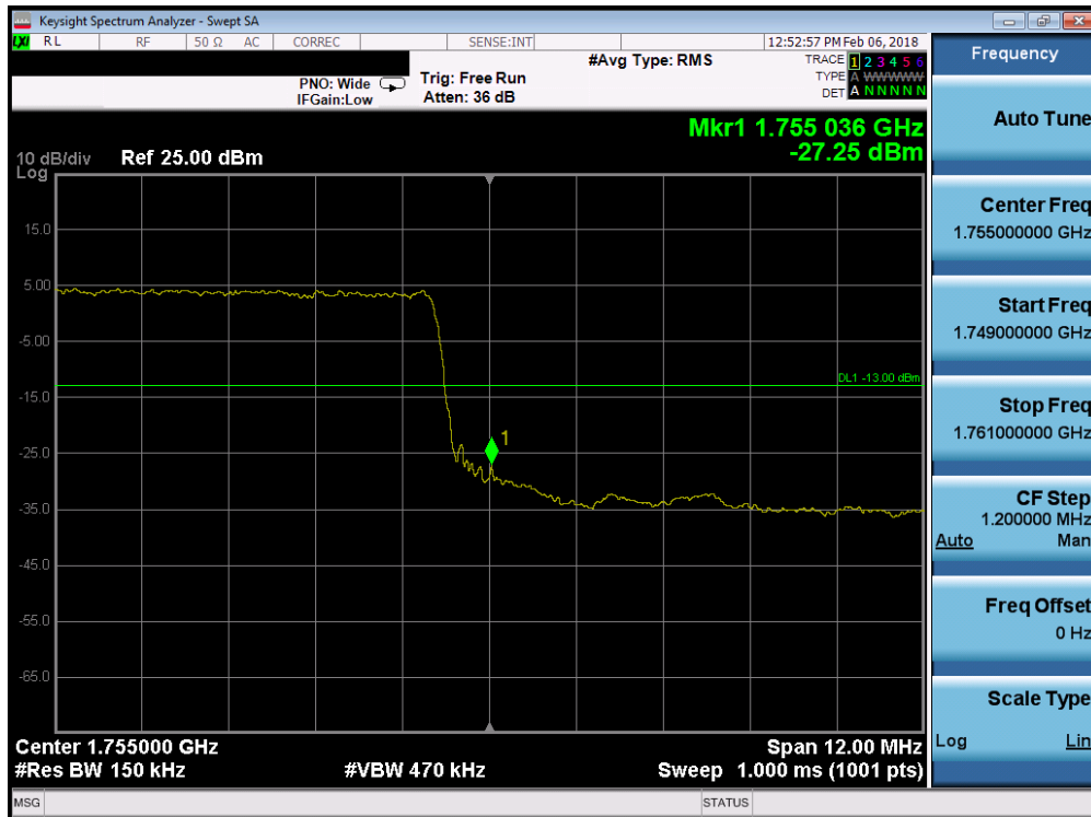
Plot 7-170. Upper Band Edge Plot (Band 4 - 15.0MHz QPSK - Full RB Configuration)
