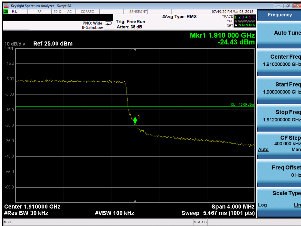
Plot 7-180. Upper Band Edge Plot (Band 2 - 3.0MHz QPSK - Full RB Configuration)
