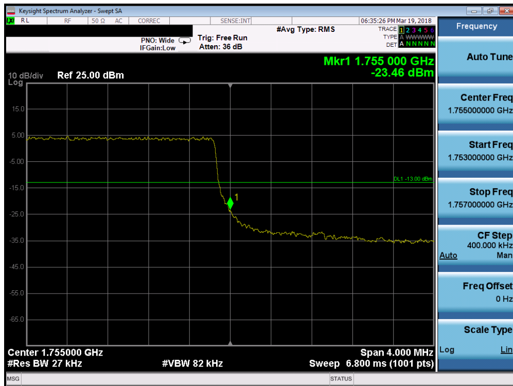
Plot 7-164. Upper Band Edge Plot (Band 4 - 3.0MHz QPSK - Full RB Configuration)
