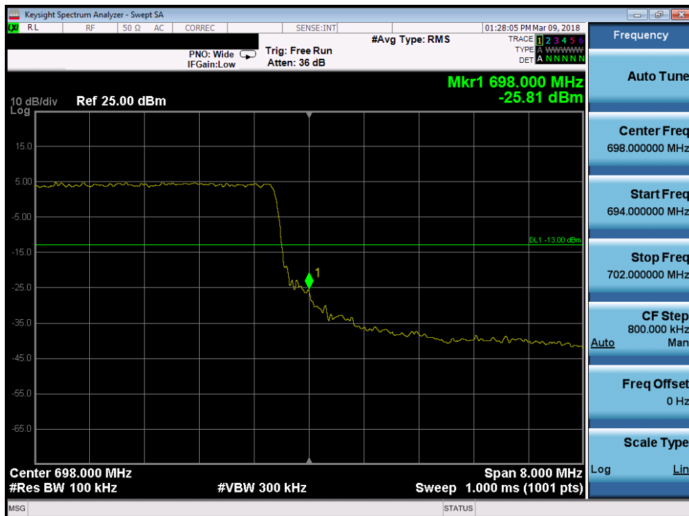
Plot 7-114. Upper Band Edge Plot (Band 71 - 10.0MHz QPSK - Full RB Configuration)
