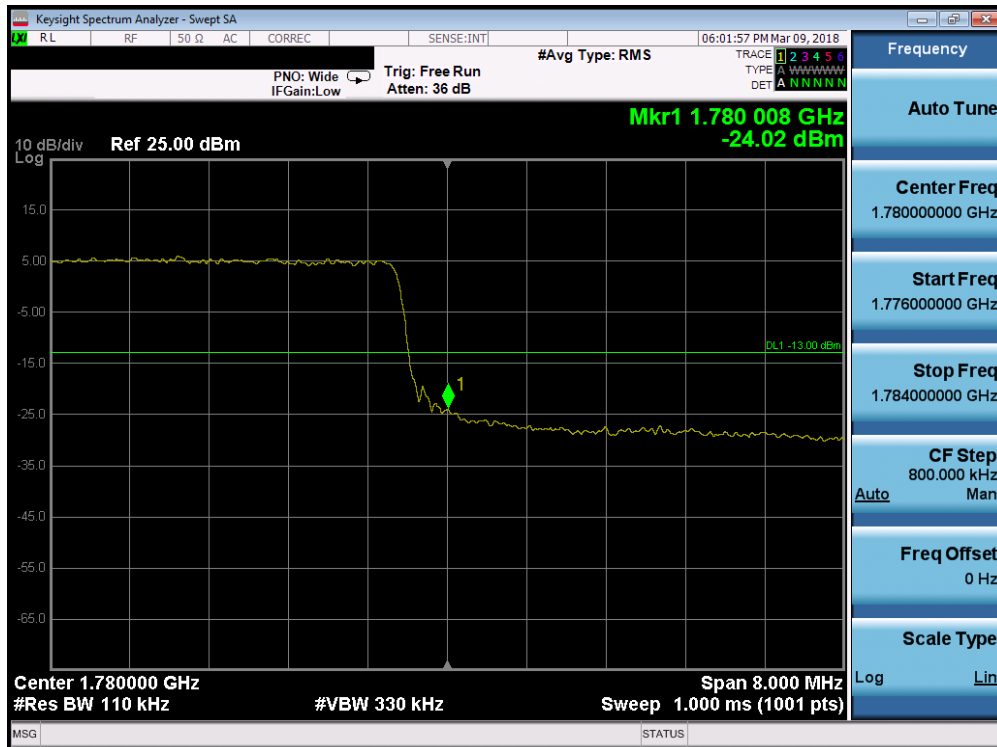
Plot 7-152. Upper Band Edge Plot (Band 66 - 10.0MHz QPSK - Full RB Configuration)
