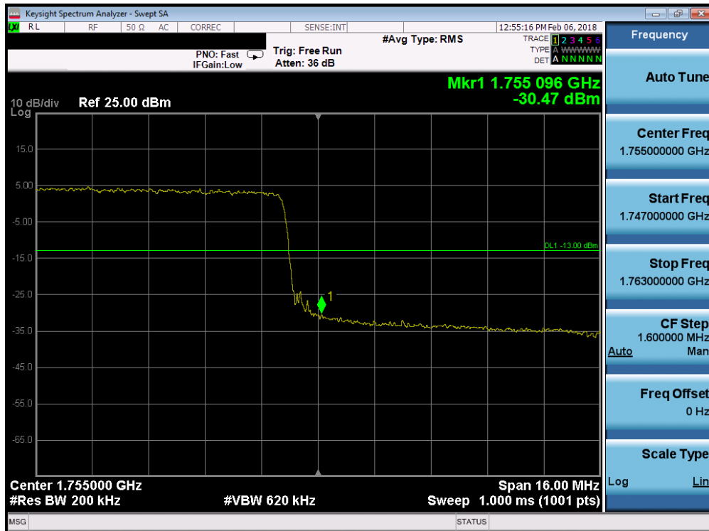
Plot 7-172. Upper Band Edge Plot (Band 4 - 20.0MHz QPSK - Full RB Configuration)
