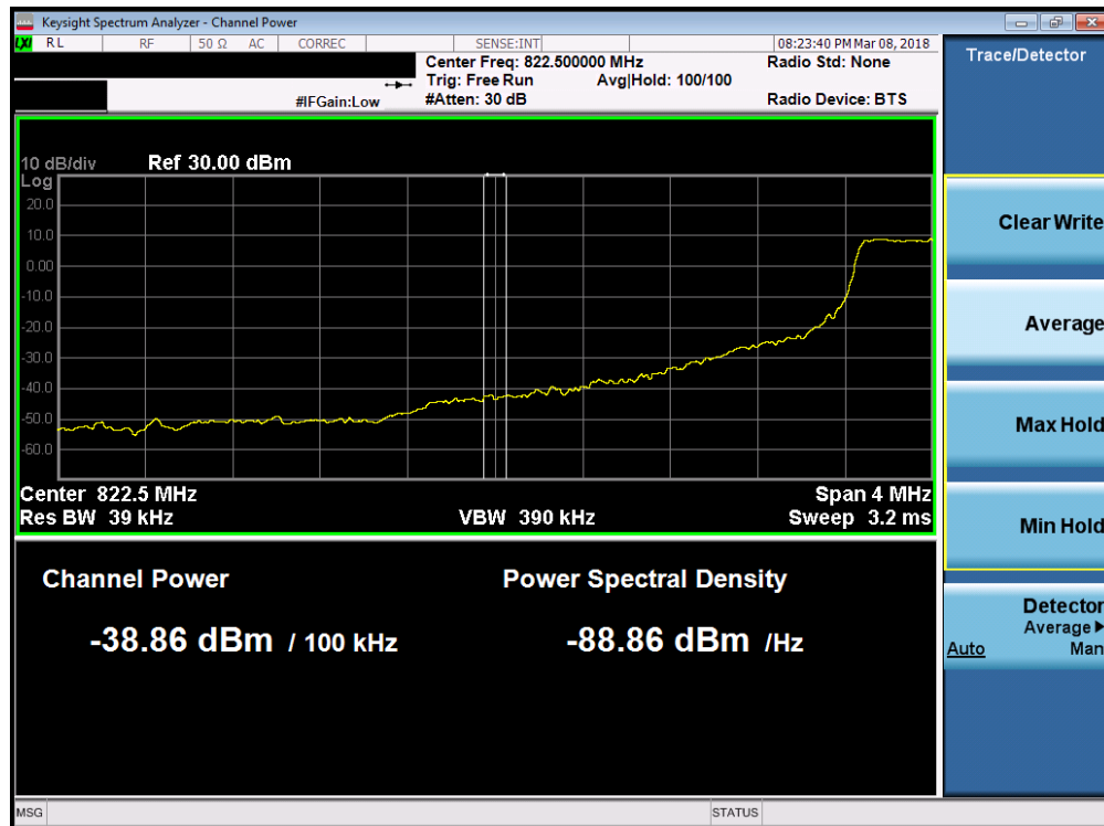
Plot 7-129. Lower Extended Band Edge Plot (Band 5 - 1.4MHz QPSK - Full RB Configuration)
