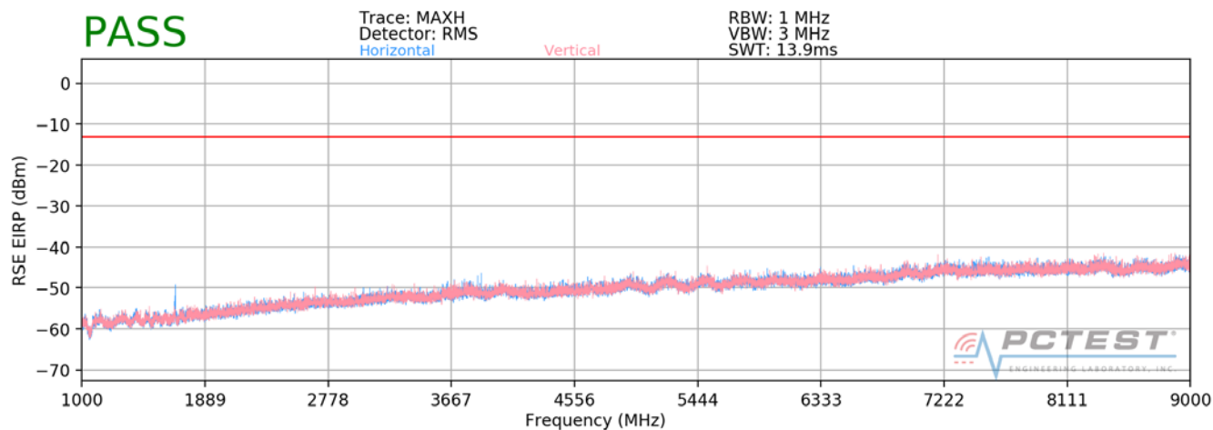
Plot 7-88. Radiated Spurious Plot above 1GHz (Cellular WCDMA)
