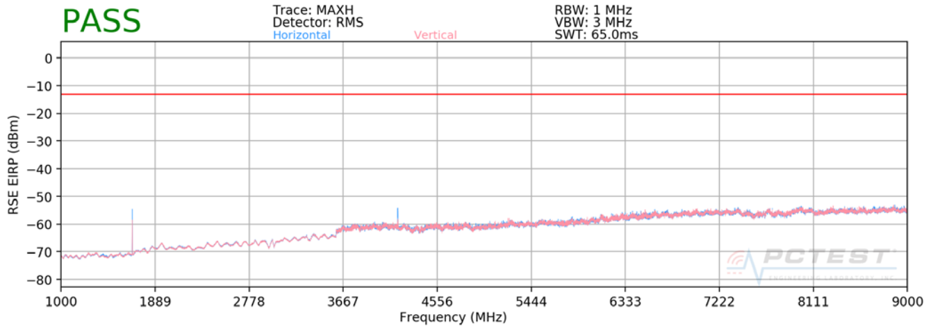
Plot 7-87. Radiated Spurious Plot above 1GHz (Cellular CDMA)
