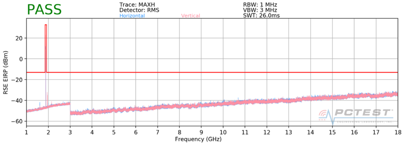
Plot 7-89. Radiated Spurious Plot above 1GHz (PCS GPRS)
