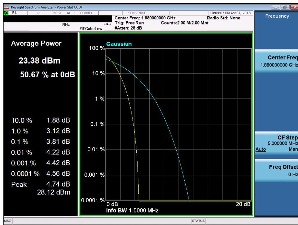
Plot 7-84. Peak-Average Ratio Plot (PCS CDMA Mode)
