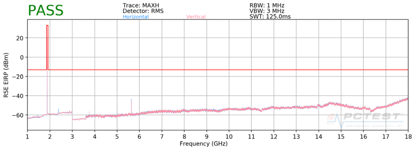
Plot 7-90. Radiated Spurious Plot above 1GHz (PCS CDMA)
