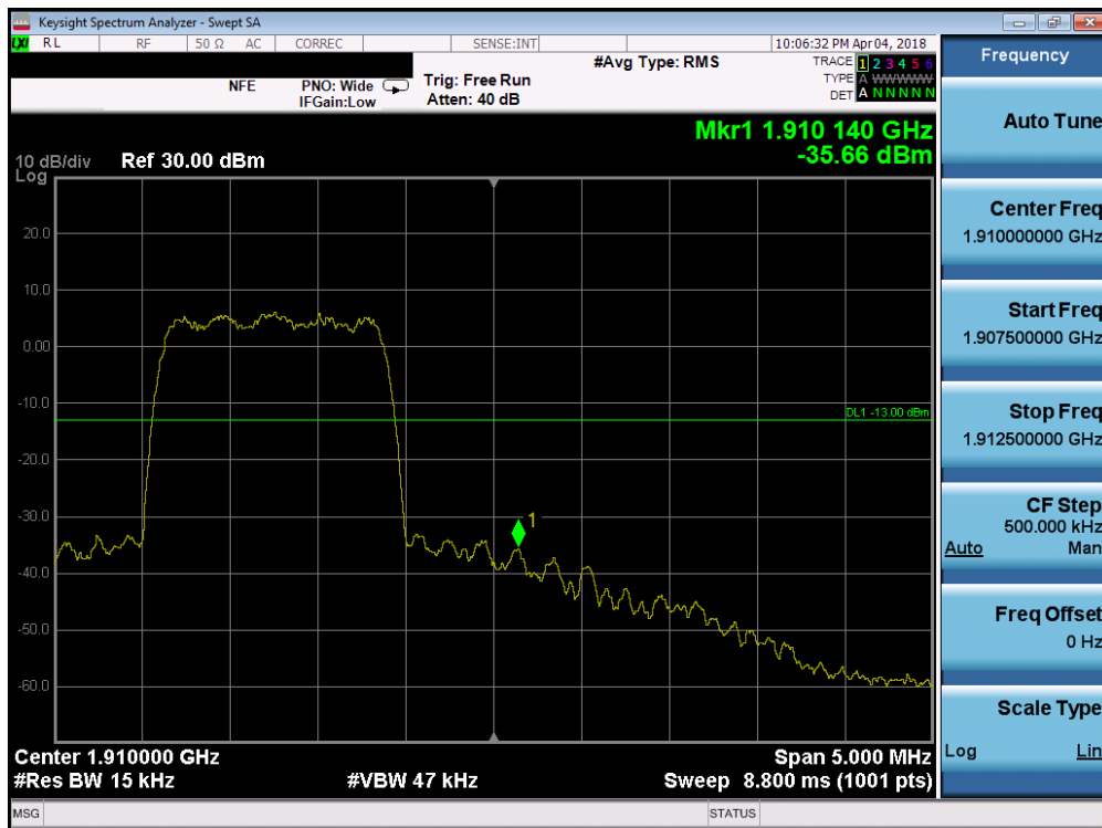
Plot 7-75. Band Edge Plot (PCS CDMA Mode - High Channel)
