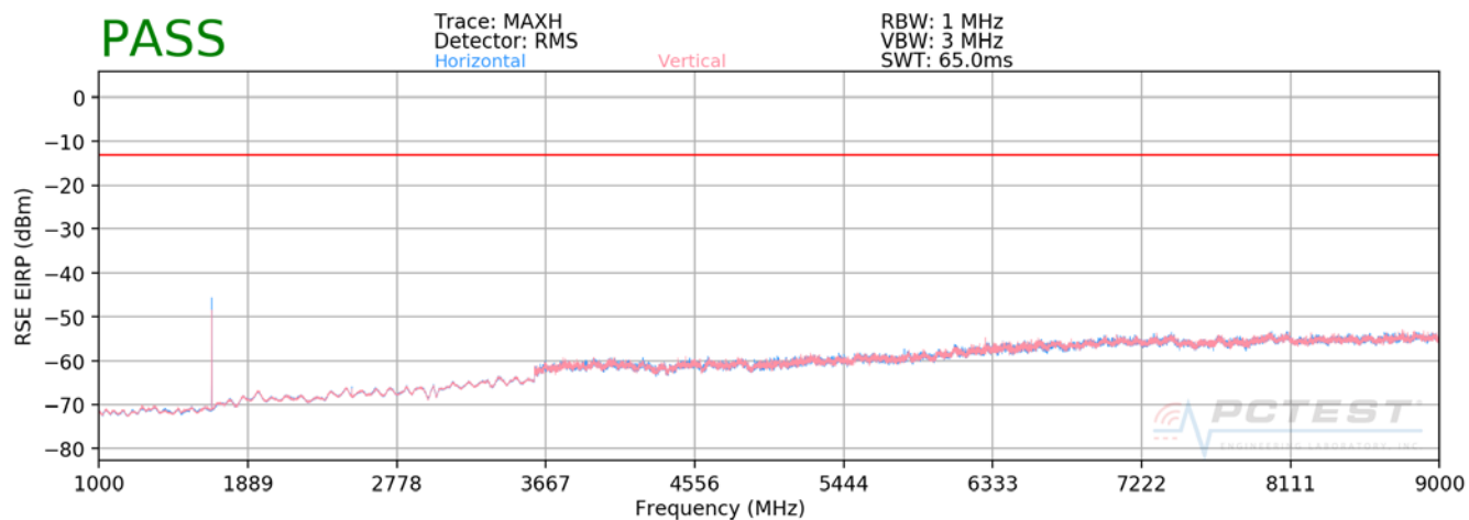
Plot 7-86. Radiated Spurious Plot above 1GHz (Cellular GPRS)
