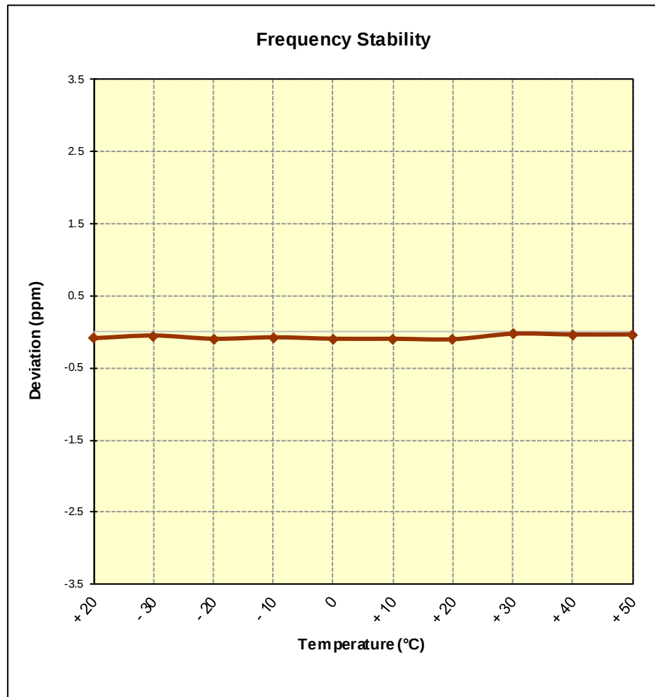
Figure 7-12. Frequency Stability Graph (PCS CDMA Mode – Ch. 600)
