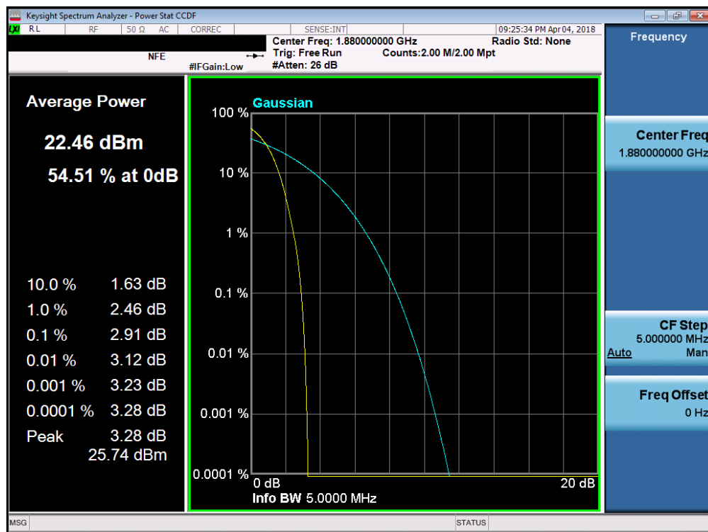
Plot 7-85. Peak-Average Ratio Plot (PCS WCDMA Mode)
