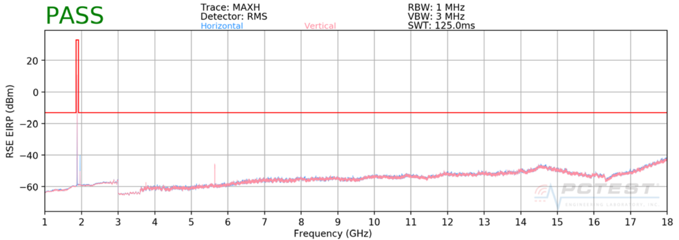
Plot 7-91. Radiated Spurious Plot above 1GHz (PCS WCDMA)
