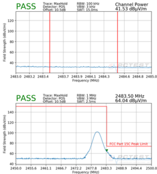
Plot 7-18. Radiated Restricted Upper Band Edge Measurement (Average & Peak)
