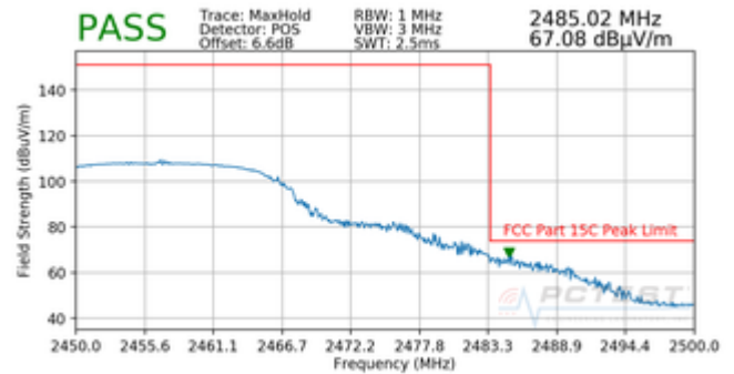
Plot 7-38. Radiated Restricted Upper Band Edge Measurement (Peak)
