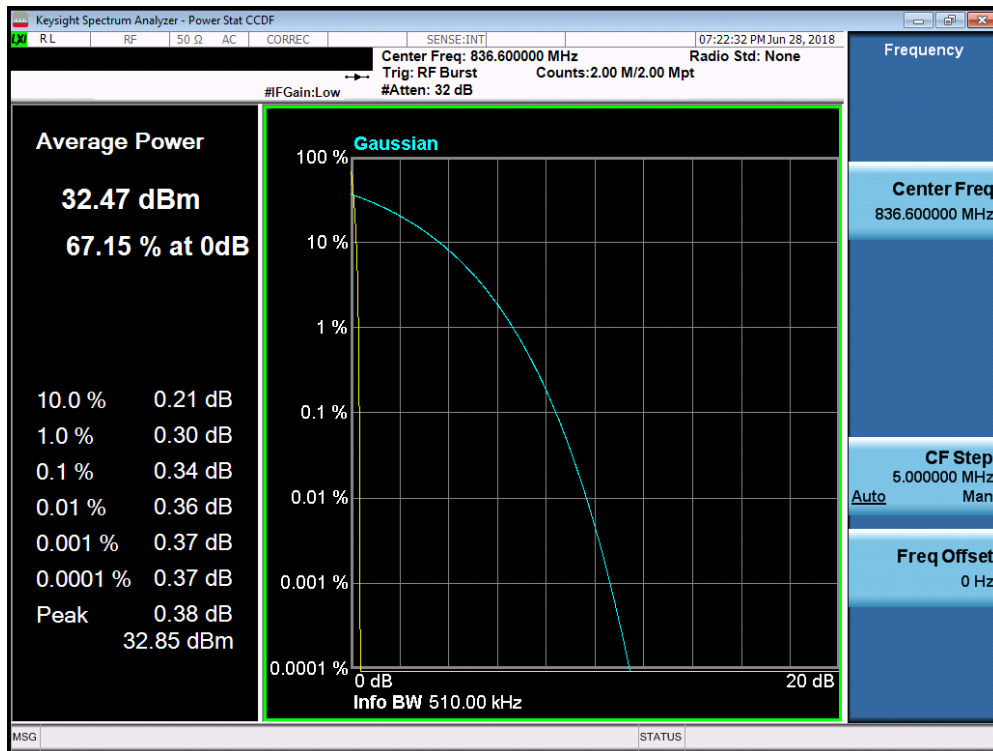
Plot 7-69. Peak-Average Ratio Plot (Cell GPRS Mode)
