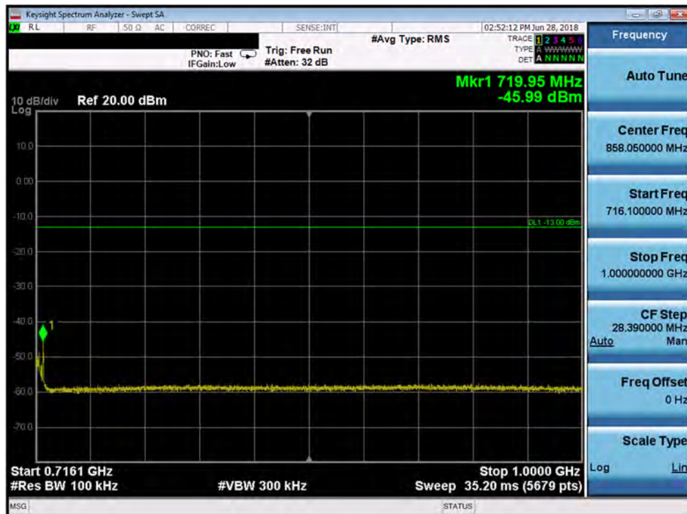
Plot 7-56. Conducted Spurious Plot (Band 12/17 - 5.0MHz QPSK - RB Size 1, RB Offset 0 - High Channel)
