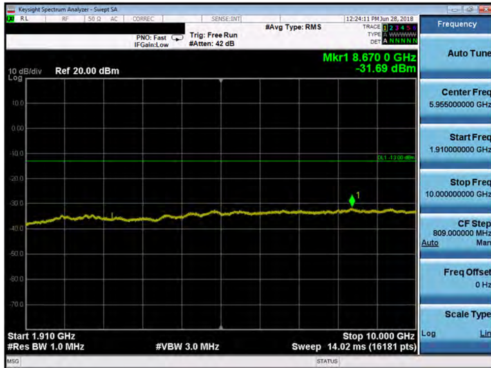
Plot 7-77. Conducted Spurious Plot (Band 2 - 1.4MHz QPSK - RB Size 1, RB Offset 0 - Low Channel)
