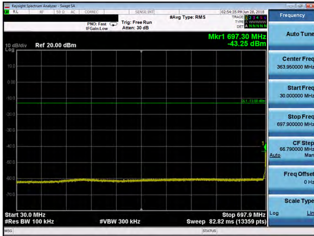
Plot 7-49. Conducted Spurious Plot (Band 12/17 - 5.0MHz QPSK - RB Size 1, RB Offset 0 - Low Channel)
