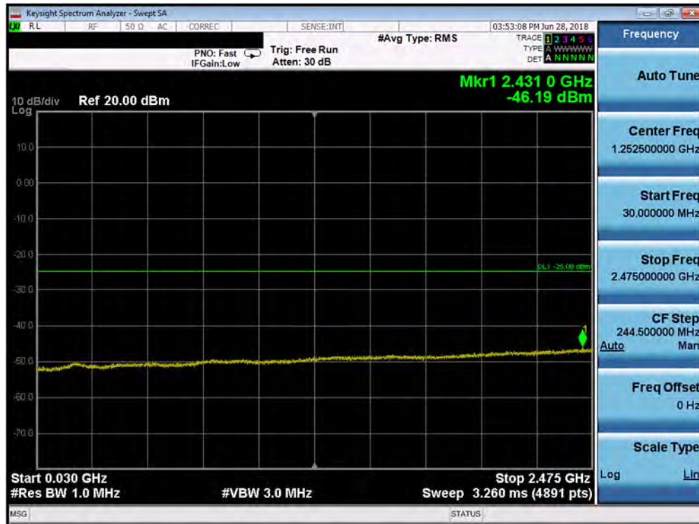
Plot 7-85. Conducted Spurious Plot (Band 7 - 5.0MHz QPSK - RB Size 1, RB Offset 0 - Low Channel)
