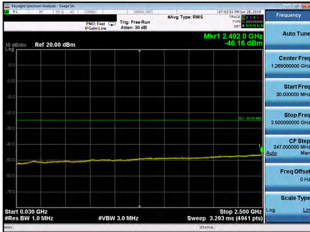
Plot 7-91. Conducted Spurious Plot (Band 7 - 5.0MHz QPSK - RB Size 1, RB Offset 0 - High Channel)
