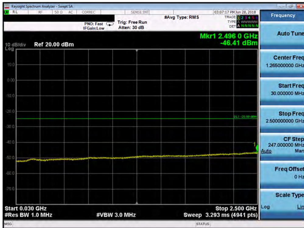
Plot 7-88. Conducted Spurious Plot (Band 7 - 5.0MHz QPSK - RB Size 1, RB Offset 0 - Mid Channel)
