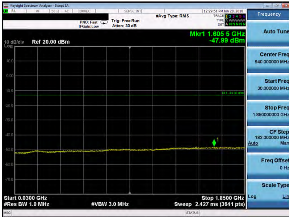
Plot 7-82. Conducted Spurious Plot (Band 2 - 1.4MHz QPSK - RB Size 1, RB Offset 0 - High Channel)
