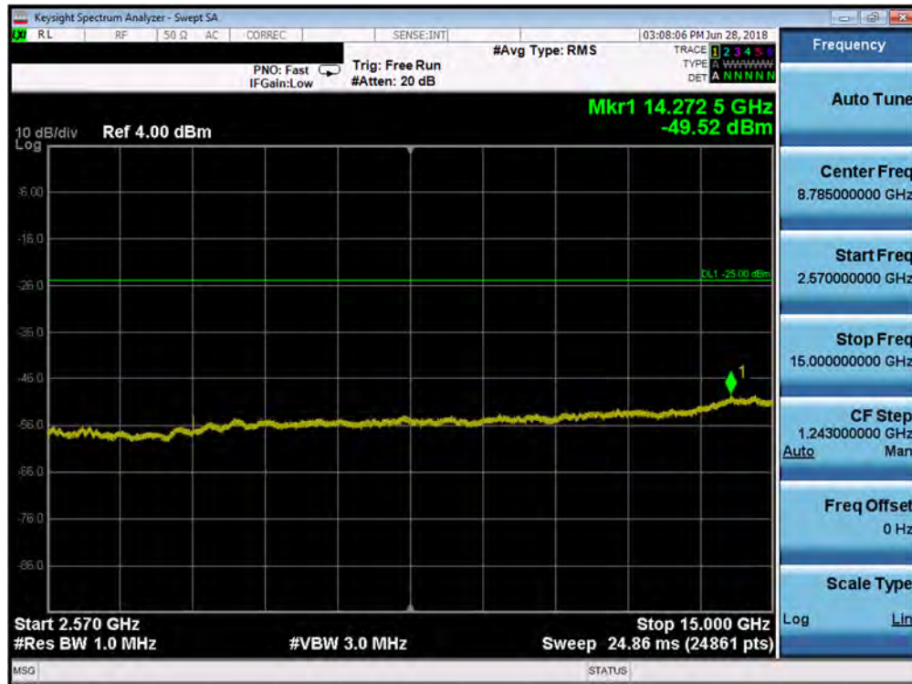
Plot 7-89. Conducted Spurious Plot (Band 7 - 5.0MHz QPSK - RB Size 1, RB Offset 0 - Mid Channel)
