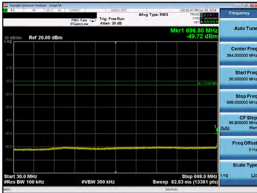
Plot 7-52. Conducted Spurious Plot (Band 12/17 - 5.0MHz QPSK - RB Size 1, RB Offset 0 - Mid Channel)
