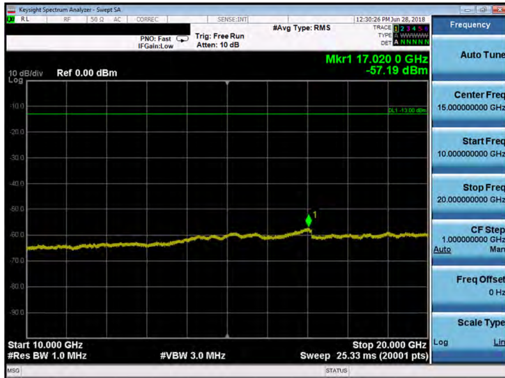
Plot 7-84. Conducted Spurious Plot (Band 2 - 1.4MHz QPSK - RB Size 1, RB Offset 0 - High Channel)
