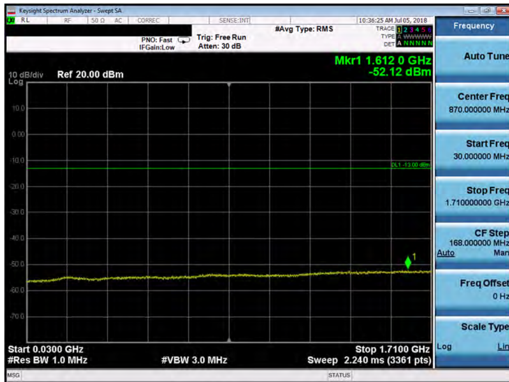
Plot 7-70. Conducted Spurious Plot (Band 66/4 - 1.4MHz QPSK - RB Size 1, RB Offset 0 - Mid Channel)
