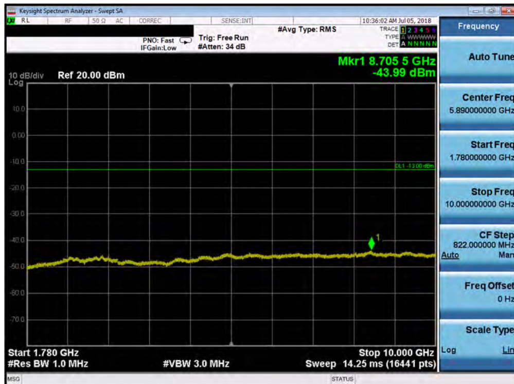
Plot 7-68. Conducted Spurious Plot (Band 66/4 - 1.4MHz QPSK - RB Size 1, RB Offset 0 - Low Channel)
