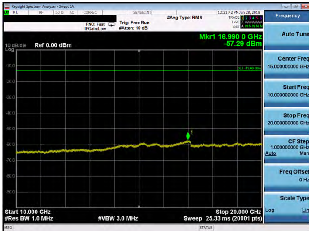
Plot 7-81. Conducted Spurious Plot (Band 2 - 1.4MHz QPSK - RB Size 1, RB Offset 0 - Mid Channel)
