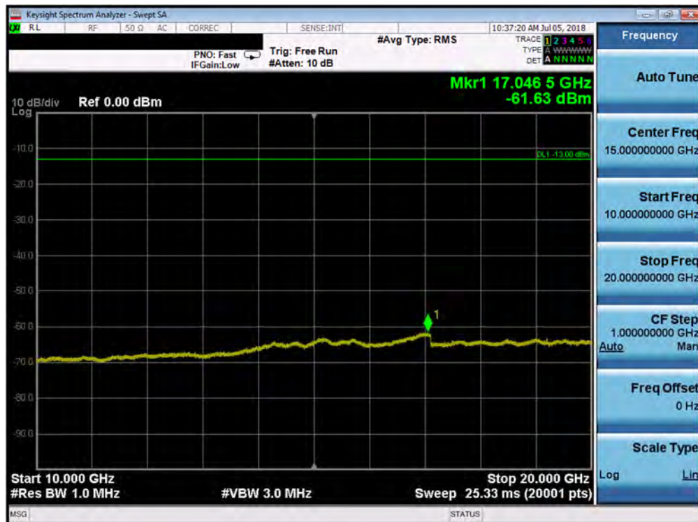
Plot 7-72. Conducted Spurious Plot (Band 66/4 - 1.4MHz QPSK - RB Size 1, RB Offset 0 - Mid Channel)
