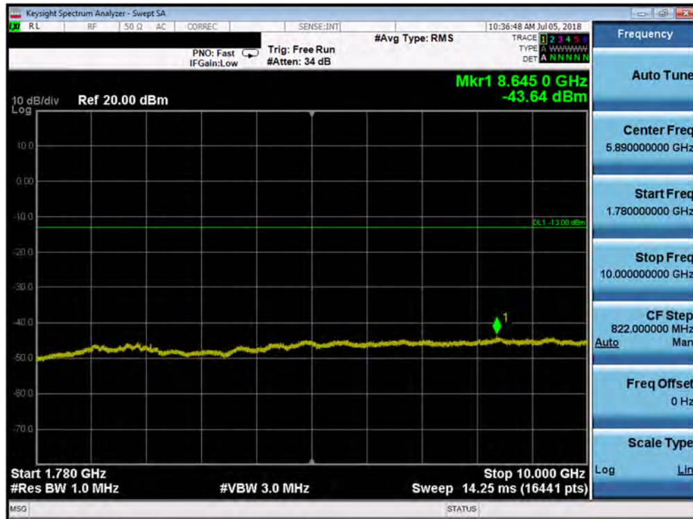
Plot 7-71. Conducted Spurious Plot (Band 66/4 - 1.4MHz QPSK - RB Size 1, RB Offset 0 - Mid Channel)
