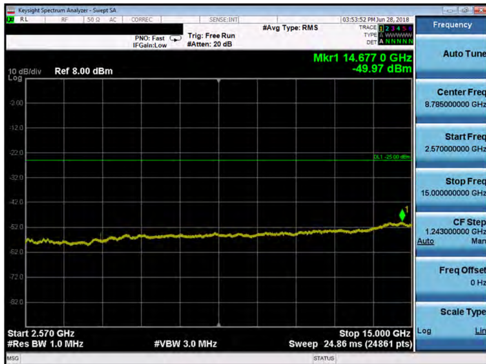
Plot 7-86. Conducted Spurious Plot (Band 7 - 5.0MHz QPSK - RB Size 1, RB Offset 0 - Low Channel)
