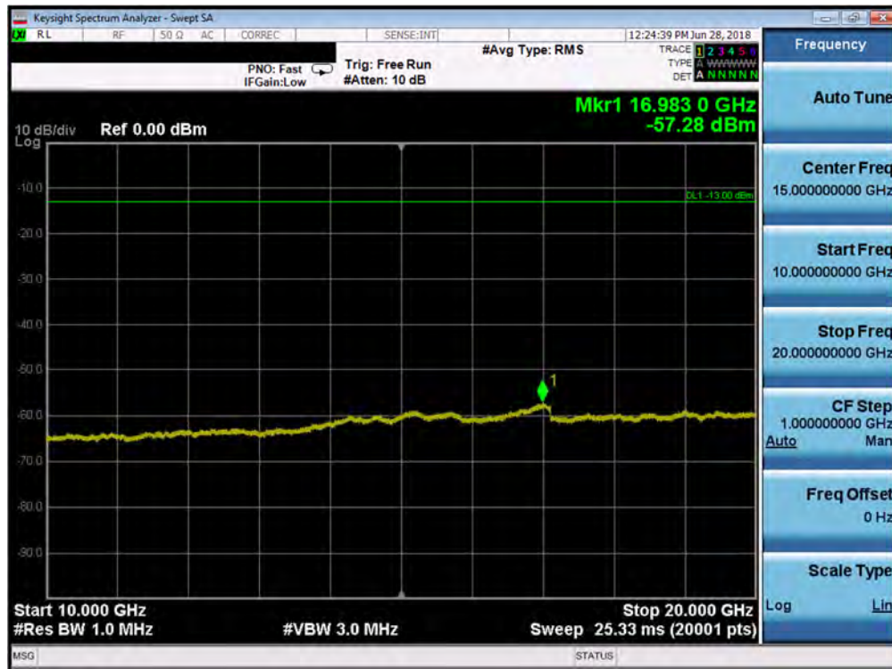
Plot 7-78. Conducted Spurious Plot (Band 2 - 1.4MHz QPSK - RB Size 1, RB Offset 0 - Low Channel)
