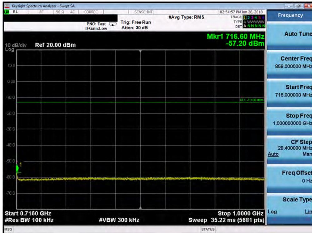
Plot 7-50. Conducted Spurious Plot (Band 12/17 - 5.0MHz QPSK - RB Size 1, RB Offset 0 - Low Channel)
