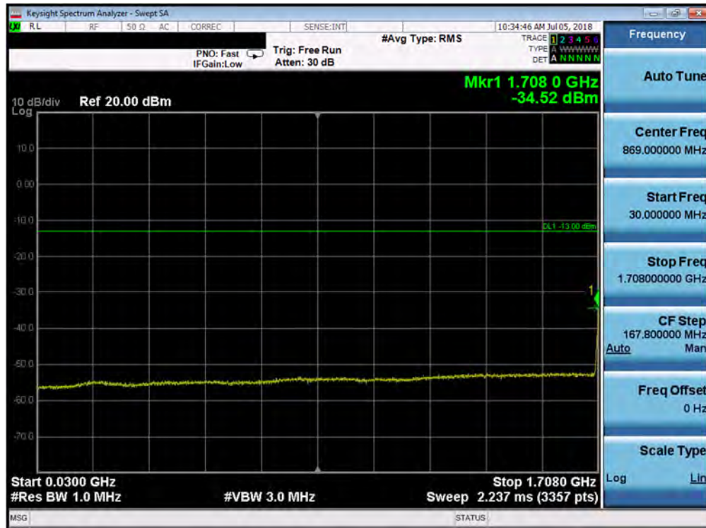
Plot 7-67. Conducted Spurious Plot (Band 66/4 - 1.4MHz QPSK - RB Size 1, RB Offset 0 - Low Channel)
