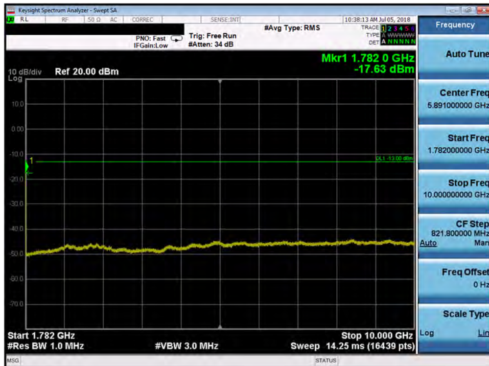
Plot 7-74. Conducted Spurious Plot (Band 66/4 - 1.4MHz QPSK - RB Size 1, RB Offset 0 - High Channel)
