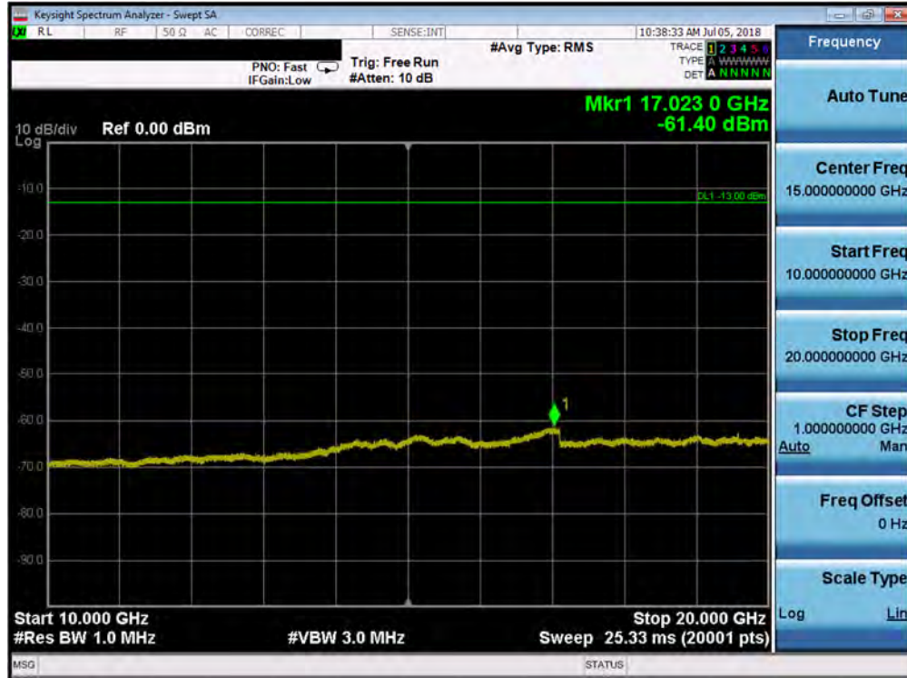
Plot 7-75. Conducted Spurious Plot (Band 66/4 - 1.4MHz QPSK - RB Size 1, RB Offset 0 - High Channel)
