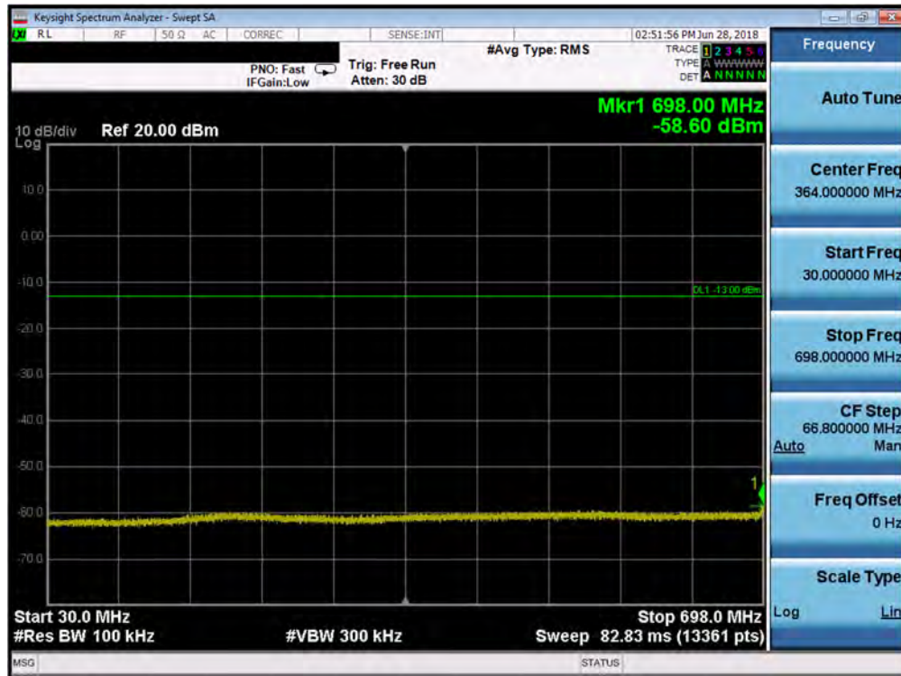
Plot 7-55. Conducted Spurious Plot (Band 12/17 - 5.0MHz QPSK - RB Size 1, RB Offset 0 - High Channel)
