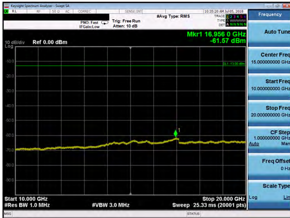
Plot 7-69. Conducted Spurious Plot (Band 66/4 - 1.4MHz QPSK - RB Size 1, RB Offset 0 - Low Channel)
