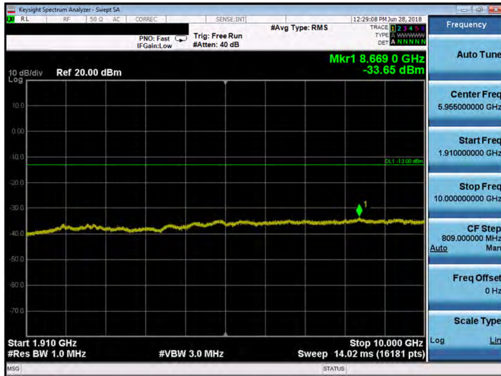
Plot 7-80. Conducted Spurious Plot (Band 2 - 1.4MHz QPSK - RB Size 1, RB Offset 0 - Mid Channel)
