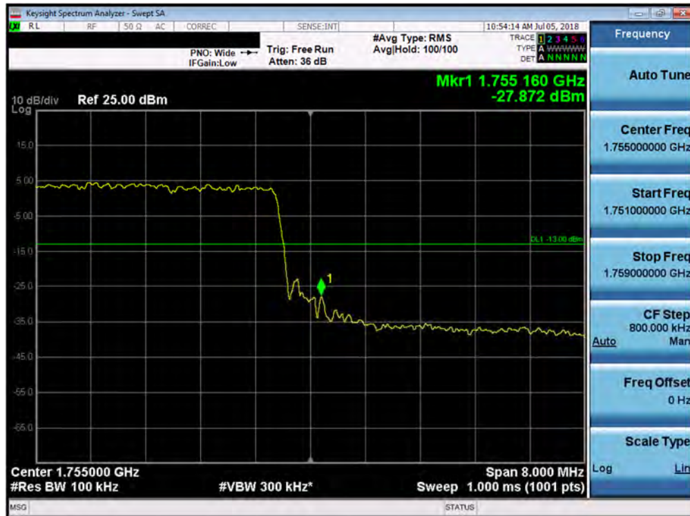
Plot 7-132. Upper Band Edge Plot (Band 4 - 10.0MHz QPSK - Full RB Configuration)
