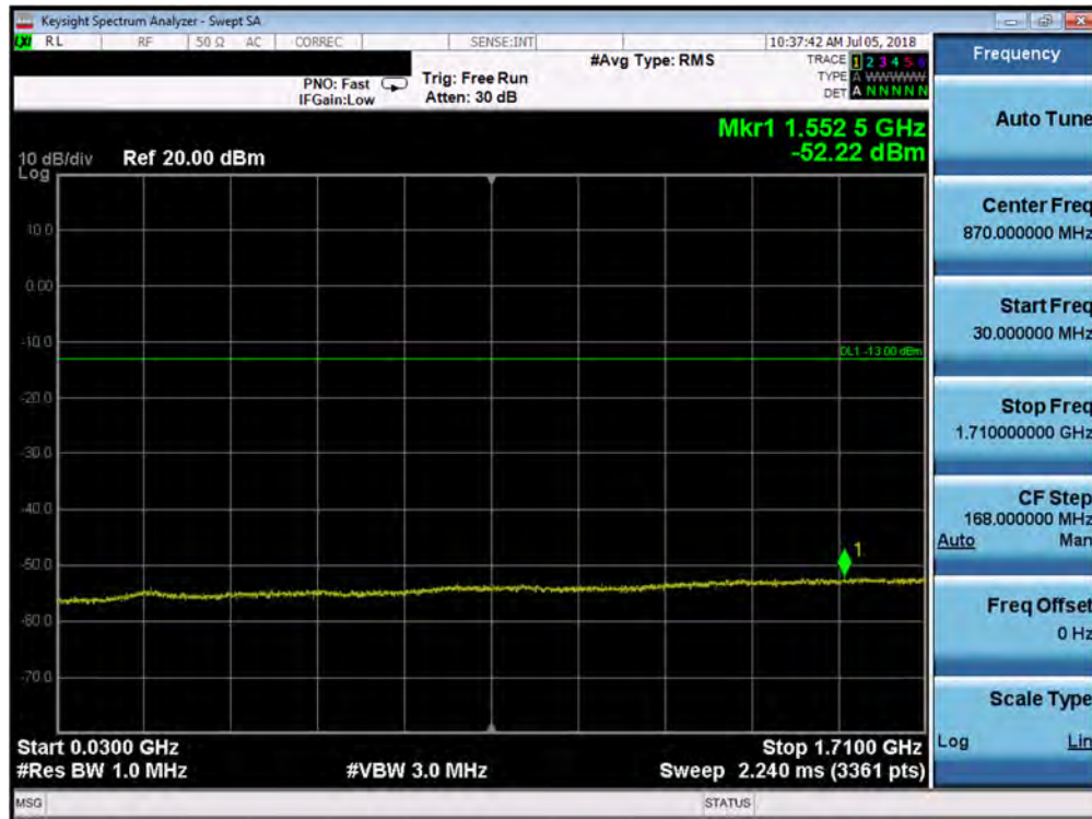
Plot 7-73. Conducted Spurious Plot (Band 66/4 - 1.4MHz QPSK - RB Size 1, RB Offset 0 - High Channel)
