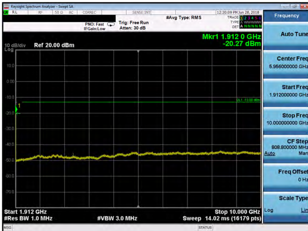
Plot 7-83. Conducted Spurious Plot (Band 2 - 1.4MHz QPSK - RB Size 1, RB Offset 0 - High Channel)
