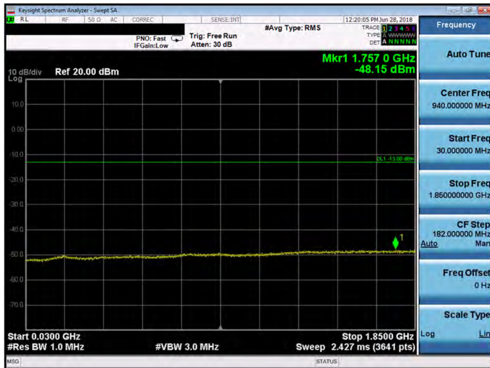
Plot 7-79. Conducted Spurious Plot (Band 2 - 1.4MHz QPSK - RB Size 1, RB Offset 0 - Mid Channel)
