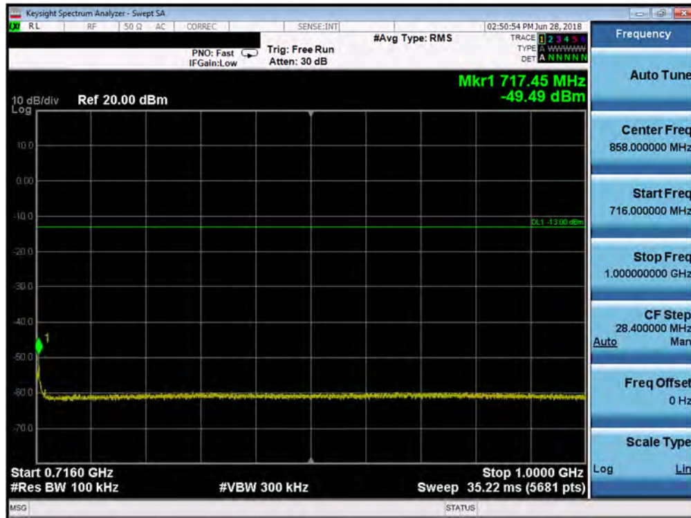
Plot 7-53. Conducted Spurious Plot (Band 12/17 - 5.0MHz QPSK - RB Size 1, RB Offset 0 - Mid Channel)
