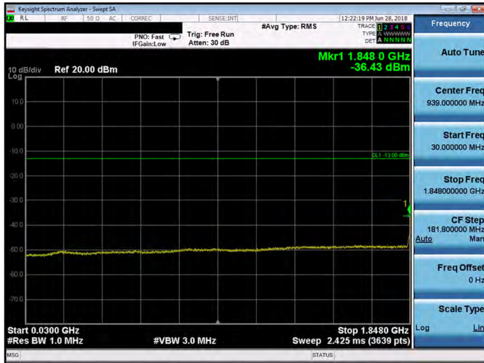
Plot 7-76. Conducted Spurious Plot (Band 2 - 1.4MHz QPSK - RB Size 1, RB Offset 0 - Low Channel)
