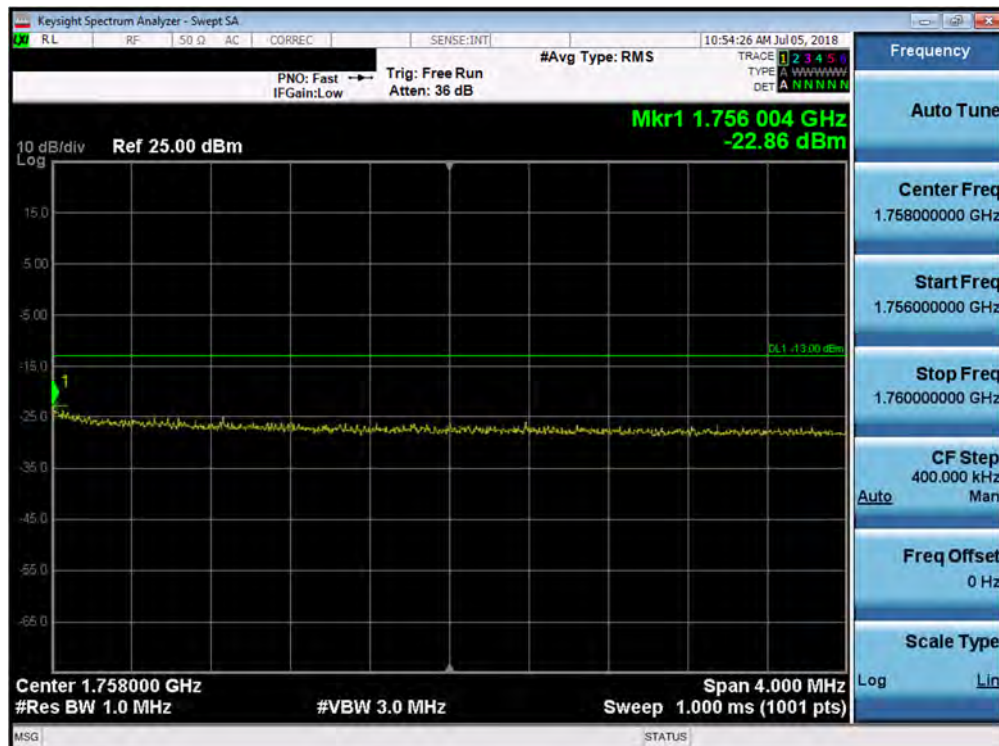
Plot 7-133. Upper Extended Band Edge Plot (Band 4 - 10.0MHz QPSK - Full RB Configuration)
