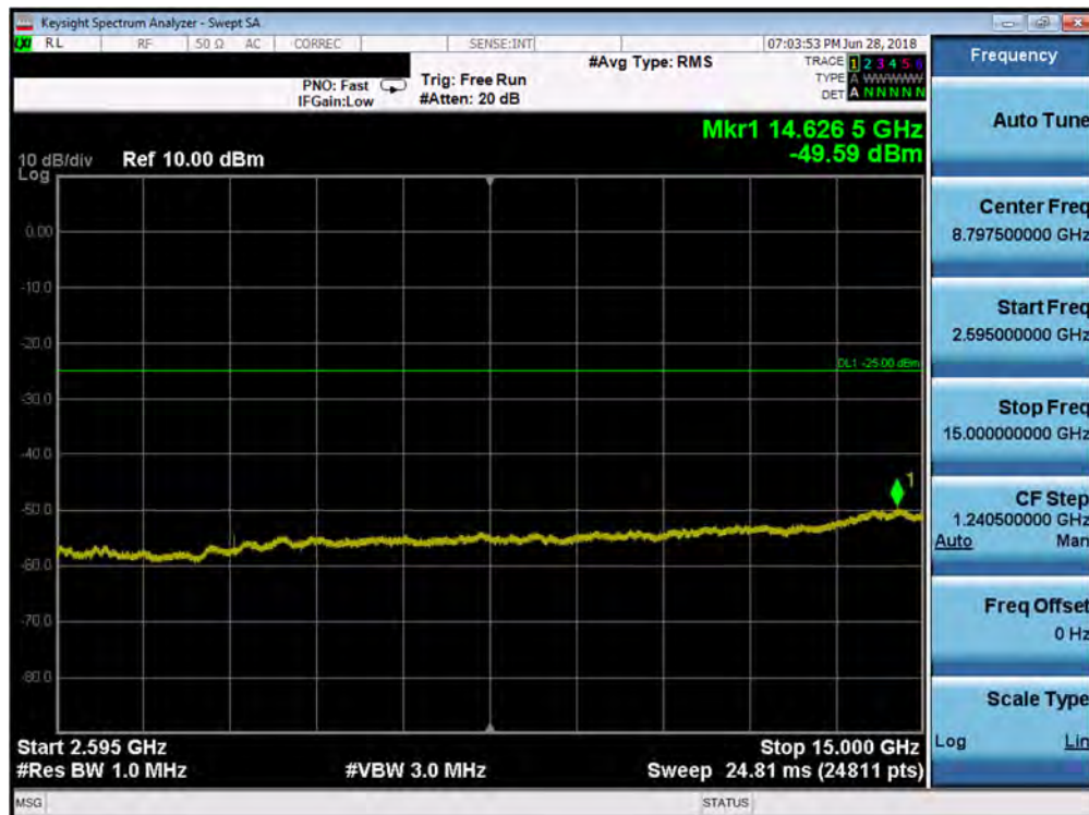
Plot 7-92. Conducted Spurious Plot (Band 7 - 5.0MHz QPSK - RB Size 1, RB Offset 0 - High Channel)
