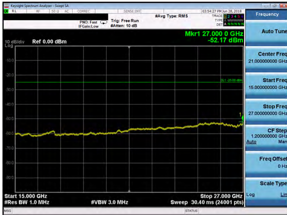
Plot 7-87. Conducted Spurious Plot (Band 7 - 5.0MHz QPSK - RB Size 1, RB Offset 0 - Low Channel)
