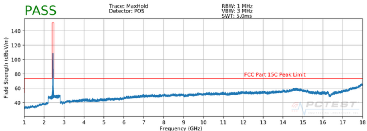
Plot 7-33. Radiated Spurious Plot above 1GHz (802.11b – Ch. 1, Ant. Pol. H)
