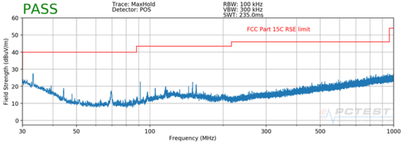
Plot 7-48. Radiated Spurious Plot below 1GHz (Ant. Pol. V)
