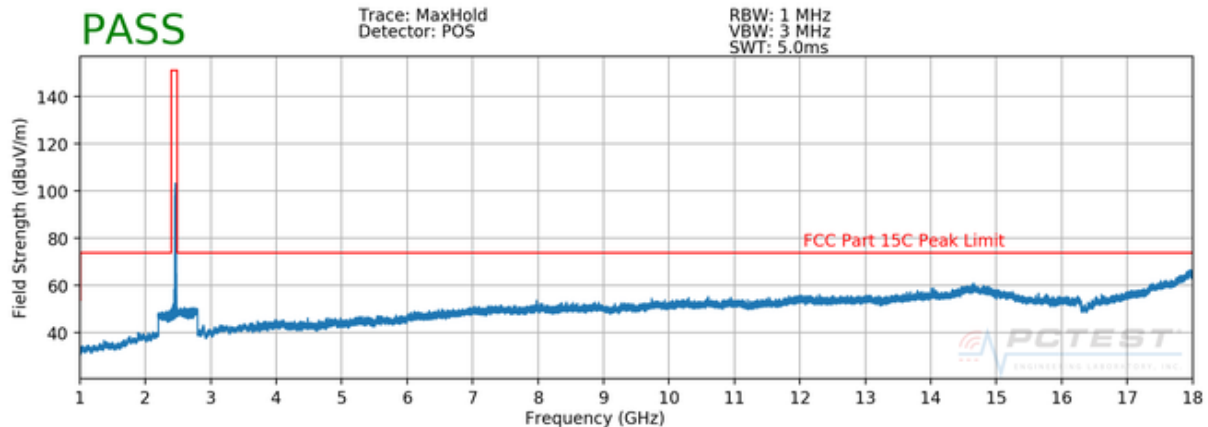
Plot 7-36. Radiated Spurious Plot above 1GHz (802.11b – Ch. 1, Ant. Pol. V)
