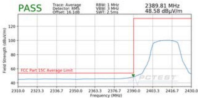
Plot 7-39. Radiated Restricted Lower Band Edge Measurement (Average)
