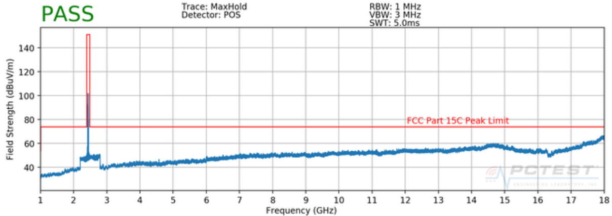
Plot 7-34. Radiated Spurious Plot above 1GHz (802.11b – Ch. 1, Ant. Pol. V)
