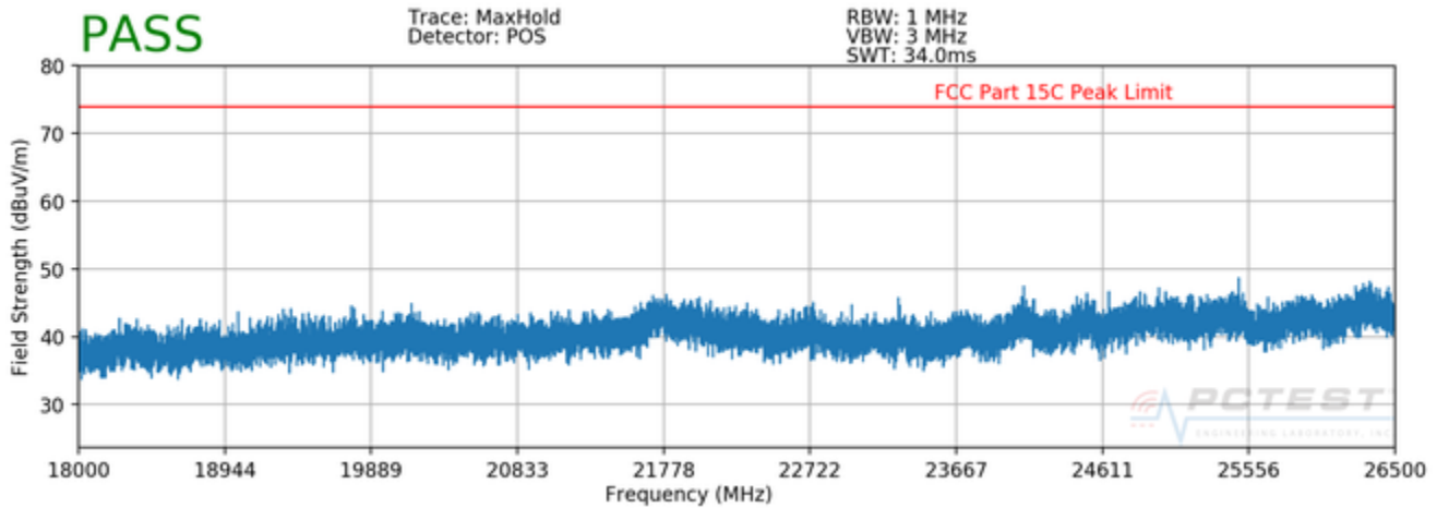
Plot 7-38. Radiated Spurious Plot above 18GHz (Ant. Pol. H)
