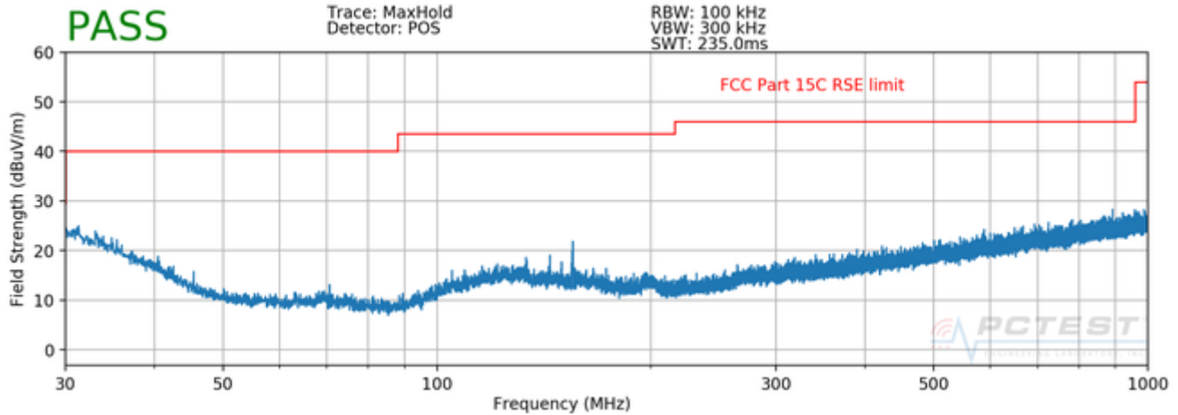
Plot 7-47. Radiated Spurious Plot below 1GHz (Ant. Pol. H)
