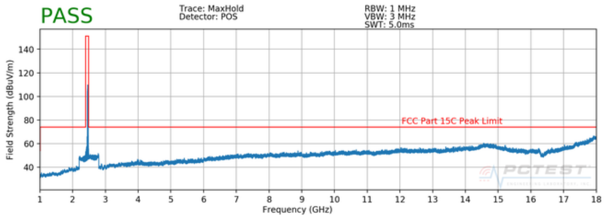
Plot 7-35. Radiated Spurious Plot above 1GHz (802.11b – Ch. 1, Ant. Pol. H)
