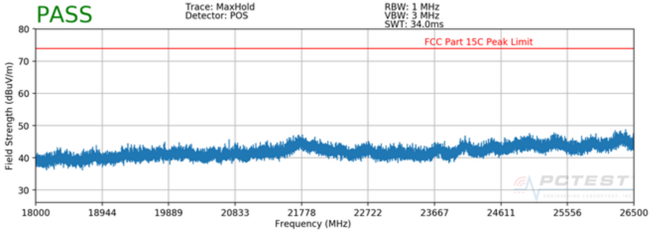
Plot 7-37. Radiated Spurious Plot above 18GHz (Ant. Pol. H)
