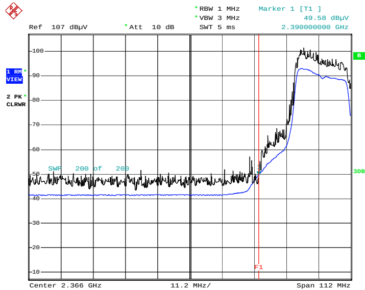
Radiated Restricted Band Edges plot – Average Reading (802.11n Ch.1)
