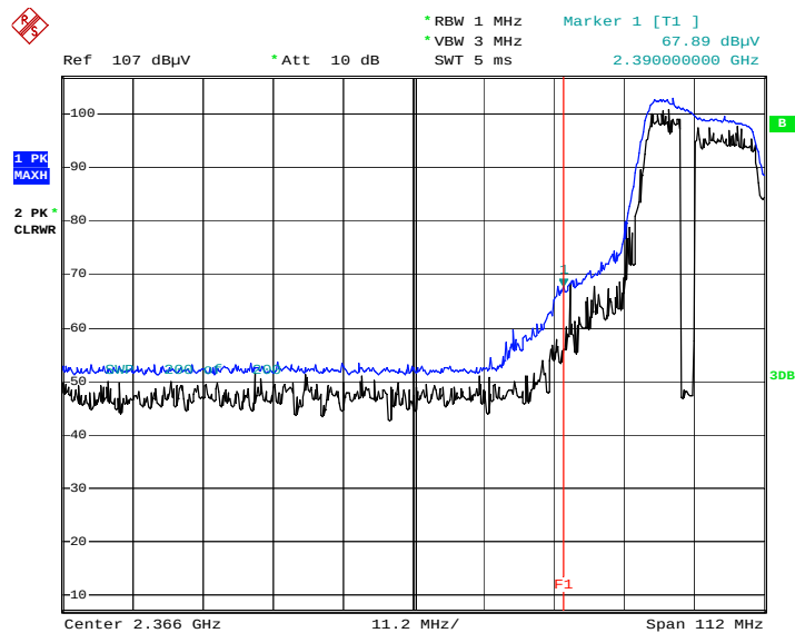
Radiated Restricted Band Edges plot – Peak Reading (802.11n Ch.1)
