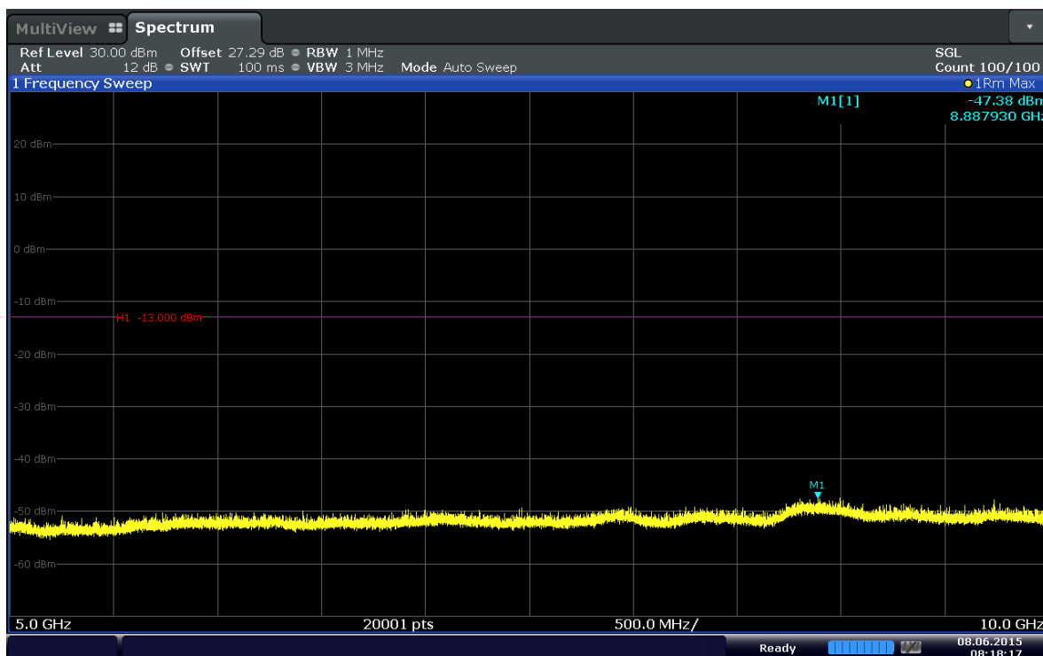
Plot 6-12. Conducted Spurious Plot (Band 5–1.4MHz–QPSK–RB Size 3–RB Offset 0–Ch.20525)
