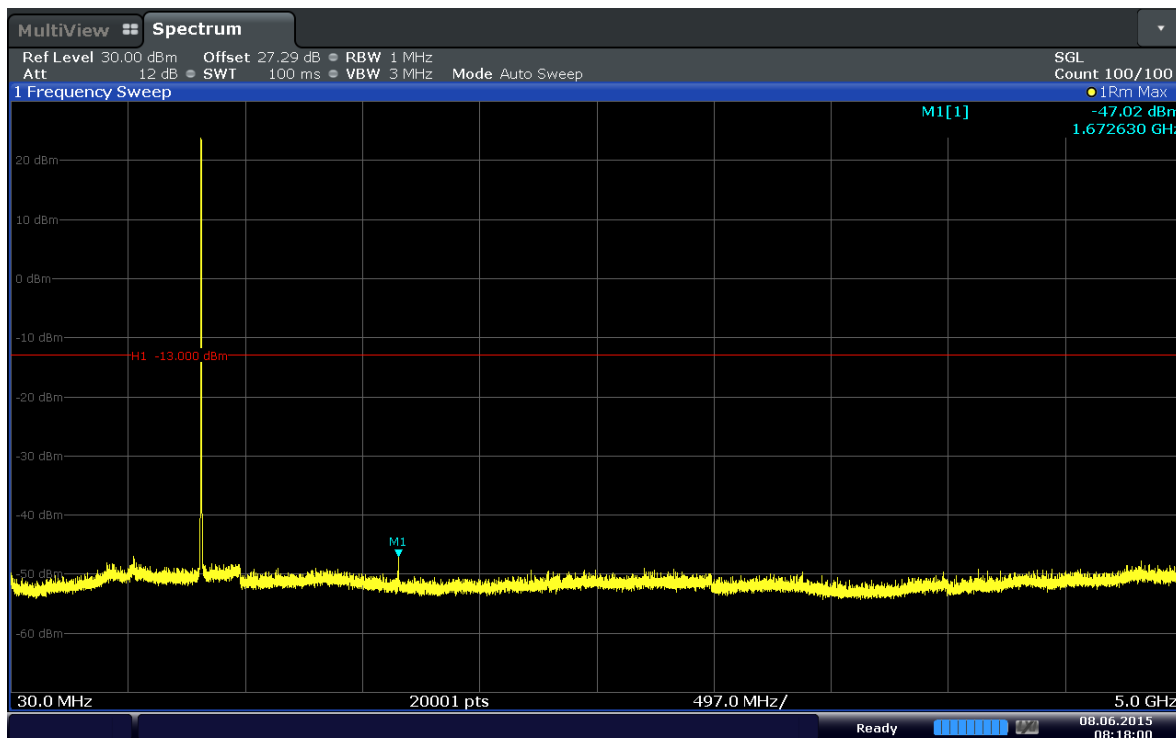
Plot 6-11. Conducted Spurious Plot (Band 5–1.4MHz–QPSK–RB Size 3–RB Offset 0–Ch.20525)
