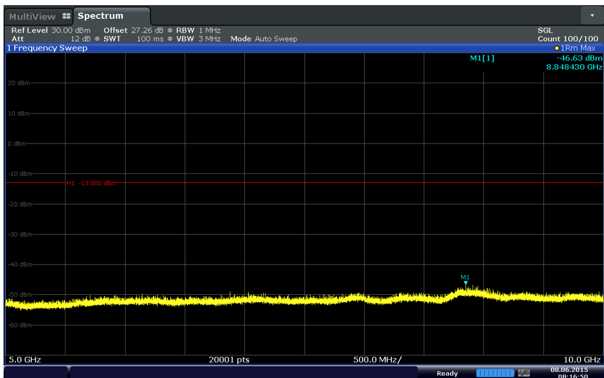
Plot 6-9. Conducted Spurious Plot (Band 5–1.4MHz–QPSK–RB Size 1–RB Offset 0–Ch.20407)
