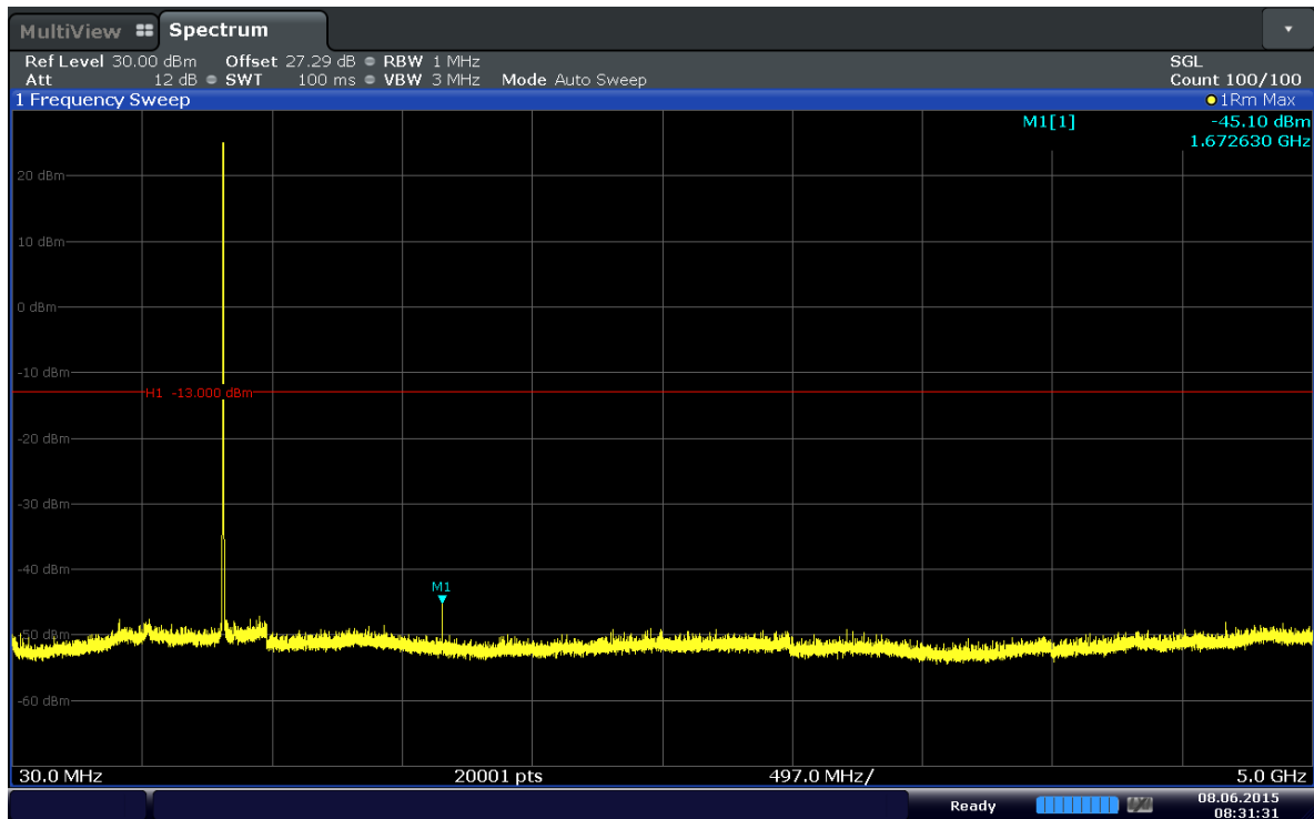
Plot 6-29. Conducted Spurious Plot (Band 5–10.0MHz–QPSK–RB Size 1–RB Offset 24– Ch.20525)
