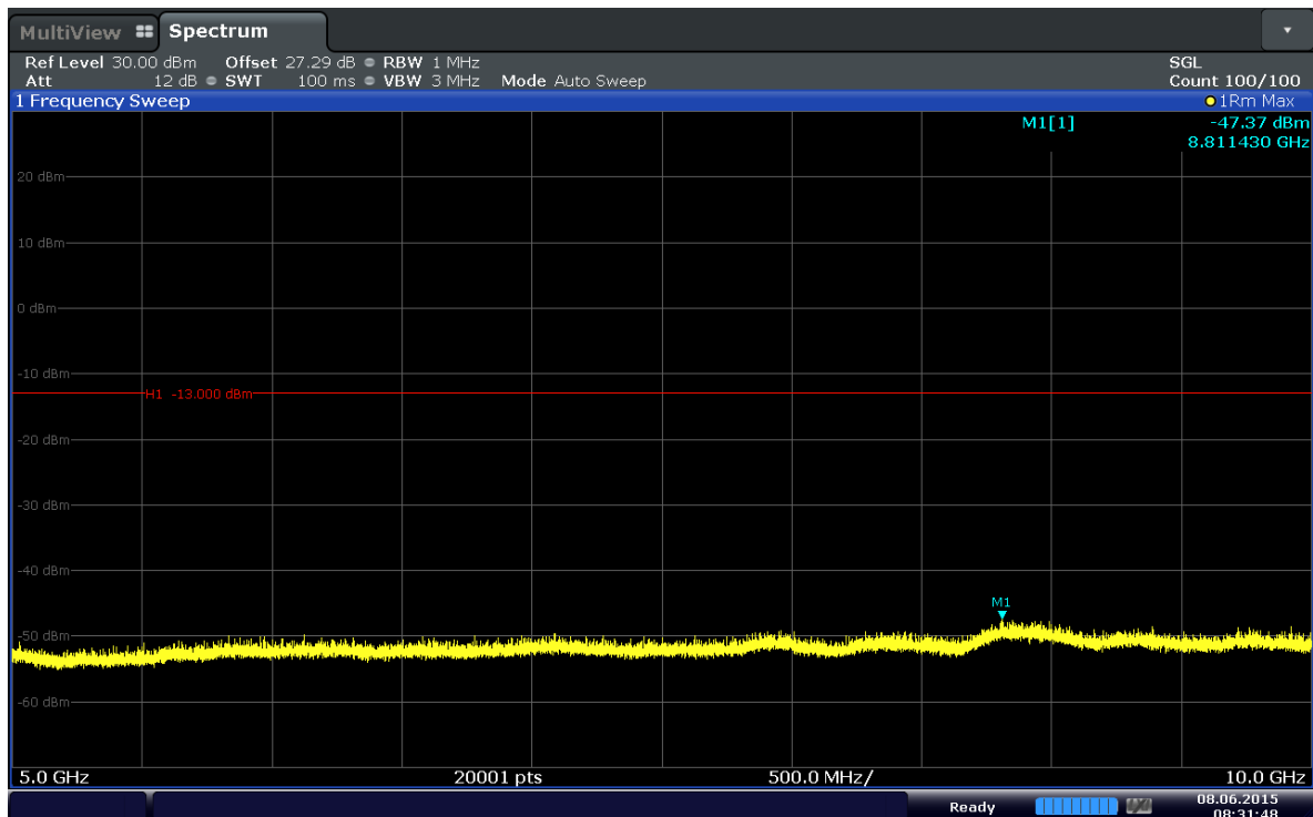
Plot 6-30. Conducted Spurious Plot (Band 5–10.0MHz–QPSK–RB Size 1–RB Offset 24– Ch.20525)
