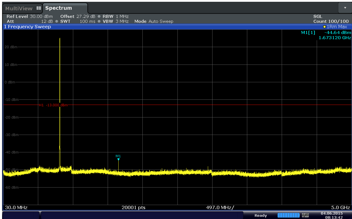
Plot 6-23. Conducted Spurious Plot (Band 5–5.0MHz–QPSK–RB Size 1–RB Offset 12– Ch.20525)
