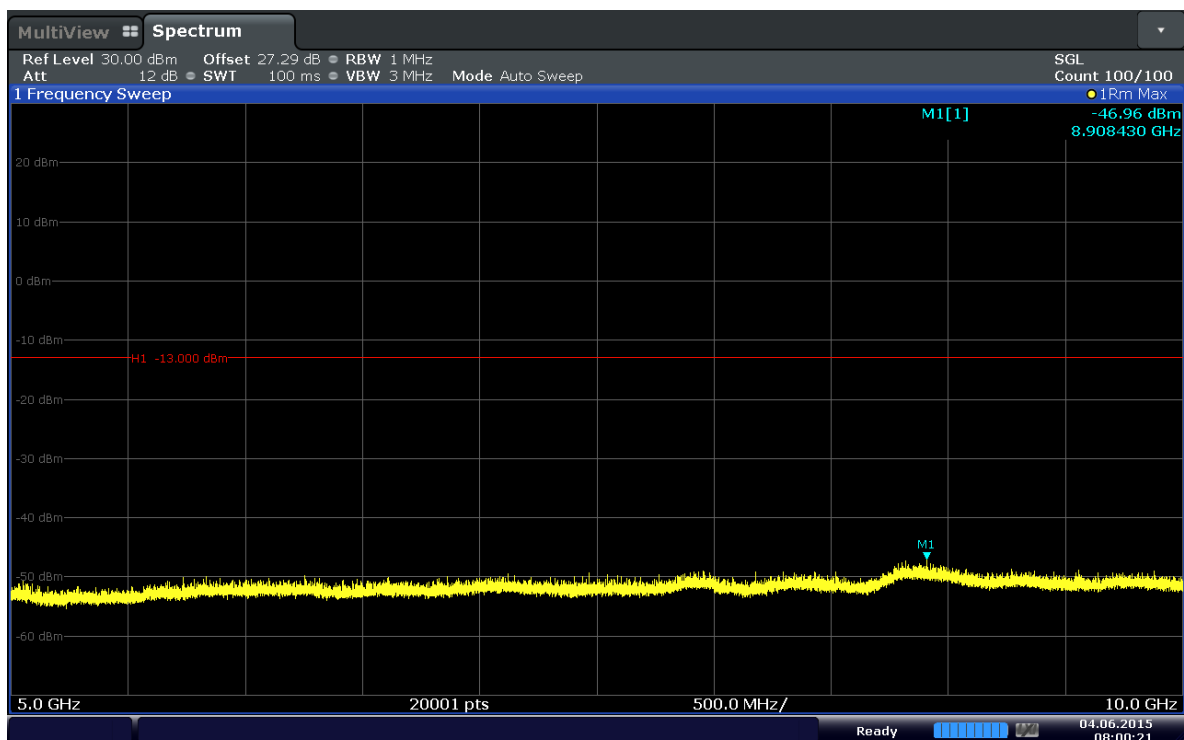
Plot 6-14. Conducted Spurious Plot (Band 5–1.4MHz–QPSK–RB Size 3–RB Offset 2– Ch.20643)
