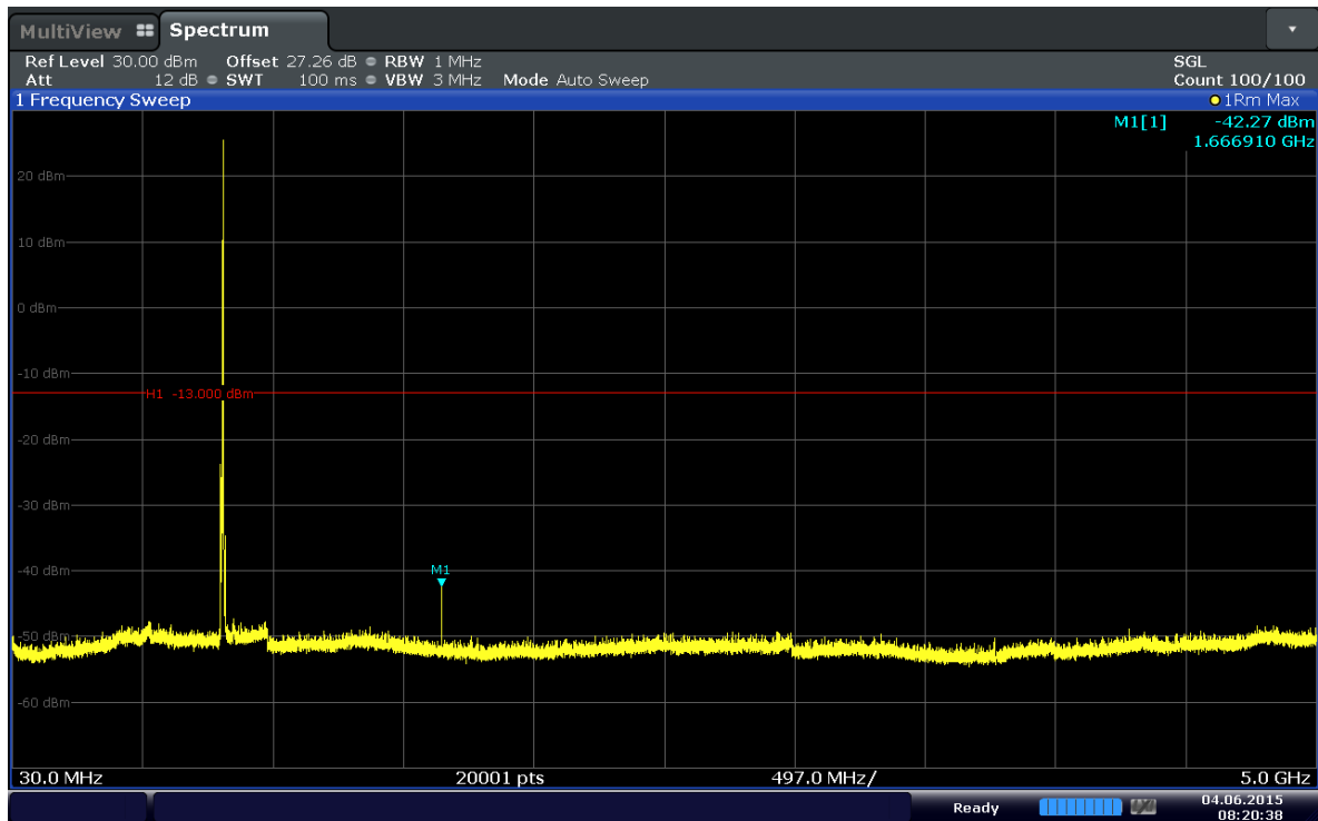
Plot 6-27. Conducted Spurious Plot (Band 5–10.0MHz–QPSK–RB Size 1–RB Offset 49– Ch.20450)
