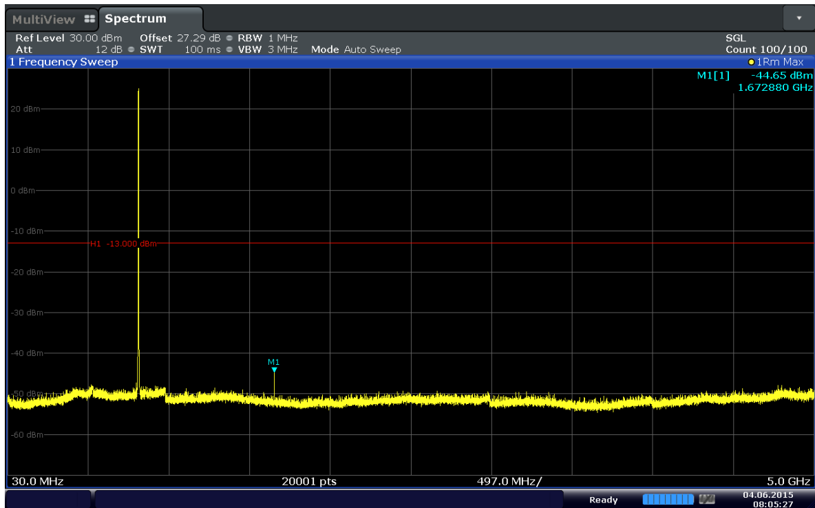
Plot 6-17. Conducted Spurious Plot (Band 5–3.0MHz–QPSK–RB Size 1–RB Offset 7– Ch.20525)
