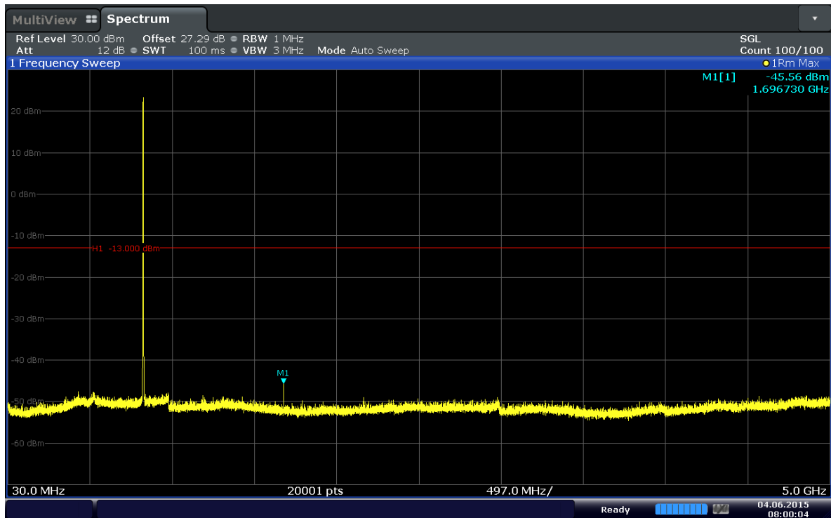
Plot 6-13. Conducted Spurious Plot (Band 5–1.4MHz–QPSK–RB Size 3–RB Offset 2– Ch.20643)
