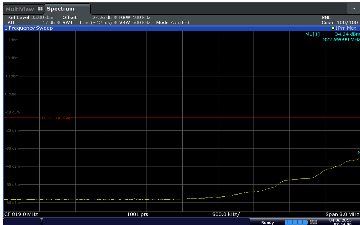
Plot 6-34. Extended Lower Band Edge Plot (Band5 – 1.4MHz – QPSK – RB Size 6)
