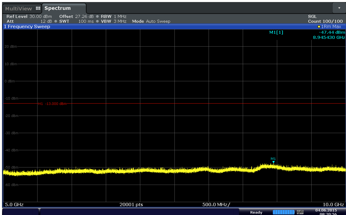
Plot 6-28. Conducted Spurious Plot (Band 5–10.0MHz–QPSK–RB Size 1–RB Offset 49– Ch.20450)
