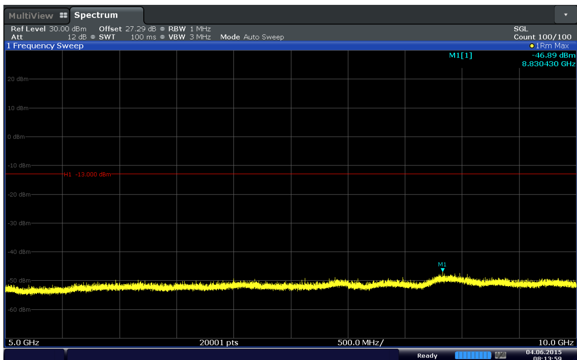
Plot 6-24. Conducted Spurious Plot (Band 5–5.0MHz–QPSK–RB Size 1–RB Offset 12– Ch.20525)
