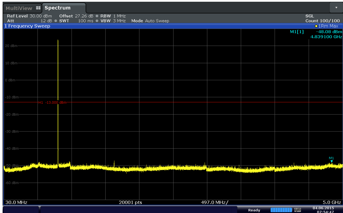
Plot 6-9. Conducted Spurious Plot (Band 5–1.4MHz–QPSK–RB Size 3–RB Offset 0–Ch.20407)
