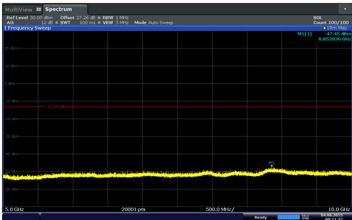
Plot 6-22. Conducted Spurious Plot (Band 5–5.0MHz–QPSK–RB Size 1–RB Offset 12– Ch.20425)
