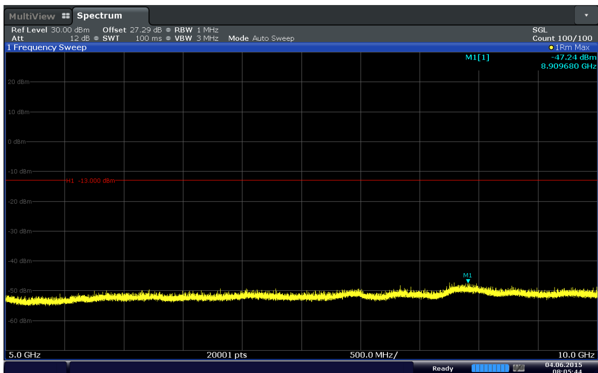
Plot 6-18. Conducted Spurious Plot (Band 5–3.0MHz–QPSK–RB Size 1–RB Offset 7– Ch.20525)
