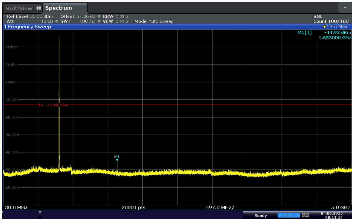
Plot 6-21. Conducted Spurious Plot (Band 5–5.0MHz–QPSK–RB Size 1–RB Offset 12– Ch.20425)
