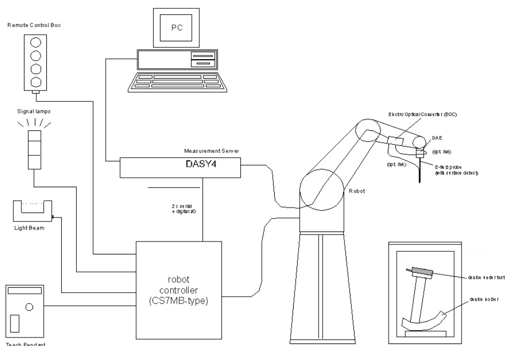
Figure 3.1 SPEAG Robotic System Description
