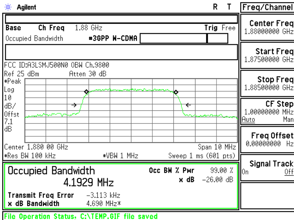
Plot 6-3. Occupied Bandwidth Plot (PCS WCDMA Mode - Ch.9400(DL9800))
