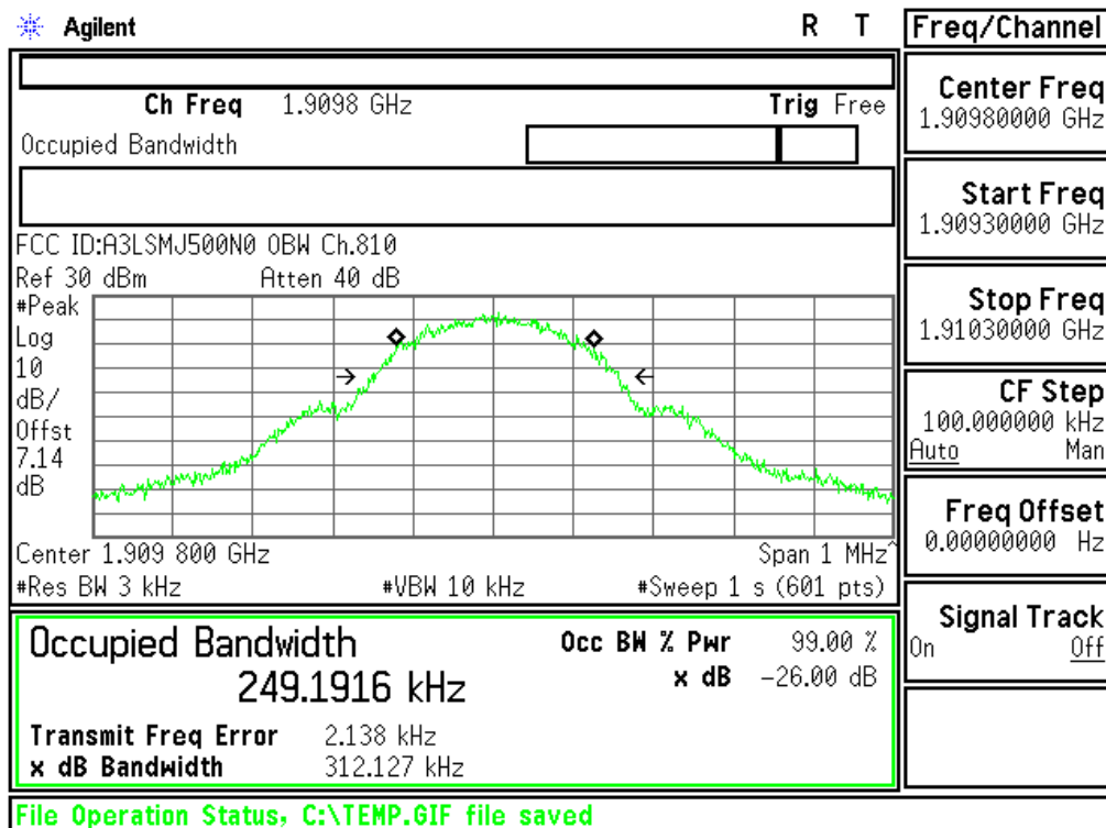
Plot 6-1. Occupied Bandwidth Plot (PCS GSM Mode - Ch.810)
