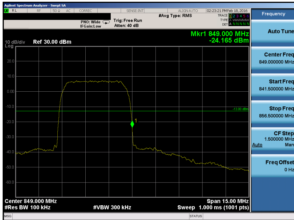
Plot 7-50. Band Edge Plot (Cellular WCDMA Mode – Ch. 4233)
