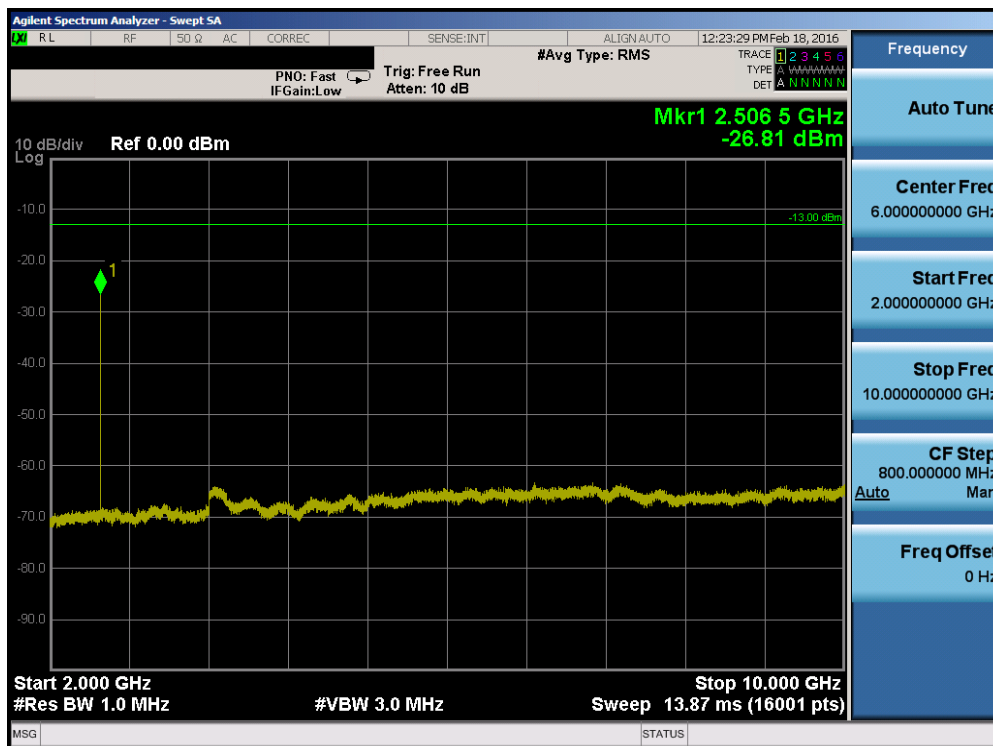
Plot 7-14. Conducted Spurious Plot (Band 5 – 3.0MHz QPSK – RB Size 1, RB Offset 0 – Mid Channel)
