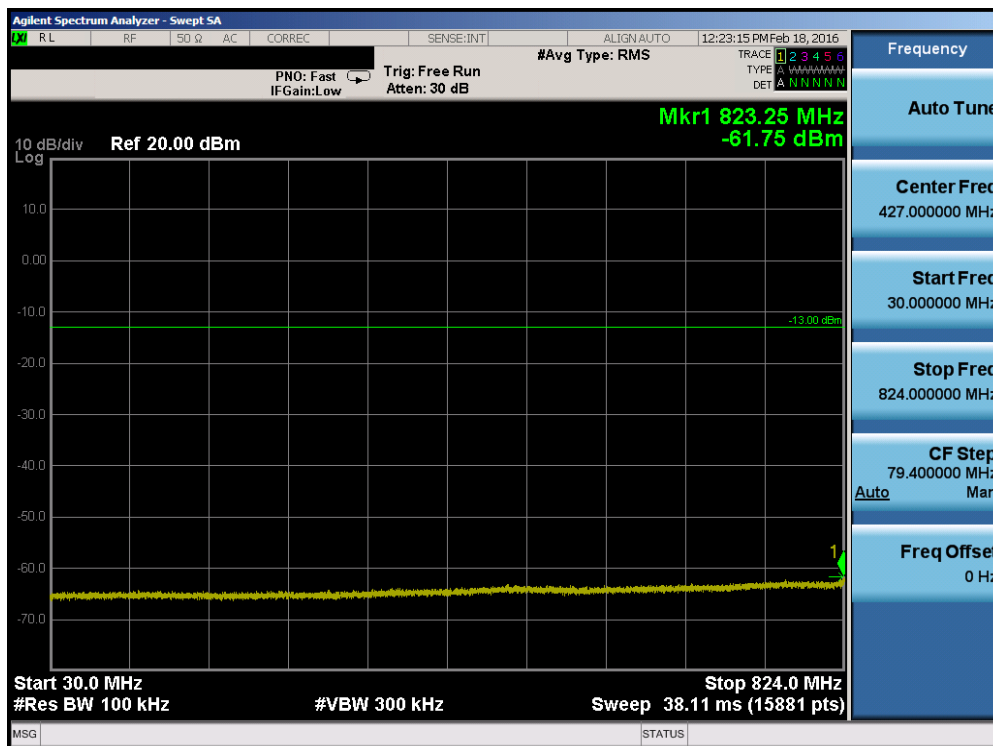
Plot 7-12. Conducted Spurious Plot (Band 5 – 3.0MHz QPSK – RB Size 1, RB Offset 0 – Mid Channel)
