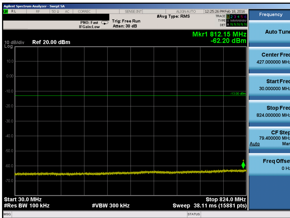
Plot 7-15. Conducted Spurious Plot (Band 5 – 3.0MHz QPSK – RB Size 1, RB Offset 0 – High Channel)
