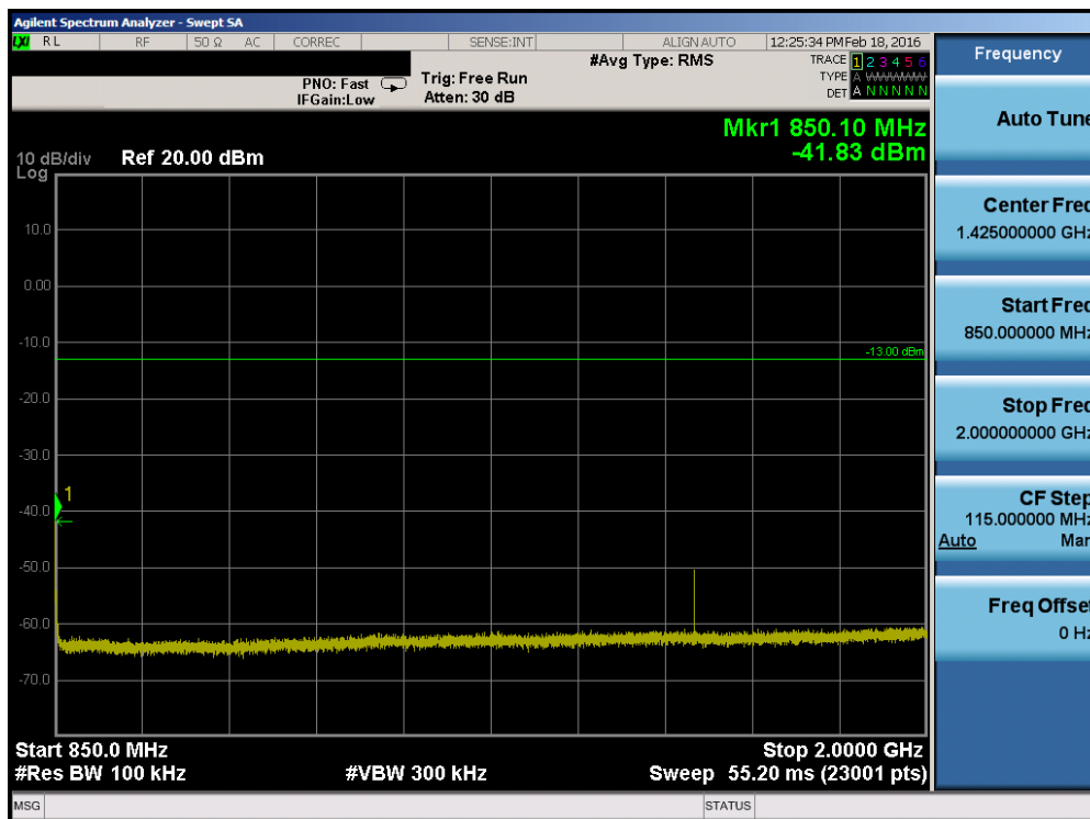
Plot 7-16. Conducted Spurious Plot (Band 5 – 3.0MHz QPSK – RB Size 1, RB Offset 0 – High Channel)
