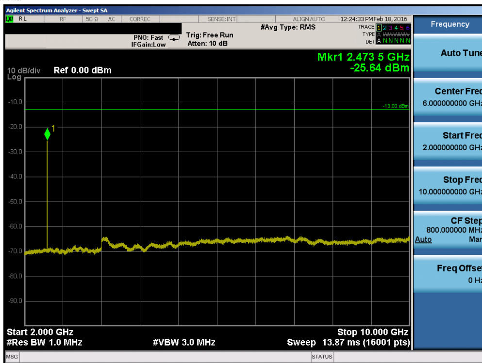
Plot 7-11. Conducted Spurious Plot (Band 5 – 3.0MHz QPSK – RB Size 1, RB Offset 0 – Low Channel)
