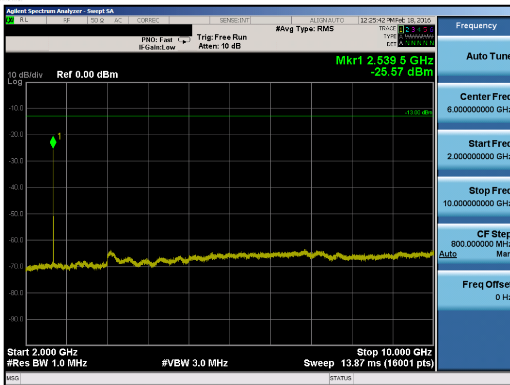
Plot 7-17. Conducted Spurious Plot (Band 5 – 3.0MHz QPSK – RB Size 1, RB Offset 0 – High Channel)
