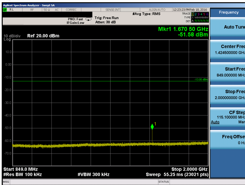
Plot 7-13. Conducted Spurious Plot (Band 5 – 3.0MHz QPSK – RB Size 1, RB Offset 0 – Mid Channel)
