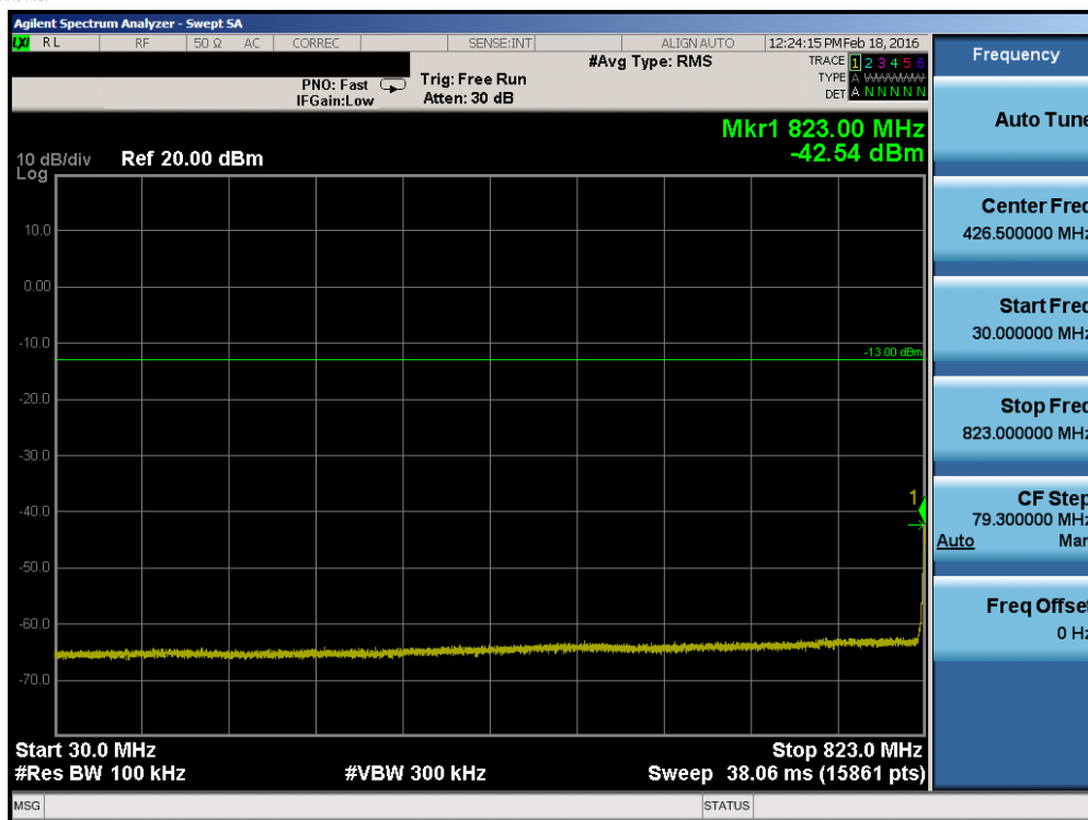
Plot 7-9. Conducted Spurious Plot (Band 5 – 3.0MHz QPSK – RB Size 1, RB Offset 0 – Low Channel)
