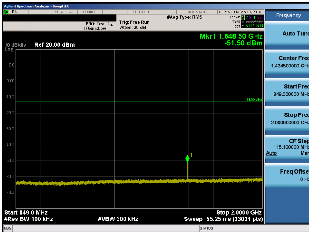
Plot 7-10. Conducted Spurious Plot (Band 5 – 3.0MHz QPSK – RB Size 1, RB Offset 0 – Low Channel)
