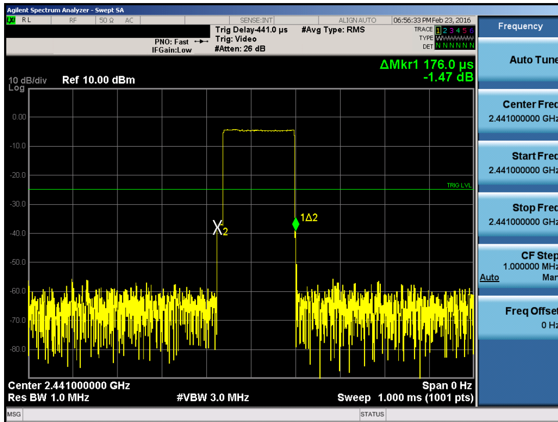
Plot 7-2. Pulse Width Measurement
