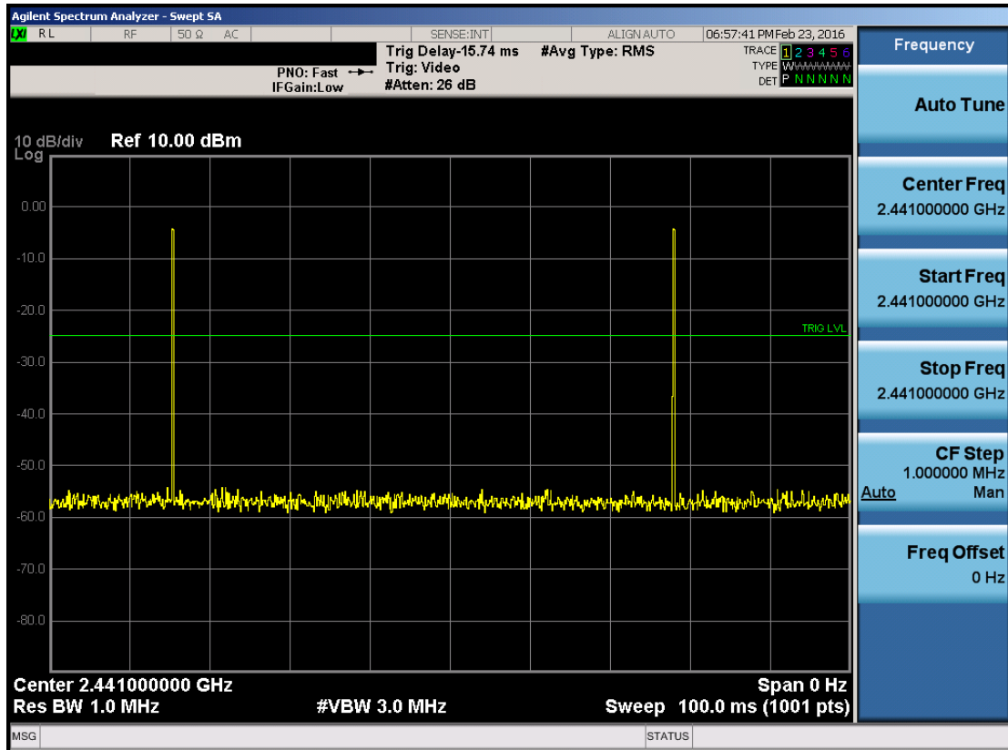
Plot 7-3. Worst Case 100ms Operation
