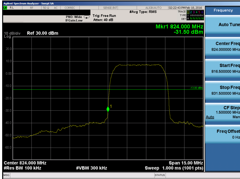
Plot 7-49. Band Edge Plot (Cellular WCDMA Mode – Ch. 4132)
