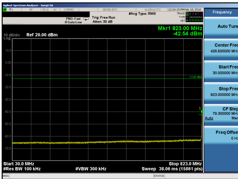
Plot 7-17. Conducted Spurious Plot (Band 5 – 3.0MHz QPSK – RB Size 1, RB Offset 0 – Low Channel)
