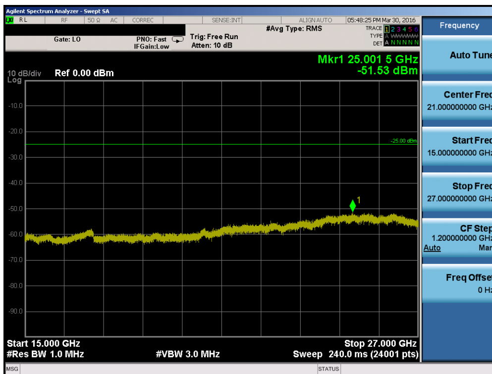
Plot 7-28. Conducted Spurious Plot (Band 41 – 10.0MHz QPSK – RB Size 1, RB Offset 0 – Low Channel)
