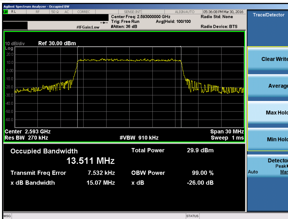
Plot 7-13. Occupied Bandwidth Plot (Band 41 – 15.0MHz QPSK – RB Size 75)
