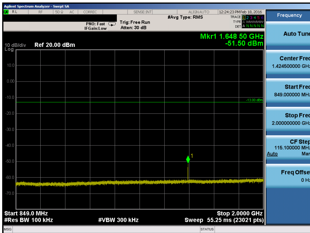
Plot 7-18. Conducted Spurious Plot (Band 5 – 3.0MHz QPSK – RB Size 1, RB Offset 0 – Low Channel)
