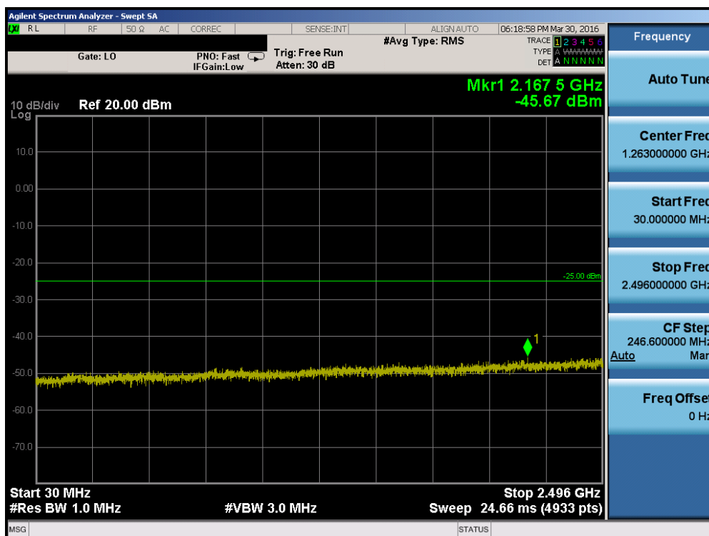
Plot 7-32. Conducted Spurious Plot (Band 41 – 10.0MHz QPSK – RB Size 1, RB Offset 0 – High Channel)
