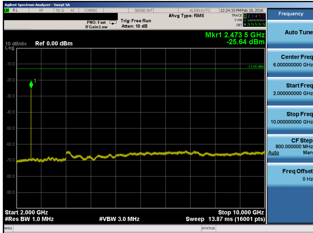
Plot 7-19. Conducted Spurious Plot (Band 5 – 3.0MHz QPSK – RB Size 1, RB Offset 0 – Low Channel)
