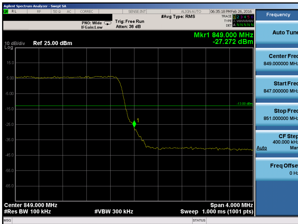
Plot 7-40. Upper Band Edge Plot (Band 5 – 5.0MHz QPSK – RB Size 25)
