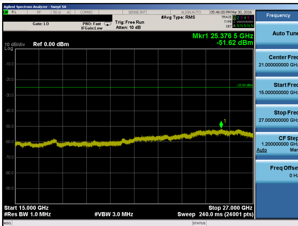
Plot 7-31. Conducted Spurious Plot (Band 41 – 10.0MHz QPSK – RB Size 1, RB Offset 0 – Mid Channel)
