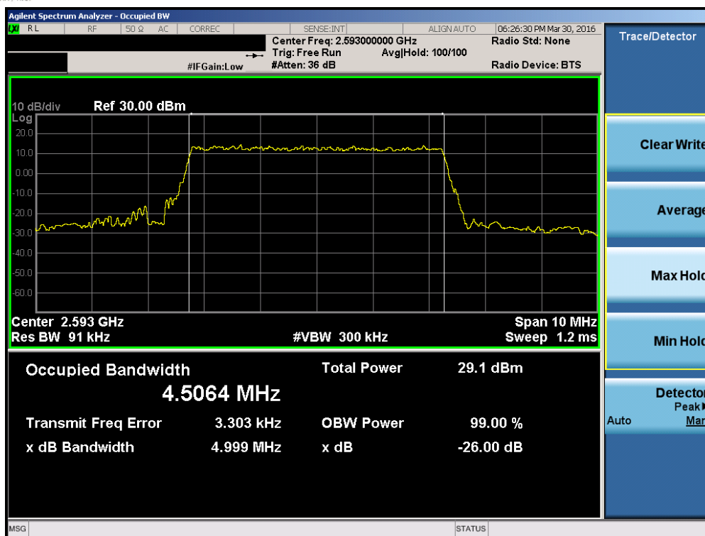
Plot 7-9. Occupied Bandwidth Plot (Band 41 – 5.0MHz QPSK – RB Size 25)
