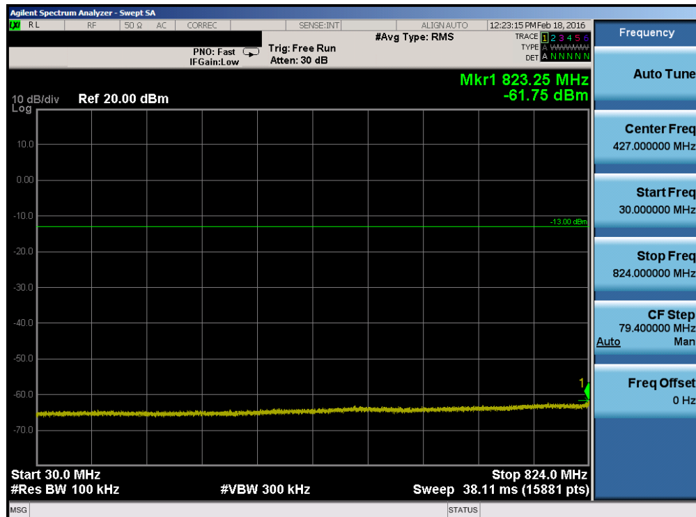
Plot 7-20. Conducted Spurious Plot (Band 5 – 3.0MHz QPSK – RB Size 1, RB Offset 0 – Mid Channel)
