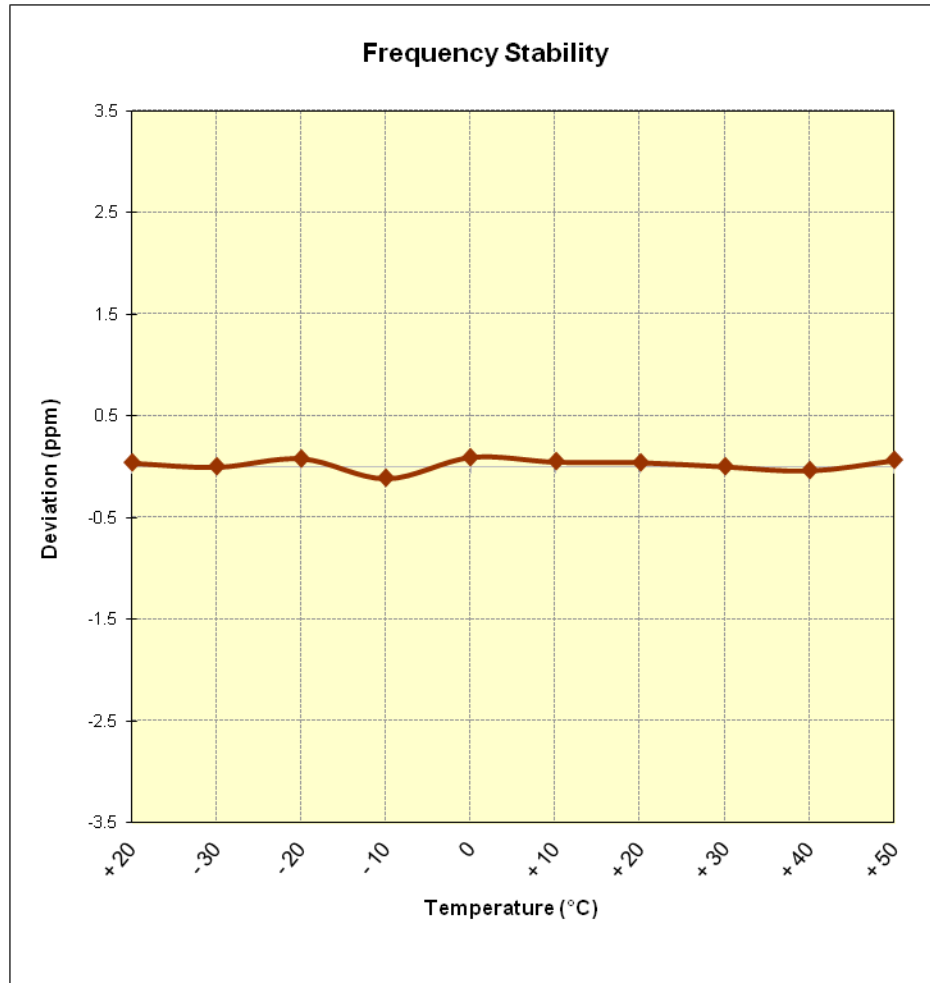
Figure 7-8. Frequency Stability Graph (Band 41)
