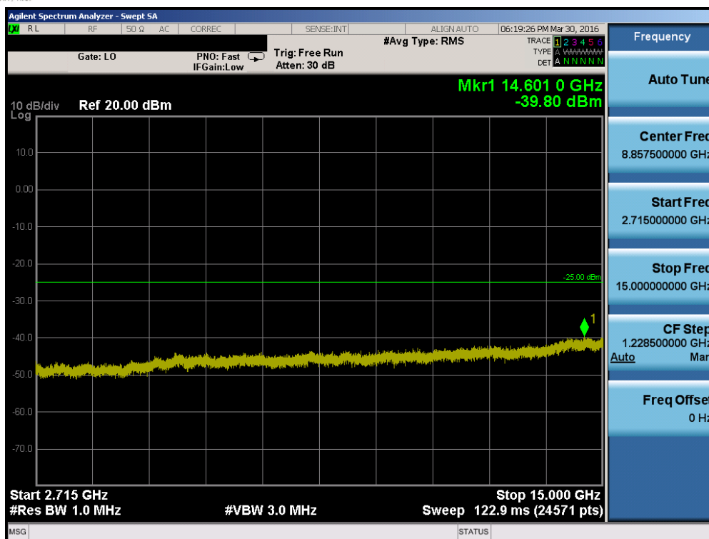
Plot 7-33. Conducted Spurious Plot (Band 41 – 10.0MHz QPSK – RB Size 1, RB Offset 0 – High Channel)
