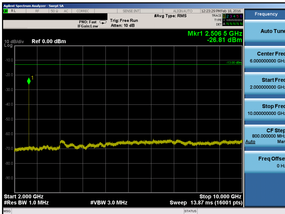
Plot 7-22. Conducted Spurious Plot (Band 5 – 3.0MHz QPSK – RB Size 1, RB Offset 0 – Mid Channel)
