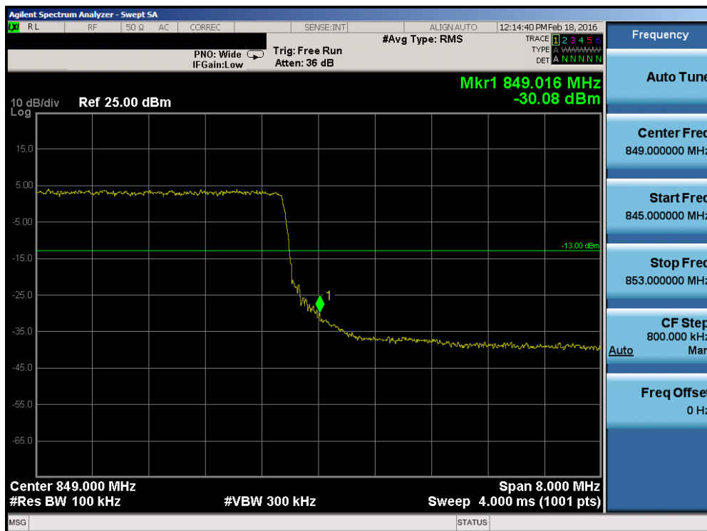
Plot 7-42. Upper Band Edge Plot (Band 5 – 10.0MHz QPSK – RB Size 50)
