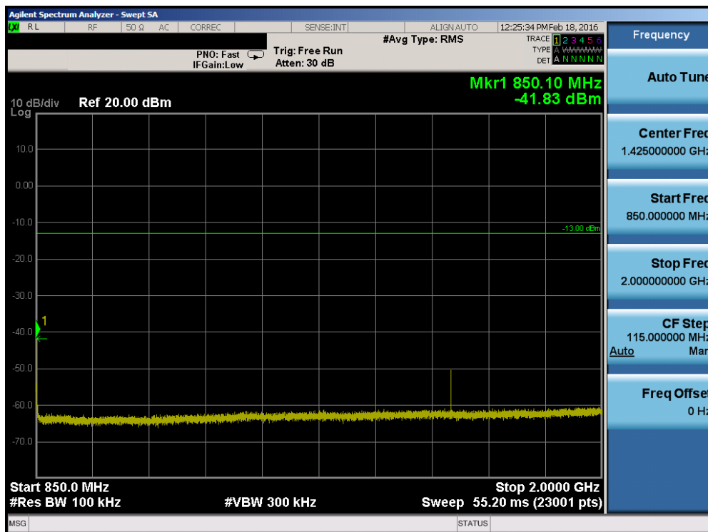
Plot 7-24. Conducted Spurious Plot (Band 5 – 3.0MHz QPSK – RB Size 1, RB Offset 0 – High Channel)
