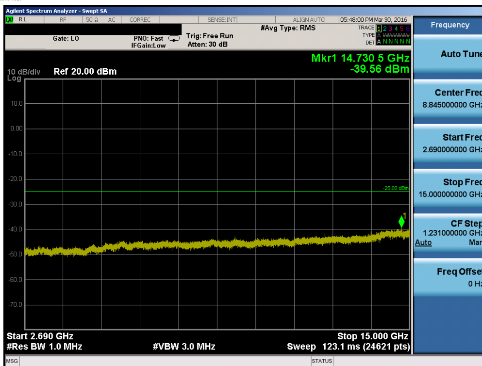
Plot 7-27. Conducted Spurious Plot (Band 41 – 10.0MHz QPSK – RB Size 1, RB Offset 0 – Low Channel)
