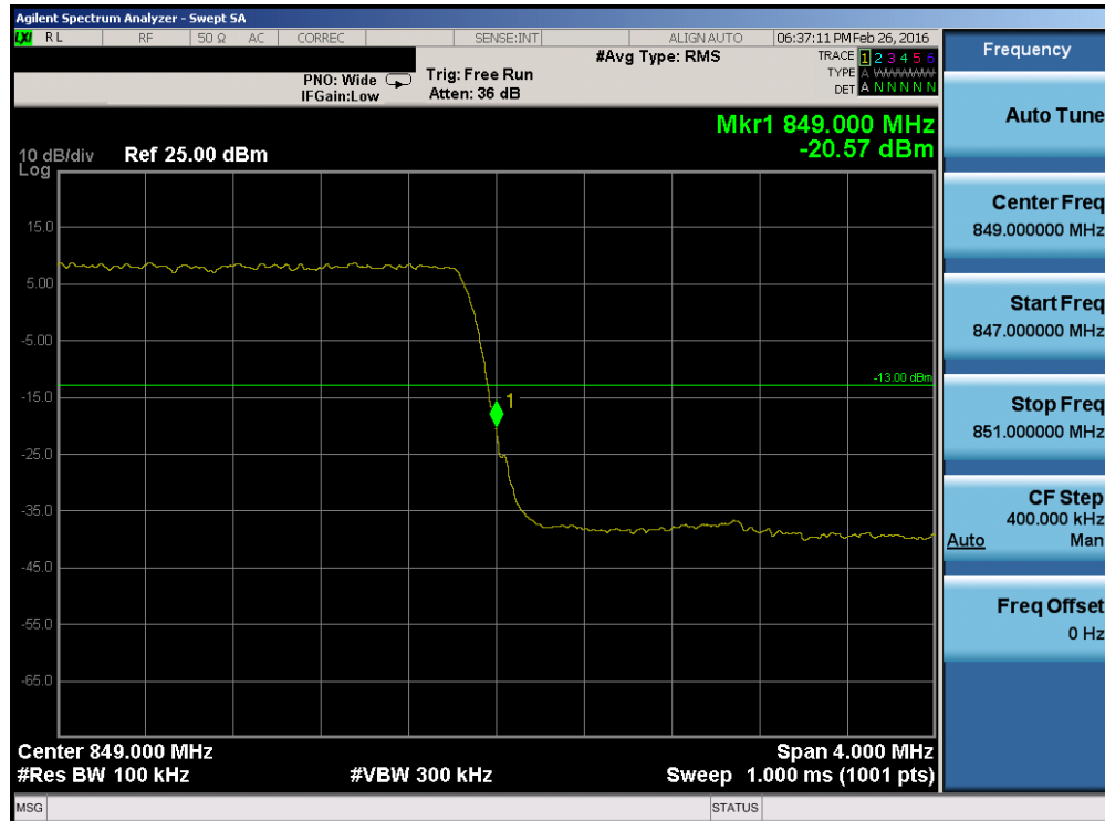
Plot 7-38. Upper Band Edge Plot (Band 5 – 3.0MHz QPSK – RB Size 15)
