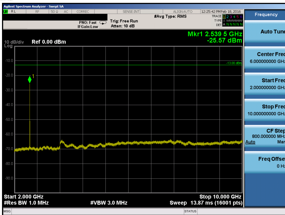
Plot 7-25. Conducted Spurious Plot (Band 5 – 3.0MHz QPSK – RB Size 1, RB Offset 0 – High Channel)
