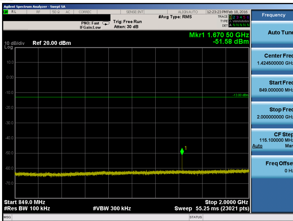
Plot 7-21. Conducted Spurious Plot (Band 5 – 3.0MHz QPSK – RB Size 1, RB Offset 0 – Mid Channel)
