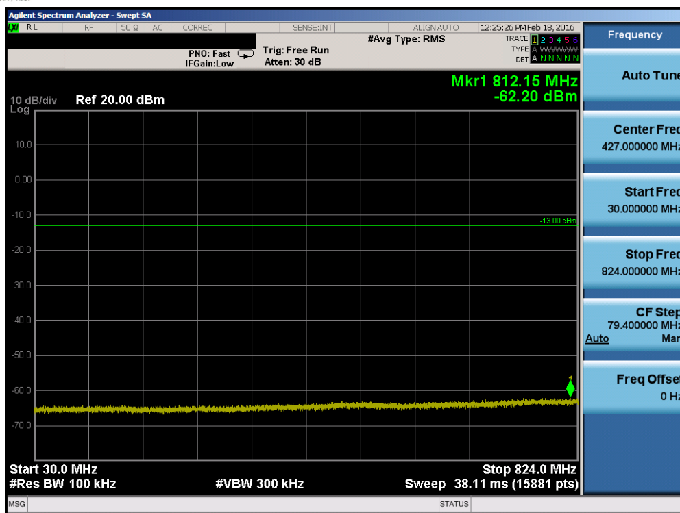
Plot 7-23. Conducted Spurious Plot (Band 5 – 3.0MHz QPSK – RB Size 1, RB Offset 0 – High Channel)
