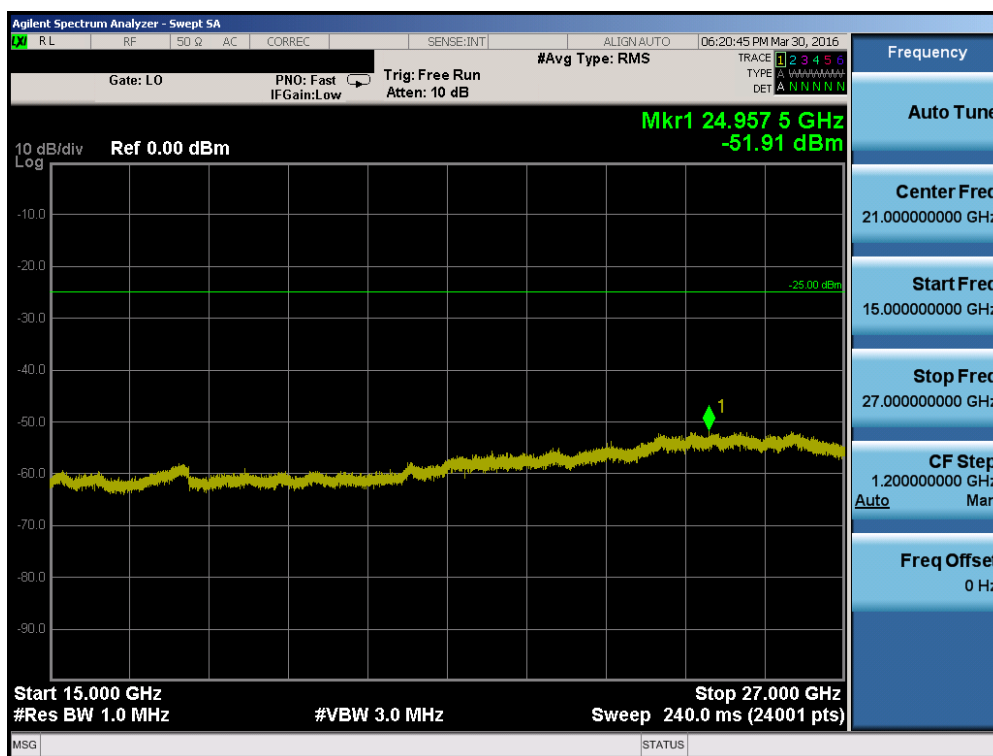
Plot 7-34. Conducted Spurious Plot (Band 41 – 10.0MHz QPSK – RB Size 1, RB Offset 0 – High Channel)
