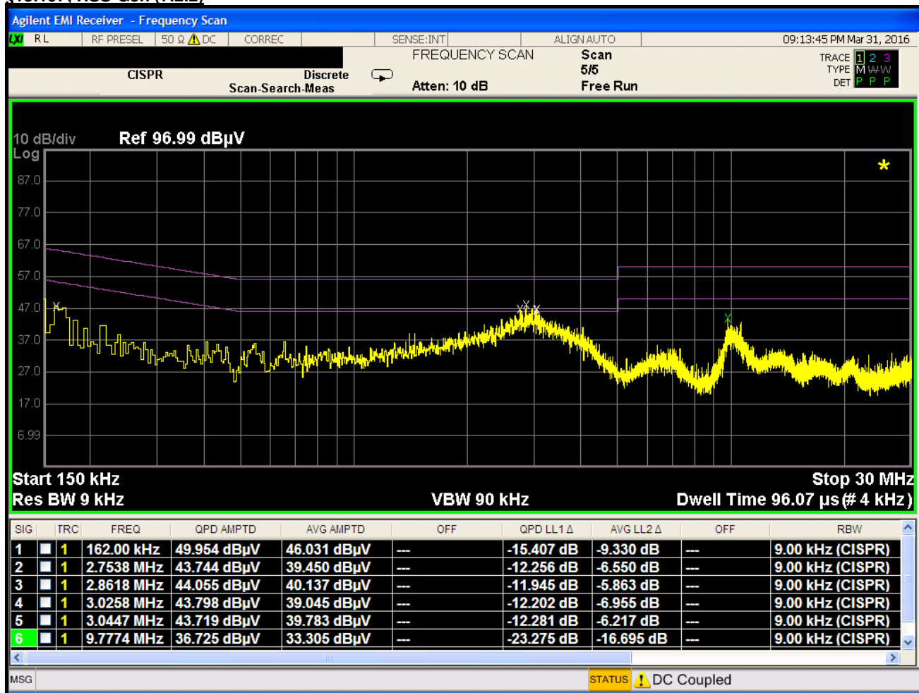
Plot 8-2. Line Conducted Plot (LN)
