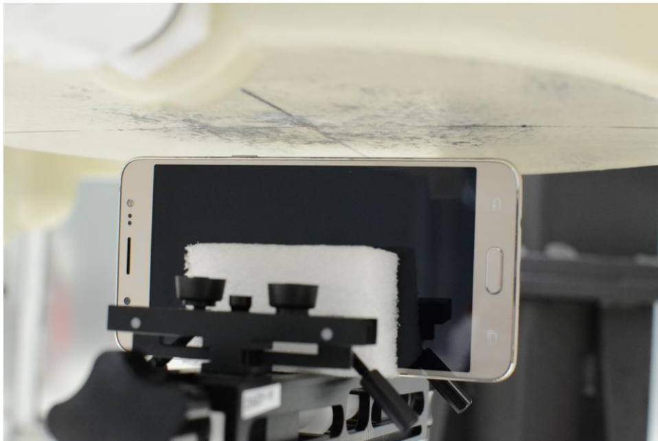
SAR Test Setup Photo 10: Right at 1.0 cm
