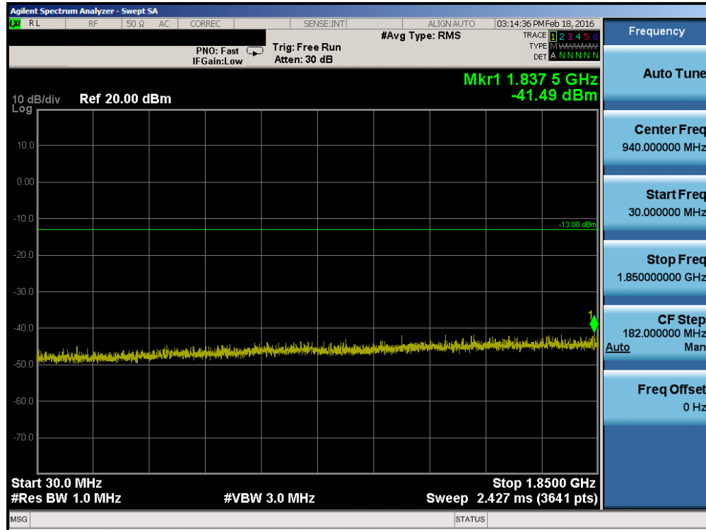
Plot 7-10. Conducted Spurious Plot (PCS GPRS Mode – Ch. 810)
