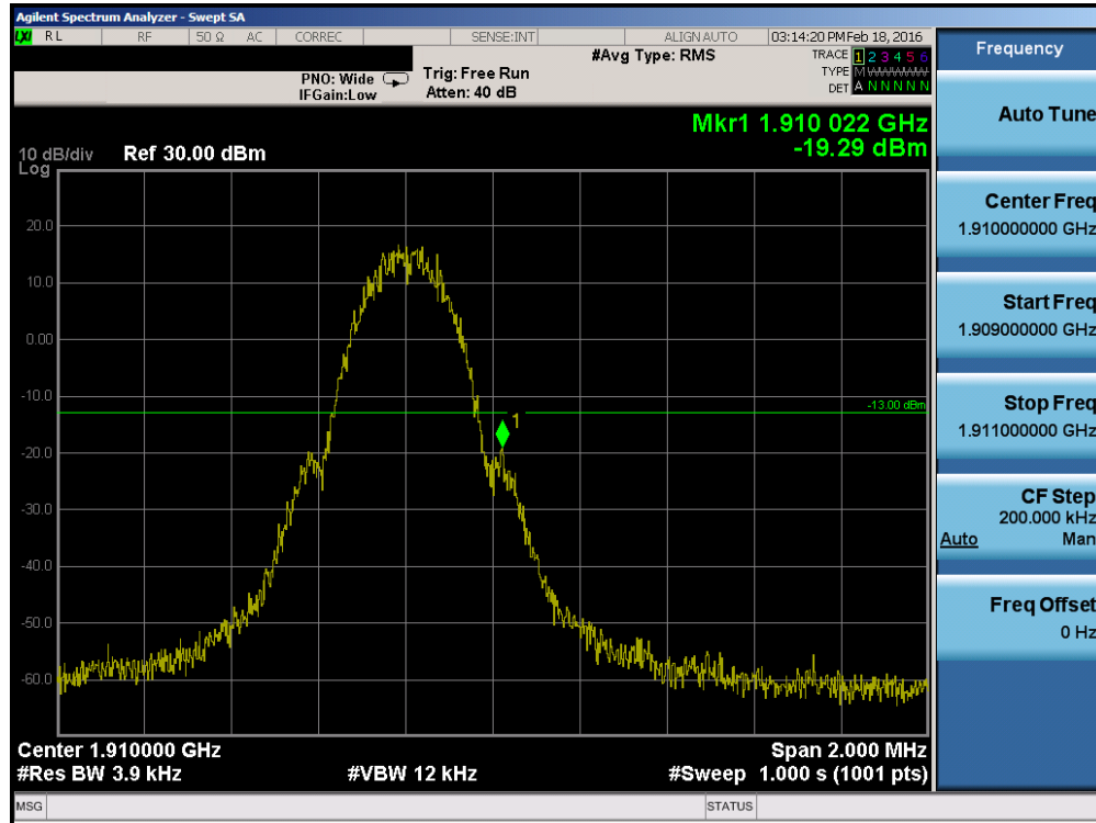
Plot 7-33. Band Edge Plot (PCS GPRS Mode – Ch. 810)
