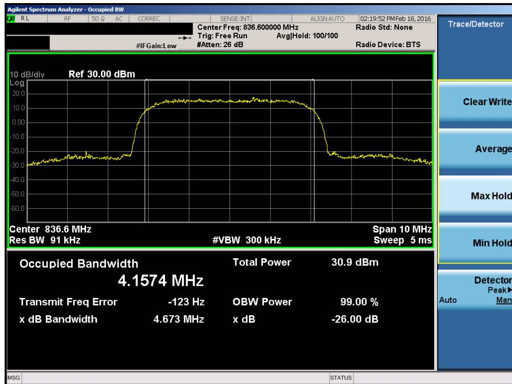
Plot 7-2. Occupied Bandwidth Plot (Cellular WCDMA Mode – Ch. 4183)
