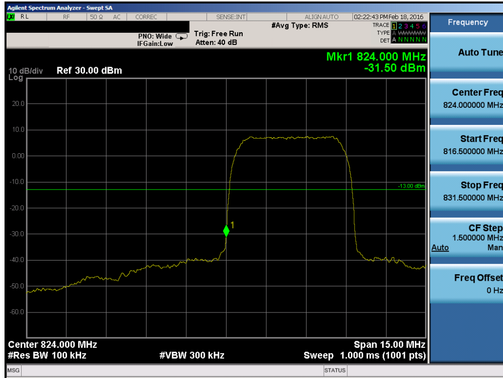
Plot 7-35. Band Edge Plot (Cellular WCDMA Mode – Ch. 4132)
