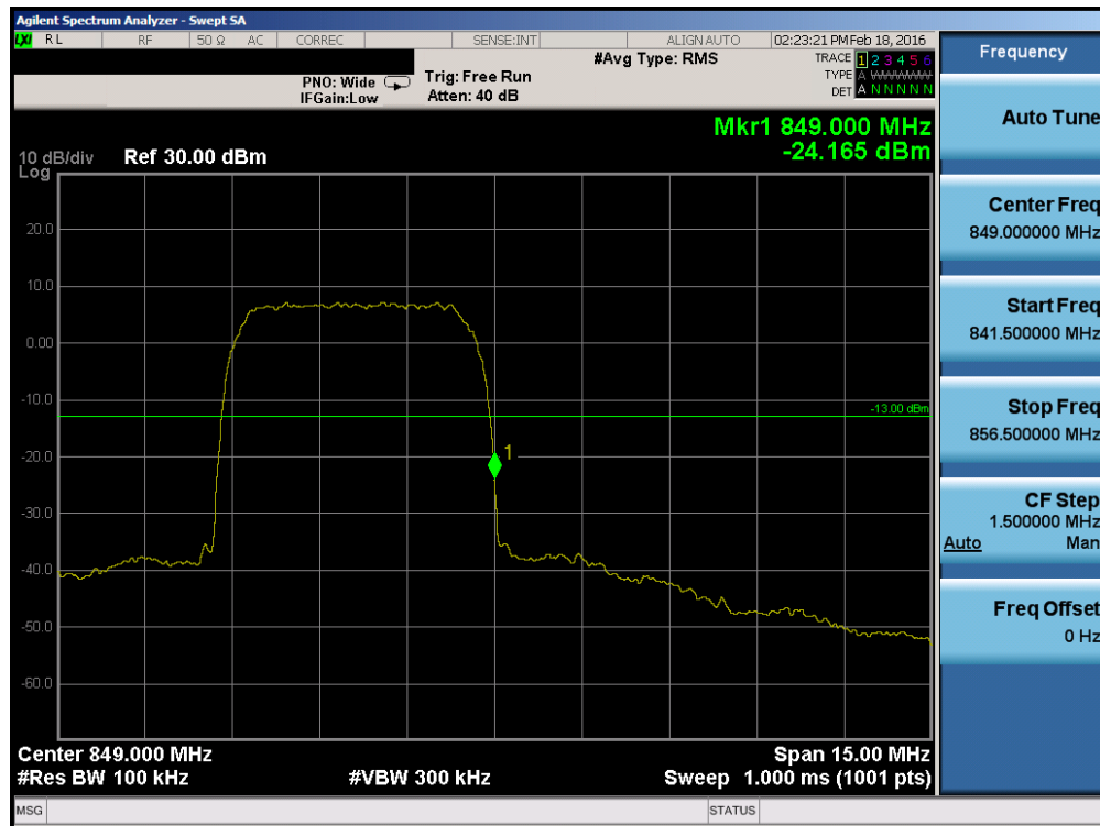
Plot 7-36. Band Edge Plot (Cellular WCDMA Mode – Ch. 4233)
