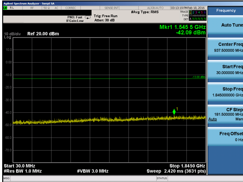
Plot 7-4. Conducted Spurious Plot (PCS GPRS Mode – Ch. 512)
