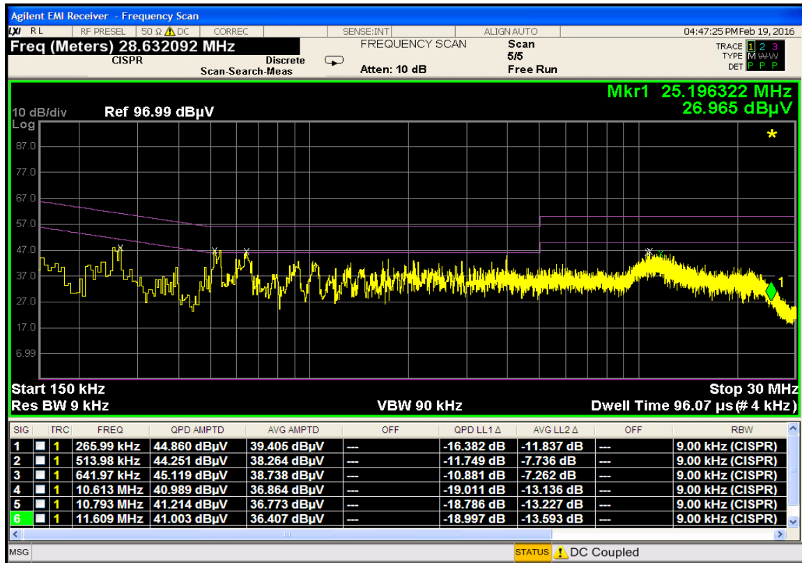
Plot 7-54. Line-Conducted Test Plot (L1)
