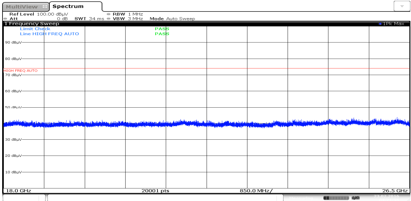
Plot 7-49. Radiated Spurious Plot above 18GHz (Pol. V)
