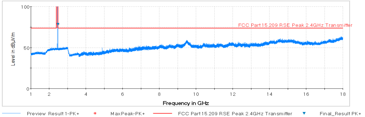
Plot 7-45. Radiated Spurious Plot above 1GHz (BT – Ch. 39, Ant. Pol. V)
