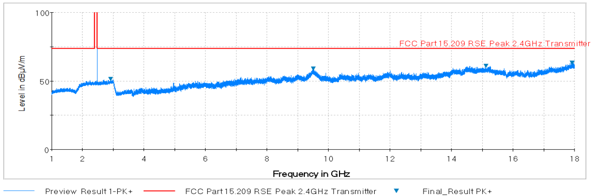
Plot 7-47. Radiated Spurious Plot above 1GHz (BT – Ch. 78, Ant. Pol. V)
