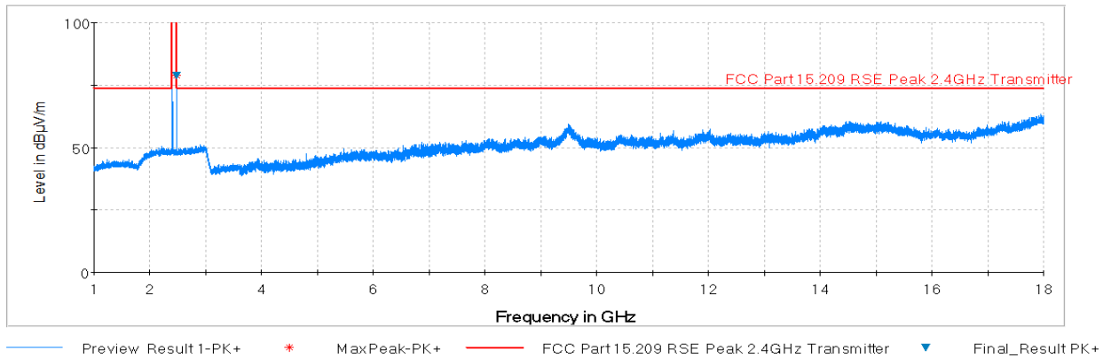
Plot 7-43. Radiated Spurious Plot above 1GHz (BT – Ch. 0, Ant. Pol. V)
