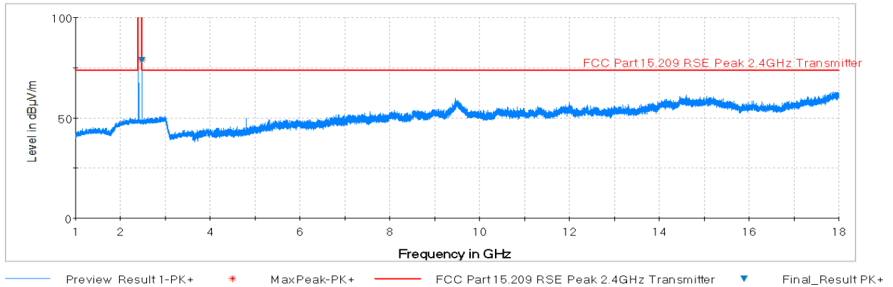
Plot 7-42. Radiated Spurious Plot above 1GHz (BT – Ch. 0, Ant. Pol. H)
