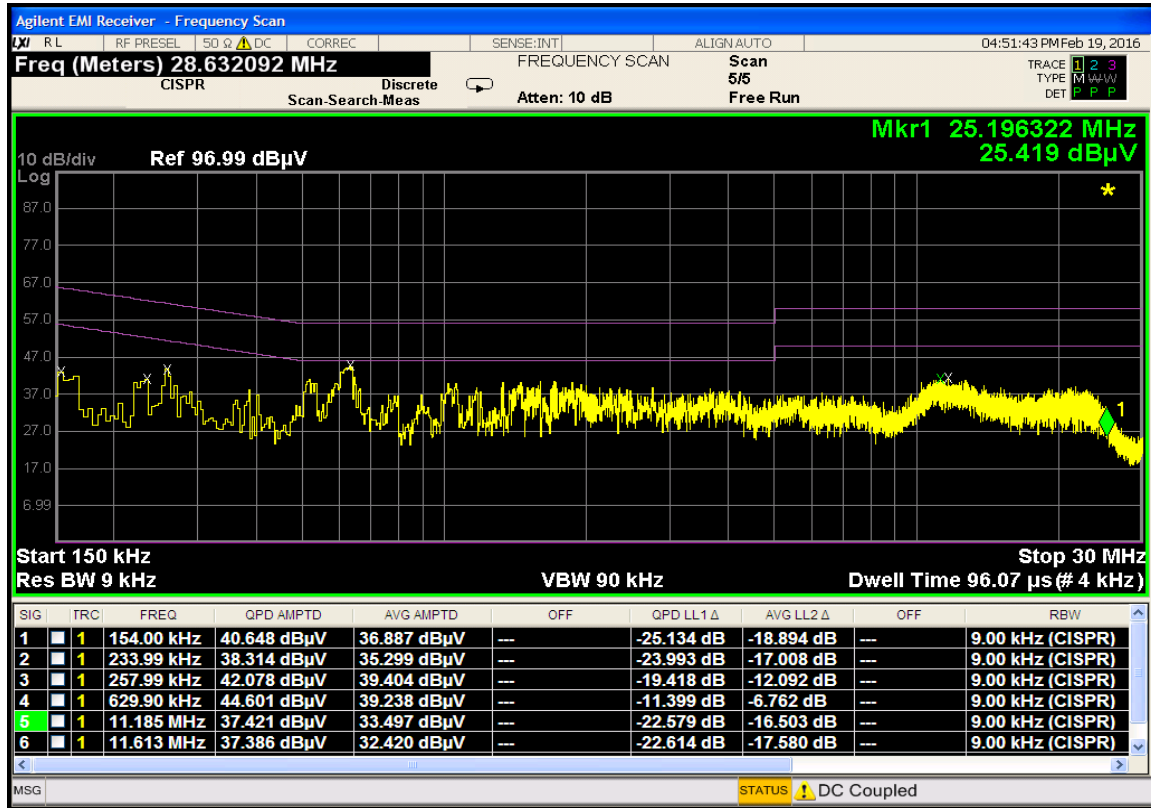
Plot 7-55. Line-Conducted Test Plot (N)
