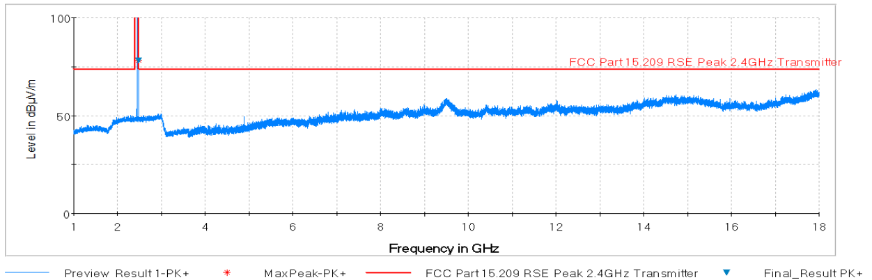
Plot 7-44. Radiated Spurious Plot above 1GHz (BT – Ch. 39, Ant. Pol. H)
