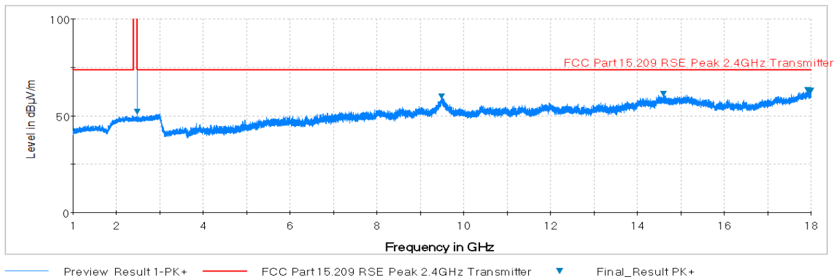
Plot 7-46. Radiated Spurious Plot above 1GHz (BT – Ch. 78, Ant. Pol. H)
