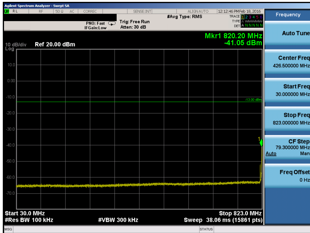
Plot 7-22. Conducted Spurious Plot (Band 5 – 10.0MHz QPSK – RB Size 1, RB Offset 0– Low Channel)
