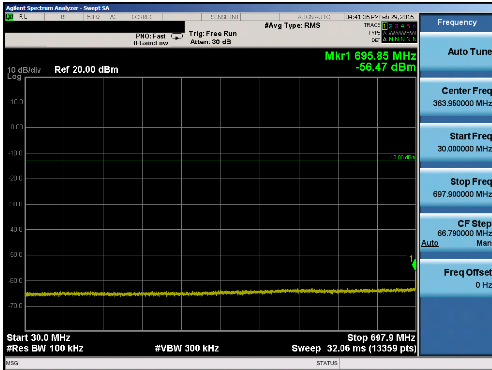
Plot 7-13. Conducted Spurious Plot (Band 17 – 10.0MHz QPSK – RB Size 1, RB Offset 0– Low Channel)
