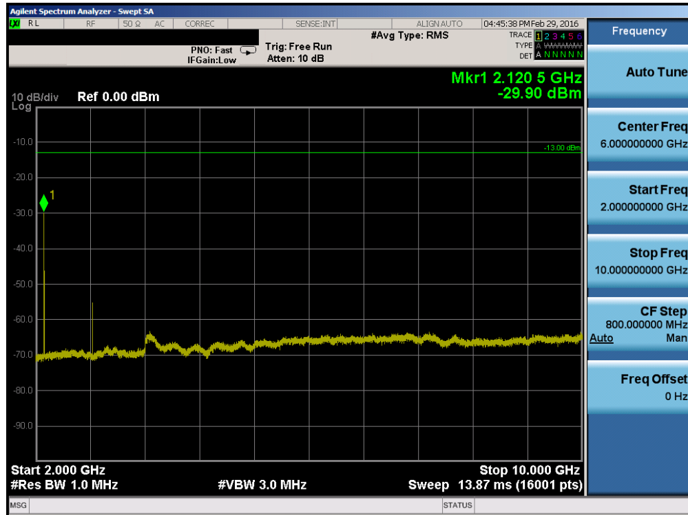
Plot 7-21. Conducted Spurious Plot (Band 17 – 10.0MHz QPSK – RB Size 1, RB Offset 0 – High Channel)
