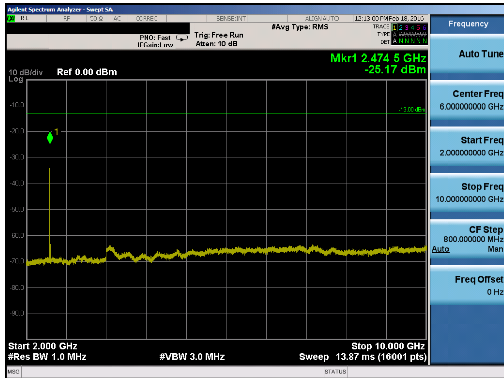
Plot 7-24. Conducted Spurious Plot (Band 5 – 10.0MHz QPSK – RB Size 1, RB Offset 0 – Low Channel)
