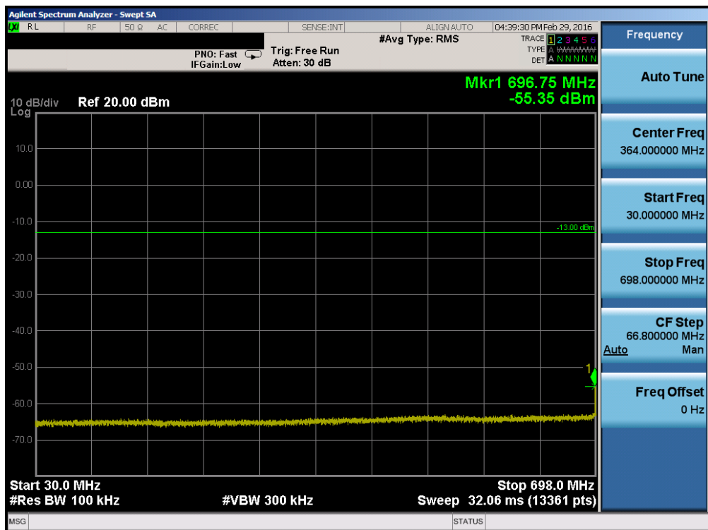
Plot 7-16. Conducted Spurious Plot (Band 17 – 10.0MHz QPSK – RB Size 1, RB Offset 0 – Mid Channel)
