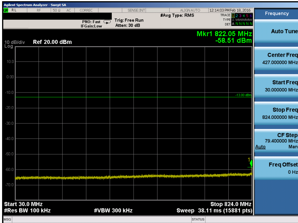
Plot 7-28. Conducted Spurious Plot (Band 5 – 10.0MHz QPSK – RB Size 1, RB Offset 0 – High Channel)
