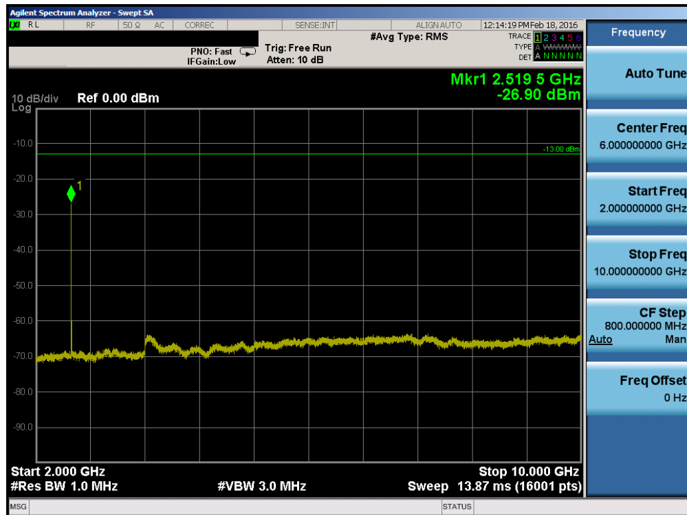
Plot 7-30. Conducted Spurious Plot (Band 5 – 10.0MHz QPSK – RB Size 1, RB Offset 0 – High Channel)
