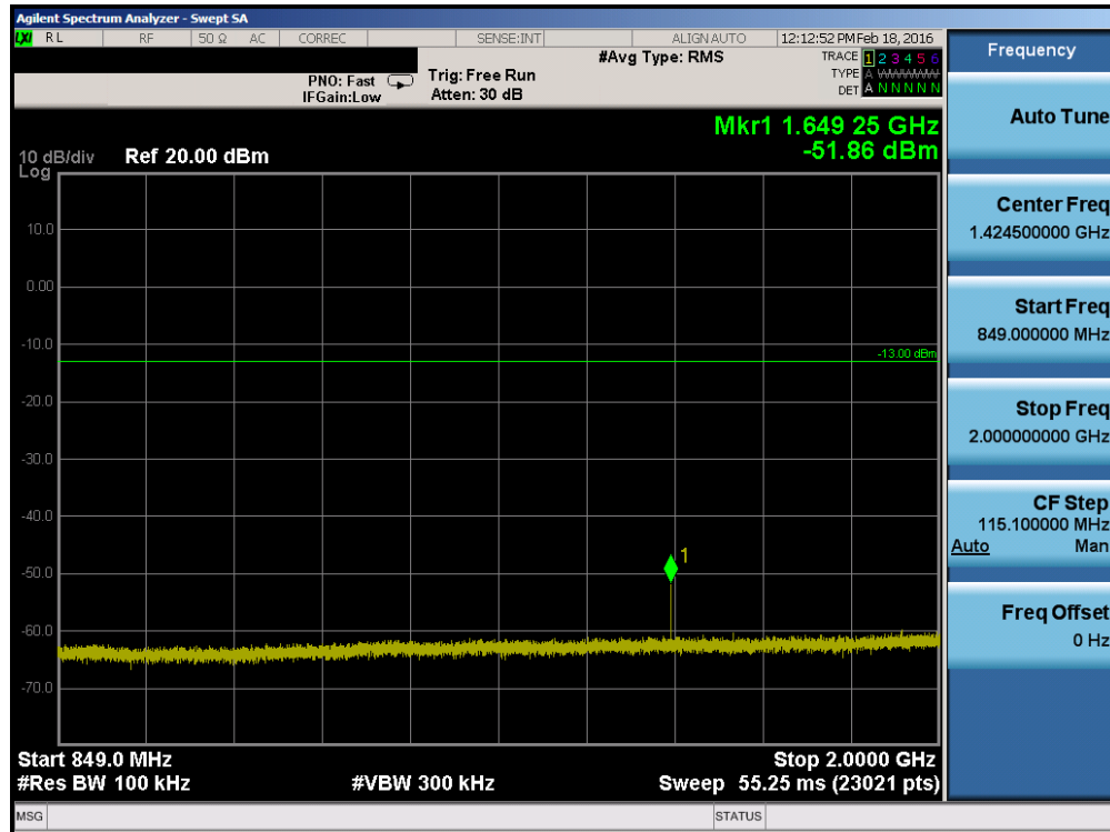
Plot 7-23. Conducted Spurious Plot (Band 5 – 10.0MHz QPSK – RB Size 1, RB Offset 0 – Low Channel)
