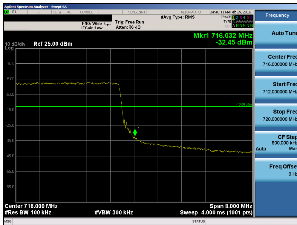
Plot 7-34. Upper Band Edge Plot (Band 17 – 10.0MHz QPSK – RB Size 50)
