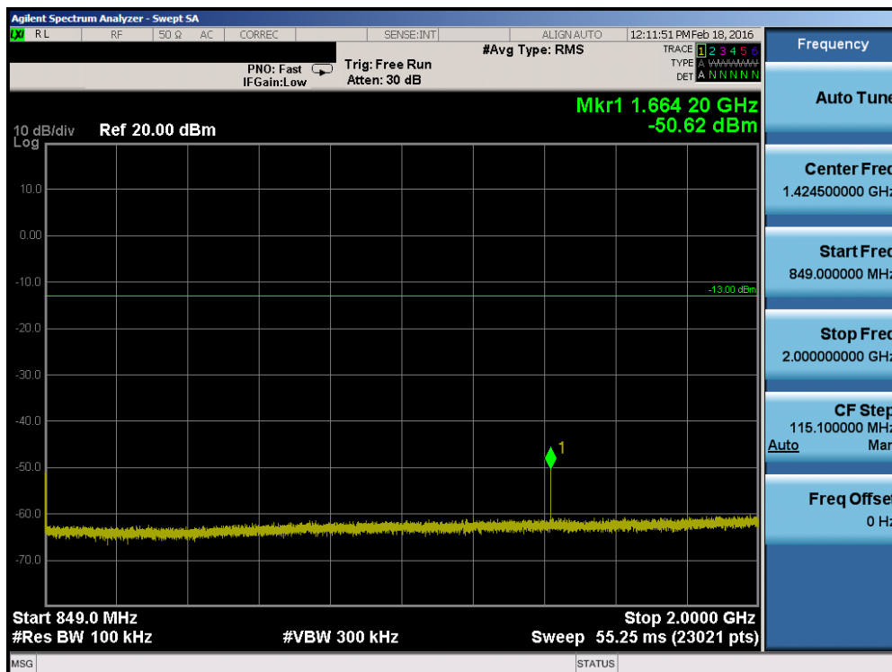
Plot 7-26. Conducted Spurious Plot (Band 5 – 10.0MHz QPSK – RB Size 1, RB Offset 0 – Mid Channel)
