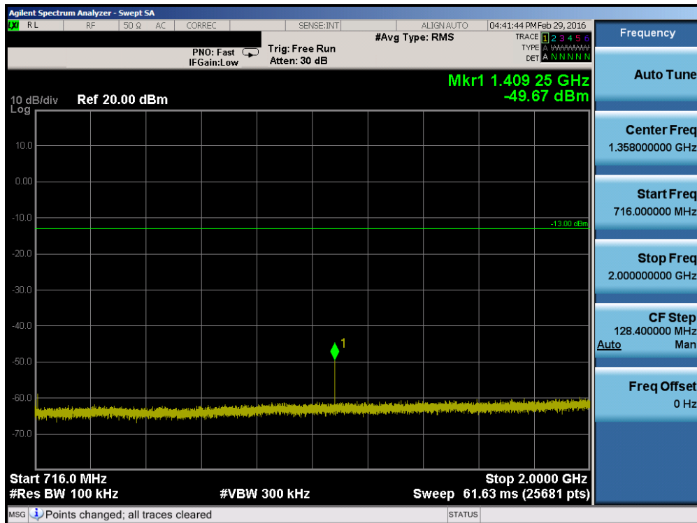
Plot 7-14. Conducted Spurious Plot (Band 17 – 10.0MHz QPSK – RB Size 1, RB Offset 0 – Low Channel)
