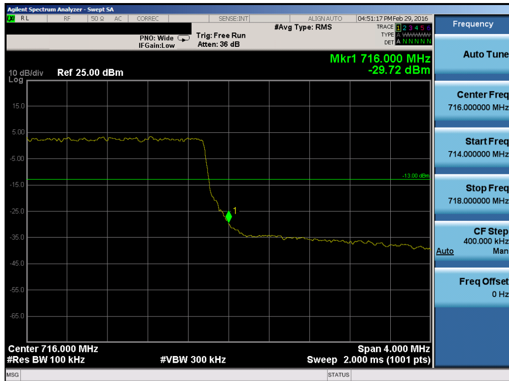
Plot 7-32. Upper Band Edge Plot (Band 17 – 5.0MHz QPSK – RB Size 25)
