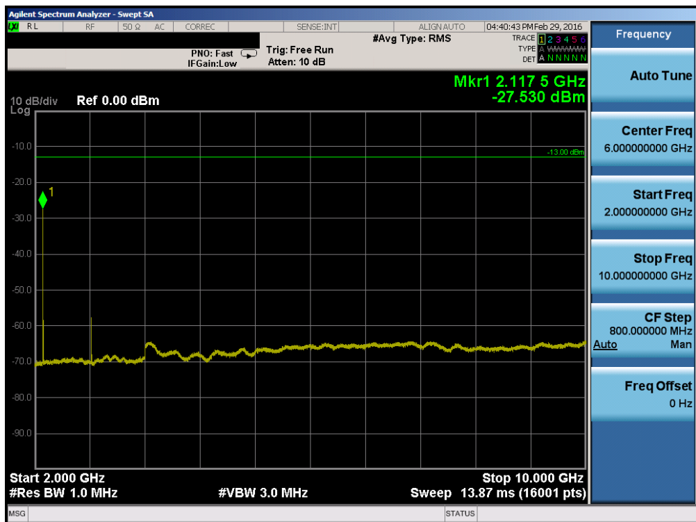
Plot 7-18. Conducted Spurious Plot (Band 17 – 10.0MHz QPSK – RB Size 1, RB Offset 0 – Mid Channel)
