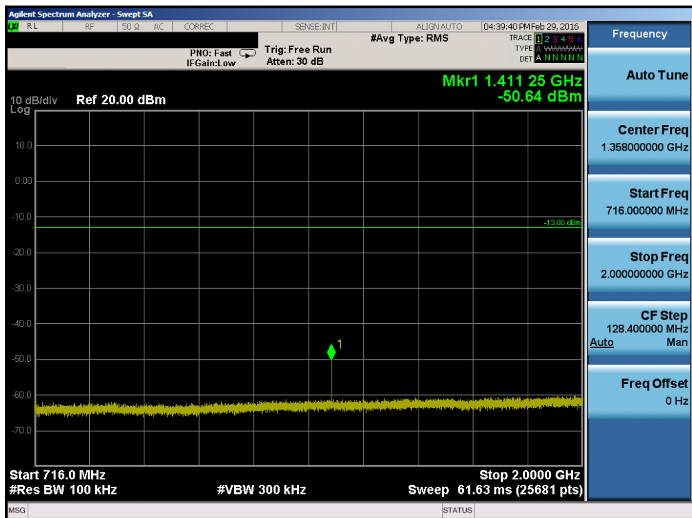
Plot 7-17. Conducted Spurious Plot (Band 17 – 10.0MHz QPSK – RB Size 1, RB Offset 0 – Mid Channel)
