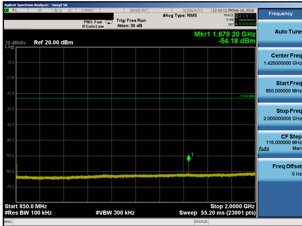
Plot 7-29. Conducted Spurious Plot (Band 5 – 10.0MHz QPSK – RB Size 1, RB Offset 0 – High Channel)
