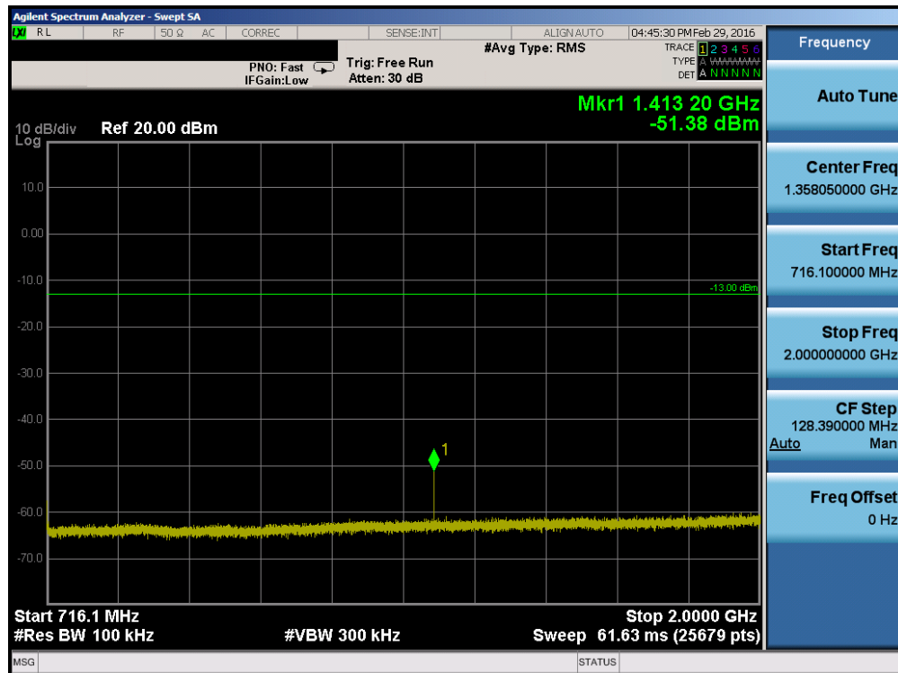
Plot 7-20. Conducted Spurious Plot (Band 17 – 10.0MHz QPSK – RB Size 1, RB Offset 0 – High Channel)
