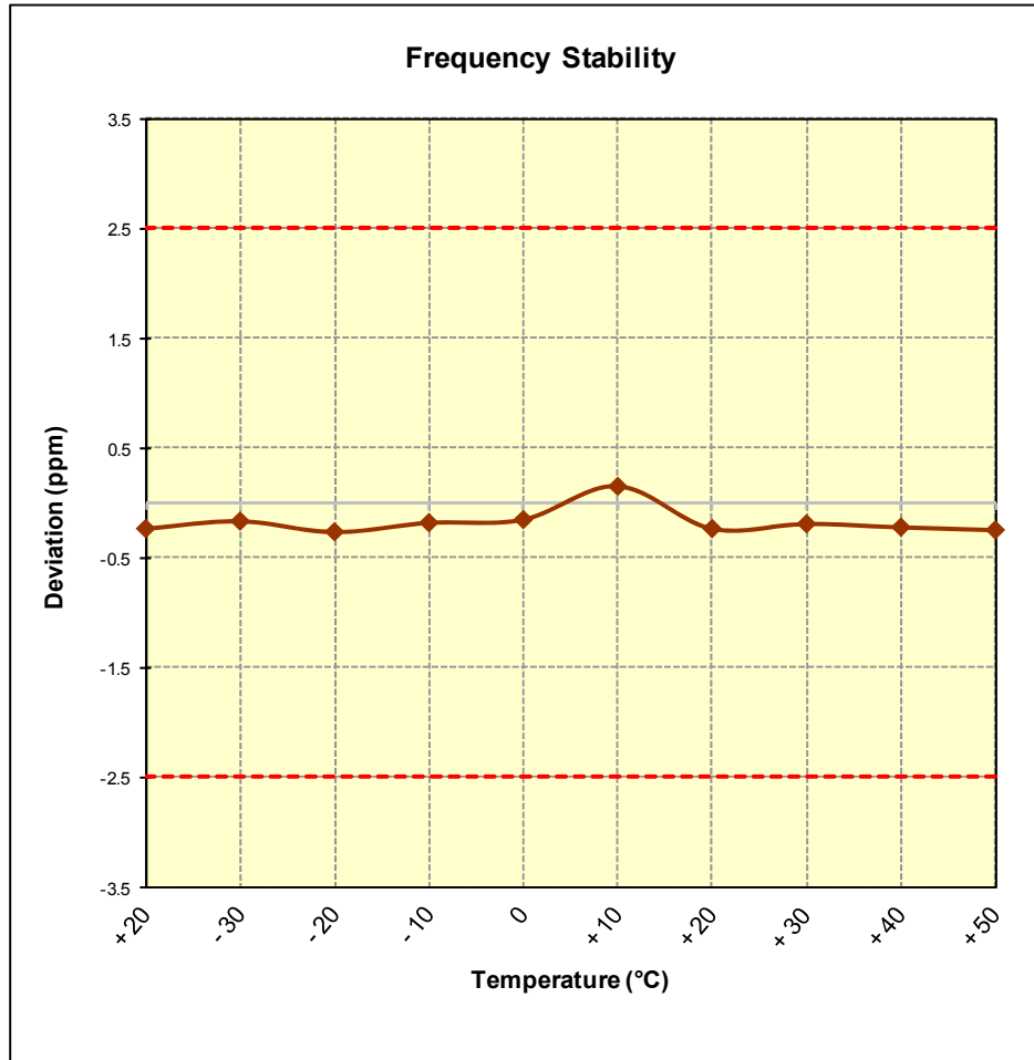
Figure 7-7. Frequency Stability Graph (Band 17)
