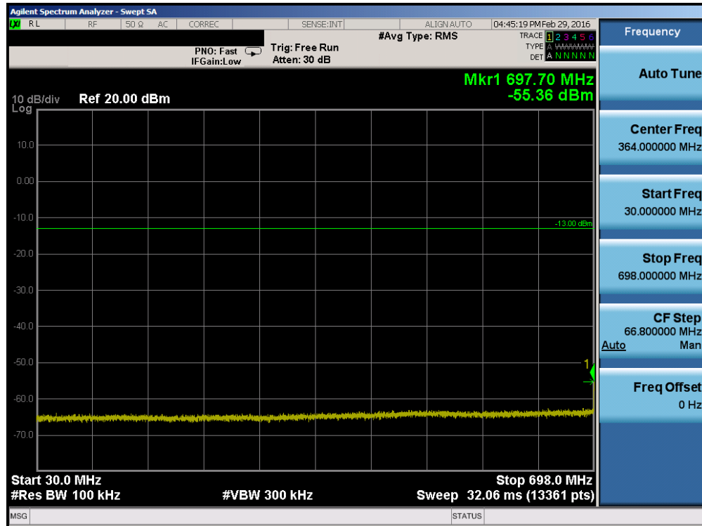
Plot 7-19. Conducted Spurious Plot (Band 17 – 10.0MHz QPSK – RB Size 1, RB Offset 0 – High Channel)
