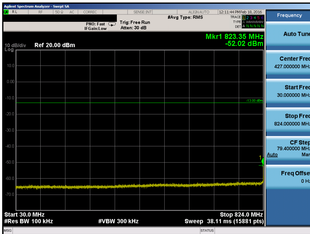
Plot 7-25. Conducted Spurious Plot (Band 5 – 10.0MHz QPSK – RB Size 1, RB Offset 0 – Mid Channel)
