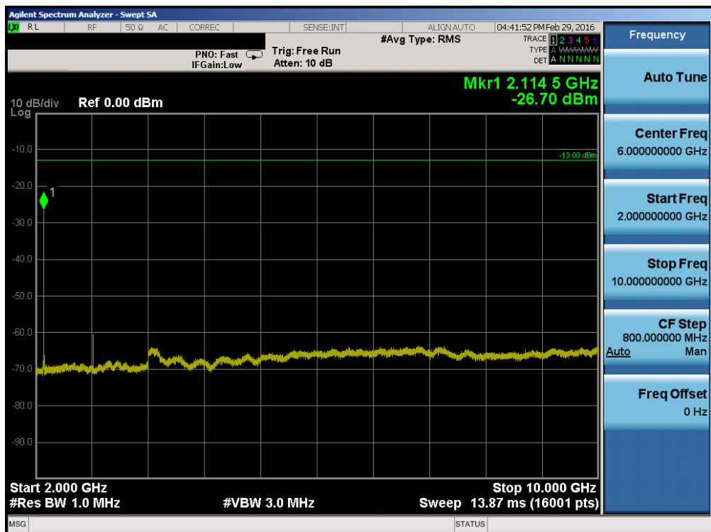
Plot 7-15. Conducted Spurious Plot (Band 17 – 10.0MHz QPSK – RB Size 1, RB Offset 0 – Low Channel)
