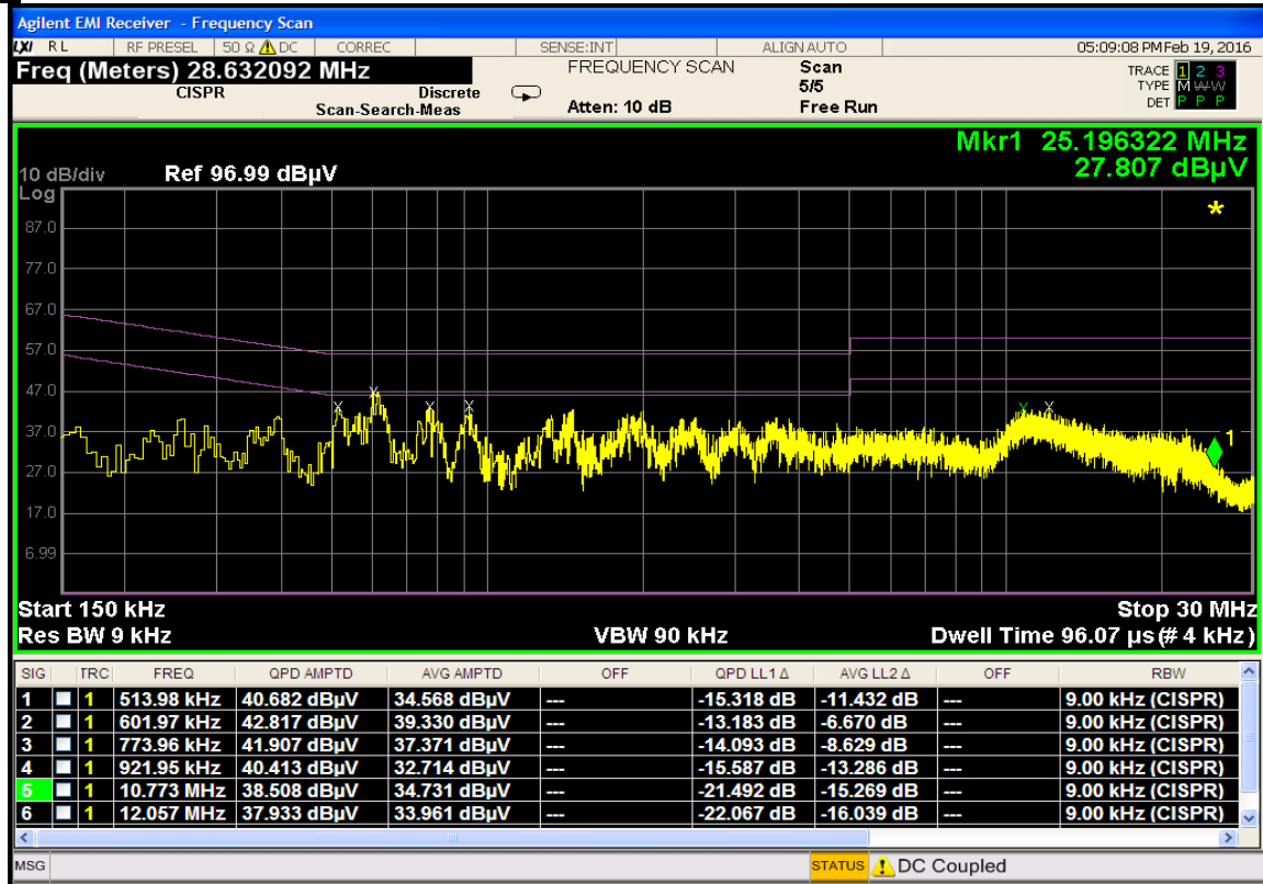
Plot 7-48. Line Conducted Plot with 802.11b (N)
