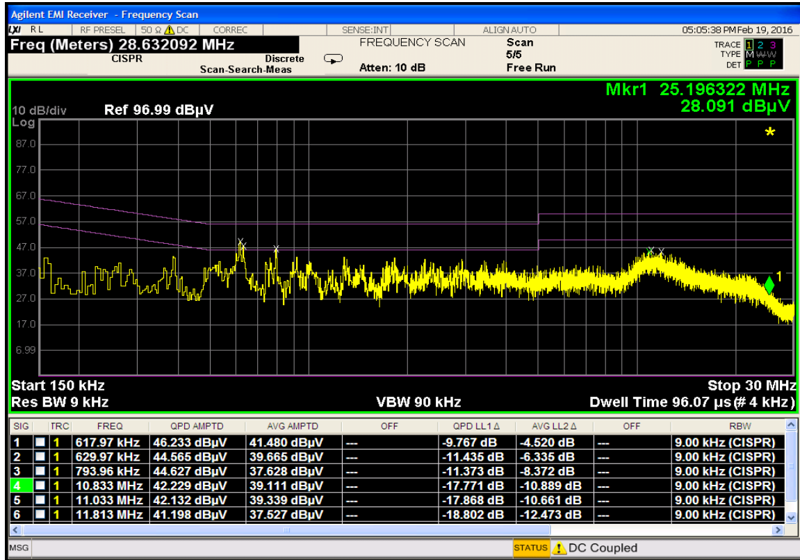
Plot 7-47. Line Conducted Plot with 802.11b (L1)
