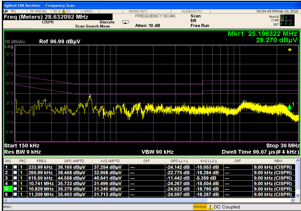
Plot 7-21. Line Conducted Plot with Bluetooth LE (N)
