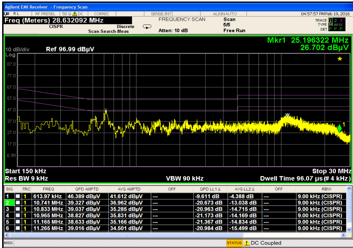
Plot 7-20. Line Conducted Plot with Bluetooth LE (L1)
