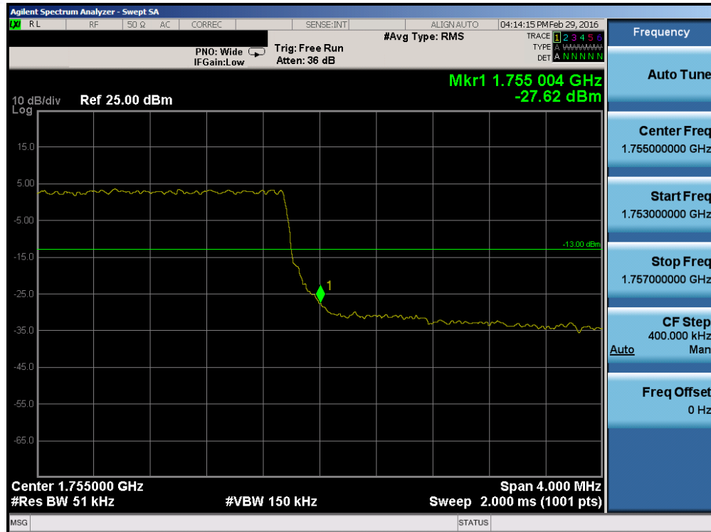
Plot 7-95. Upper Band Edge Plot (Band 4 – 5.0MHz QPSK – RB Size 25)
