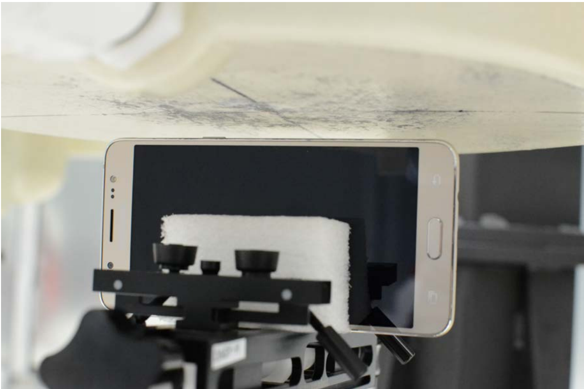
SAR Test Setup Photo 10: Right at 1.0 cm
