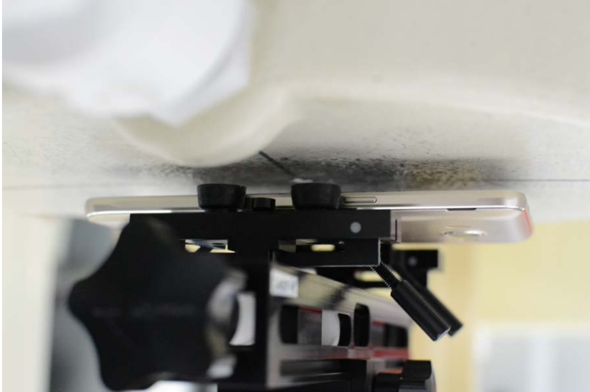
SAR Test Setup Photo 7: Front at 1.0 cm
