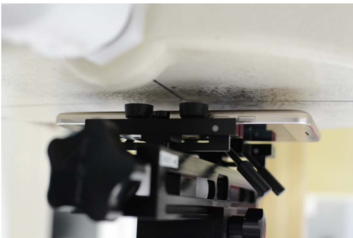
SAR Test Setup Photo 6: Back at 1.0 cm
