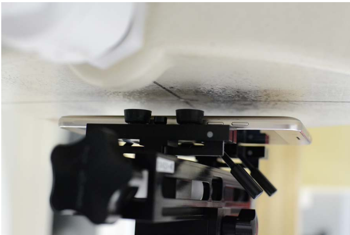
SAR Test Setup Photo 5: Back at 1.5 cm
