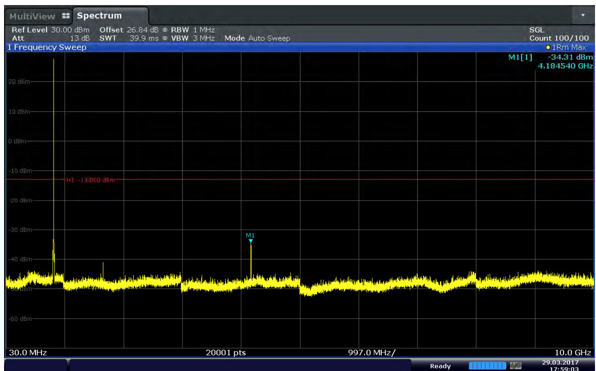
Plot 6-10. Conducted Spurious Plot (Band 5–1.4MHz–QPSK–RB Size 1–RB Offset 5–Ch.20525)
