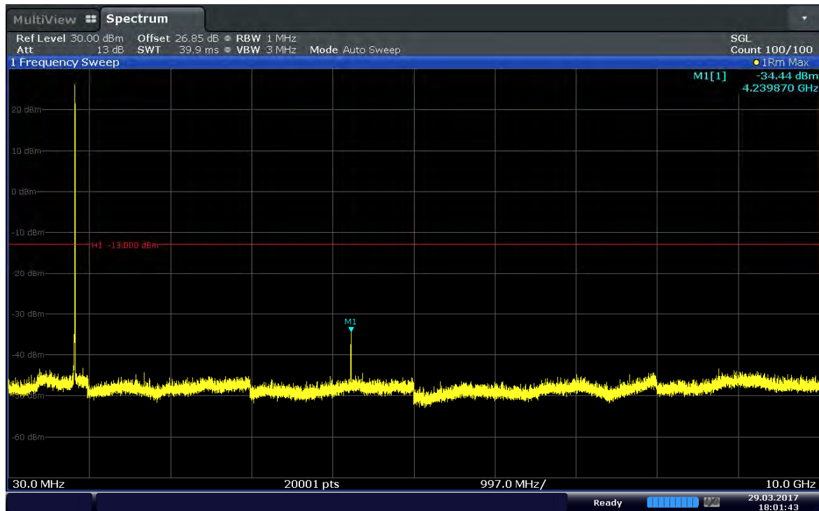
Plot 6-11. Conducted Spurious Plot (Band 5–1.4MHz–QPSK–RB Size 3–RB Offset 0– Ch.20643)
