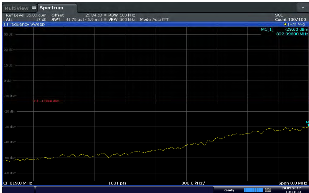
Plot 6-30. Extended Lower Band Edge Plot (Band 5 – 5.0MHz – QPSK – RB Size 25)
