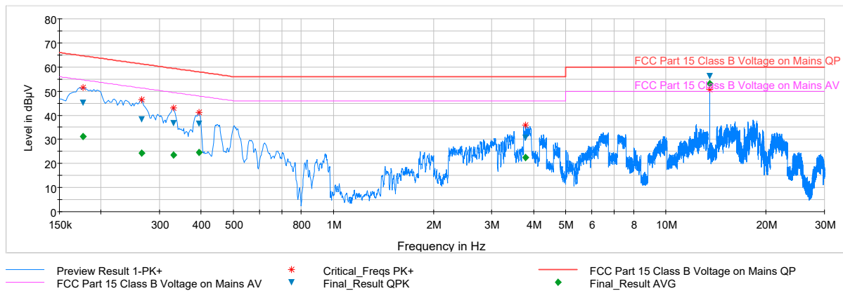
Plot 7-2. Line-Conducted Test Plot With Antenna Connected(N)
