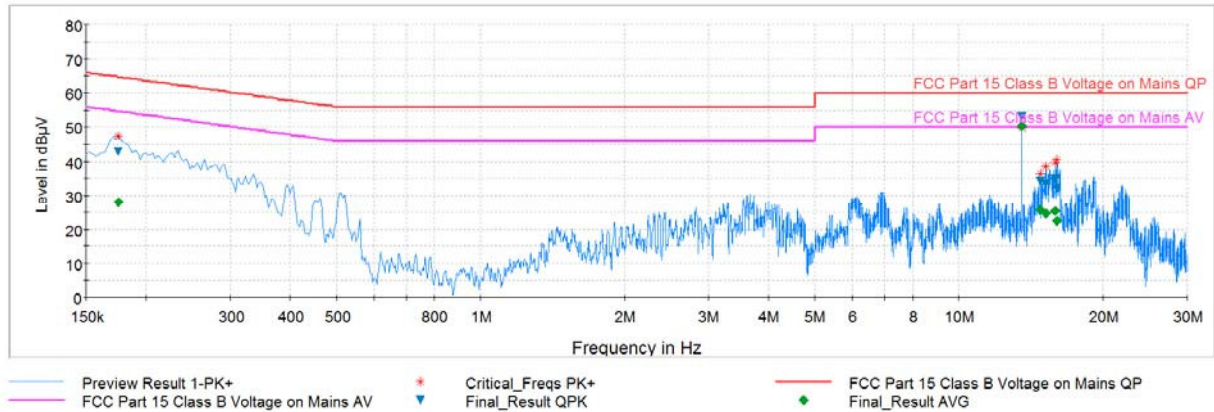
Plot 7-1. Line-Conducted Test Plot With Antenna Connected(L1)
