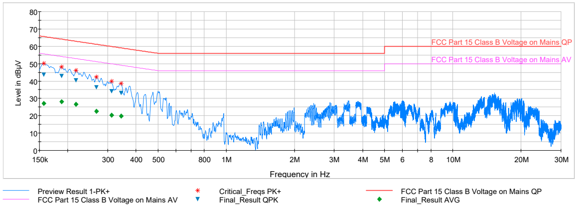
Plot 7-4. Line-Conducted Test Plot With Antenna Terminated in 50 Ω (N)
