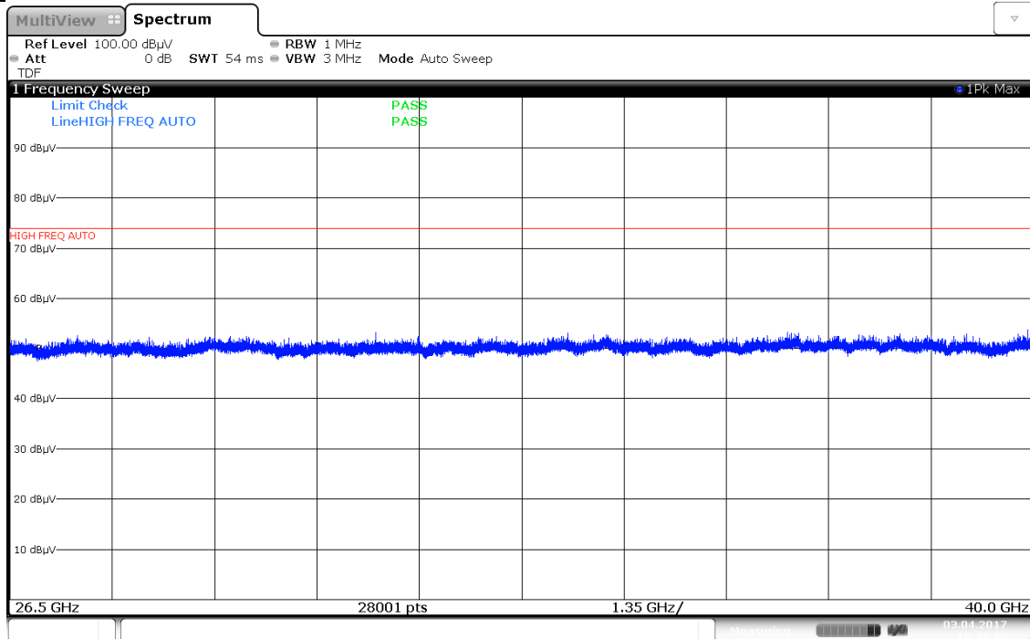
Plot 7-89. Radiated Spurious Plot 26.5GHz - 40GHz (802.11a – Ant. Pol. H)
