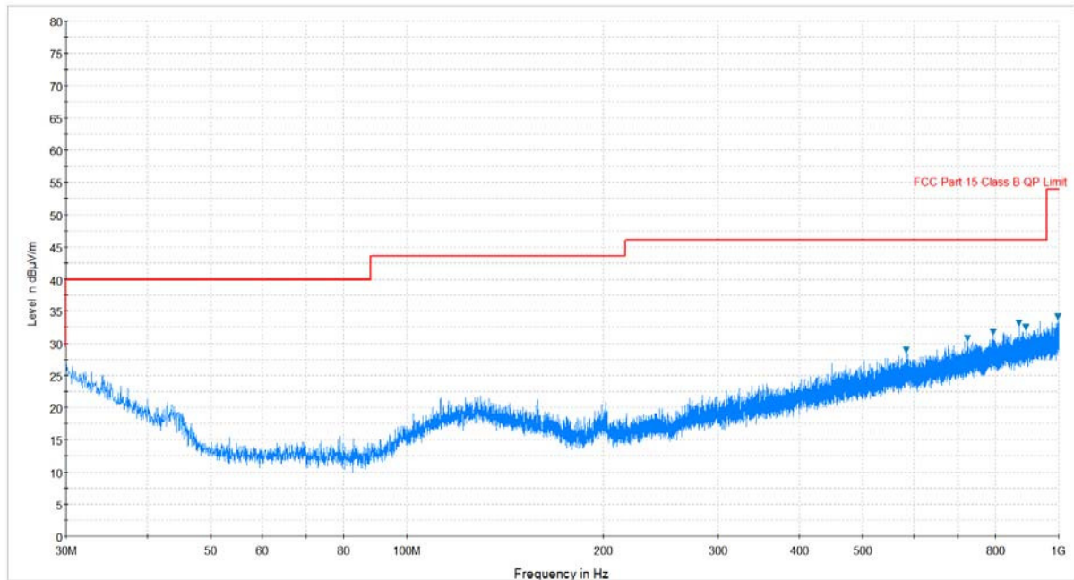
Plot 7-112. Radiated Spurious Plot below 1GHz (802.11a – U3 Ch. 157, Ant. Pol. H)
