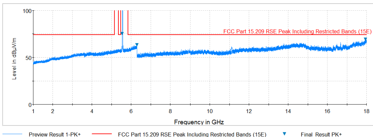
Plot 7-84. Radiated Spurious Plot above 1GHz (802.11a – U2C Ch. 120, Ant. Pol. V)
