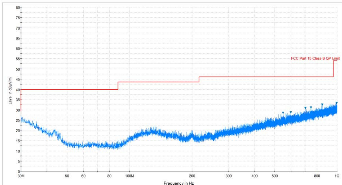
Plot 7-113. Radiated Spurious Plot below 1GHz (802.11a – U3 Ch. 157, Ant. Pol. V)
