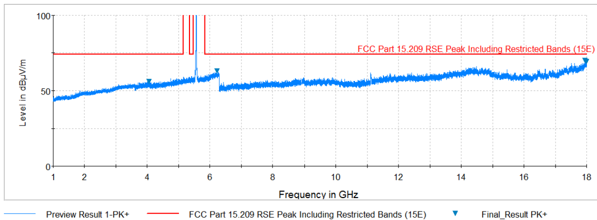
Plot 7-83. Radiated Spurious Plot above 1GHz (802.11a – U2C Ch. 120, Ant. Pol. H)
