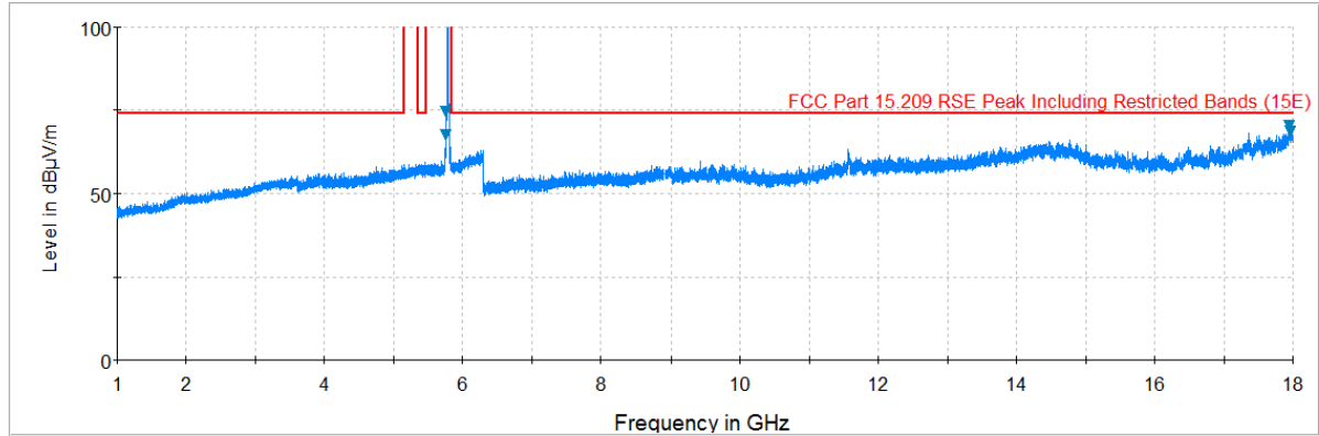
Plot 7-85. Radiated Spurious Plot above 1GHz (802.11a – U3 Ch. 157, Ant. Pol. H)
