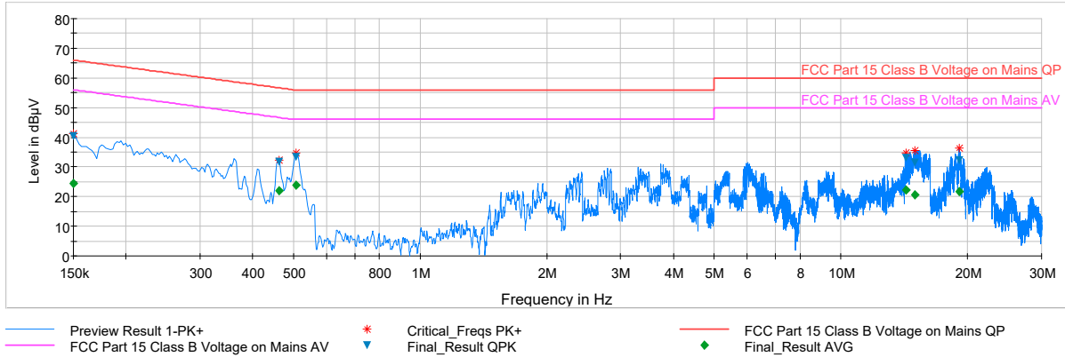
Plot 8-3. Line-Conducted Test Plot with Antenna Terminated in 50Ω (L1)
