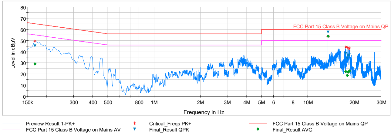
Plot 8-1. Line-Conducted Test Plot with Antenna Connected (L1)
