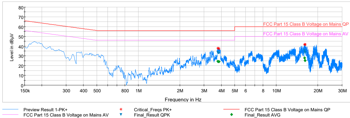
Plot 8-4. Line-Conducted Test Plot with Antenna Terminated in 50Ω (N)
