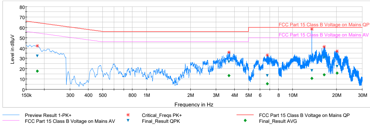
Plot 8-2. Line-Conducted Test Plot with Antenna Connected (N)
