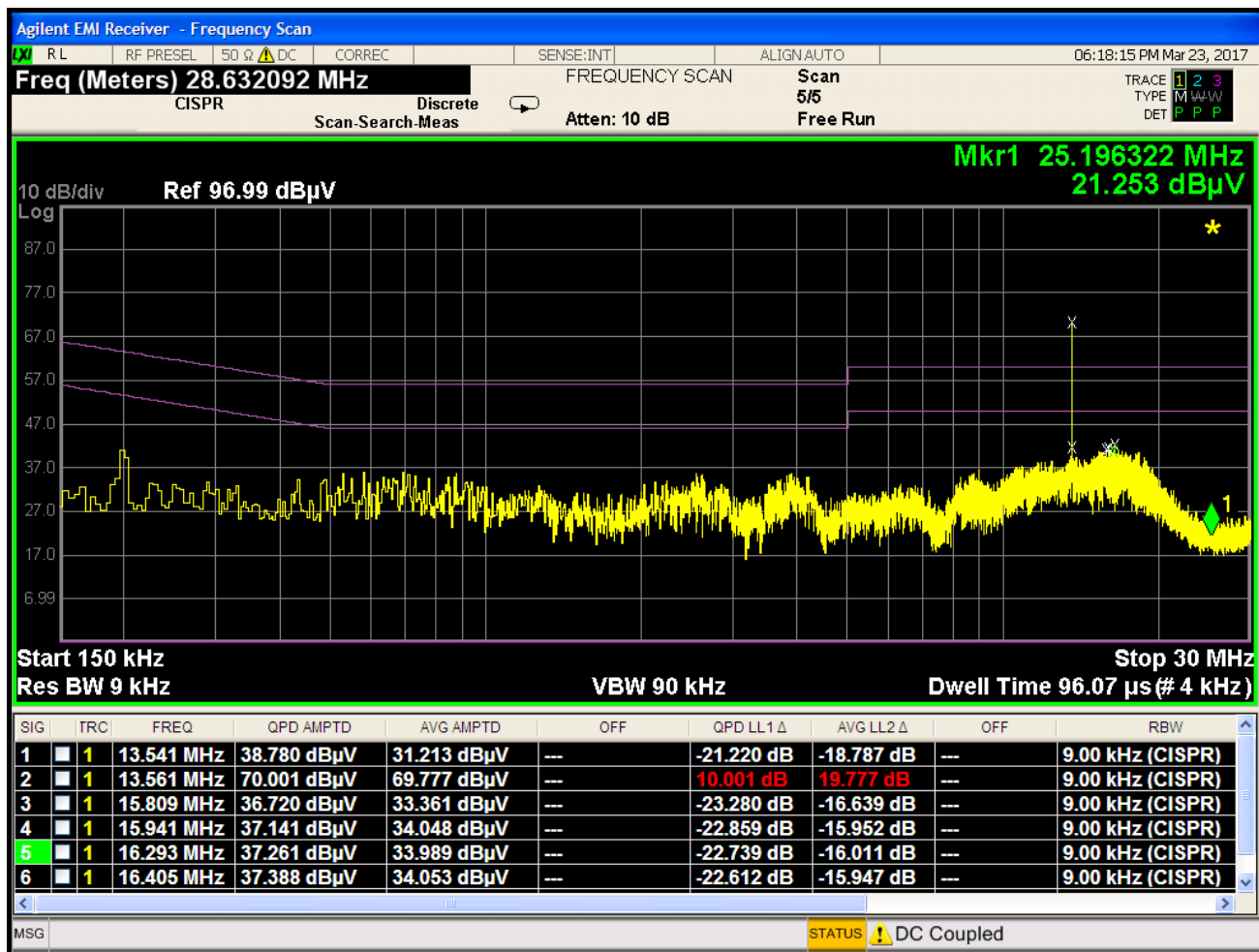
Plot 8-2. Line-Conducted Test Plot with Antenna Attached(N)
