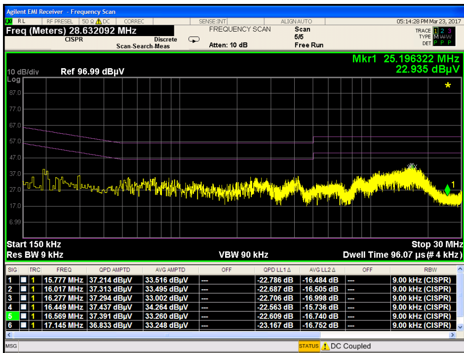
Plot 7-115. Line Conducted Plot with 802.11a UNII Band 1 (N)
