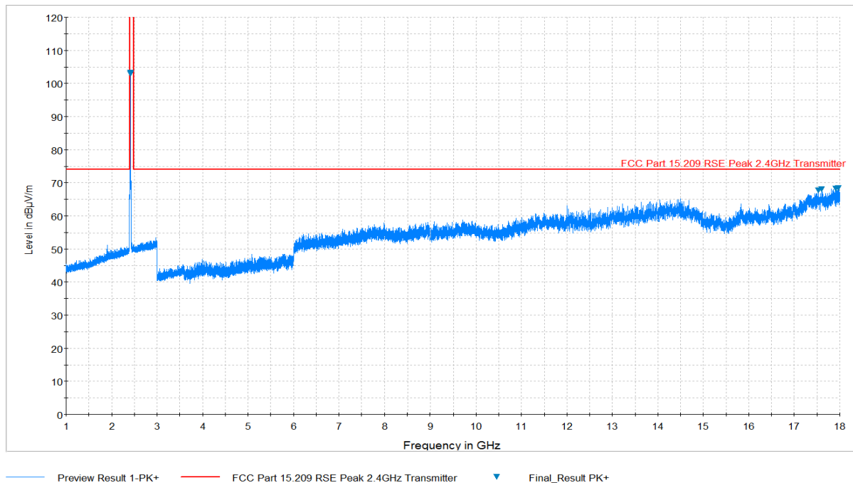
Plot 7-31. Radiated Spurious Plot above 1GHz (802.11b – Ch. 1, Ant. Pol. H)
