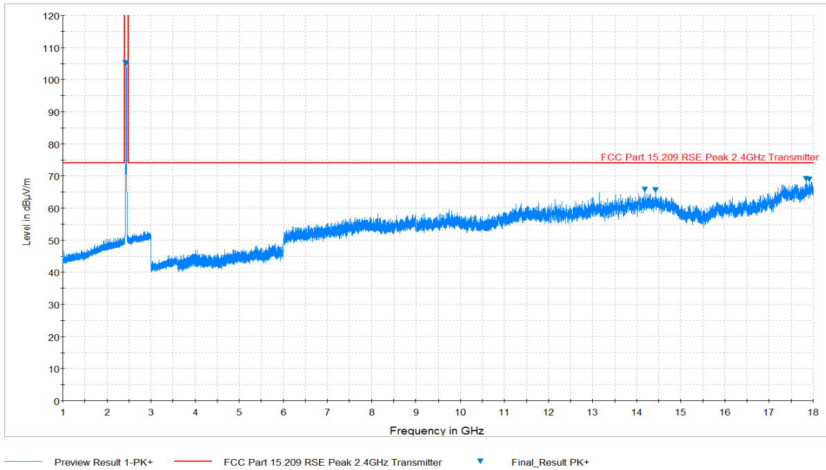
Plot 7-33. Radiated Spurious Plot above 1GHz (802.11b – Ch. 6, Ant. Pol. H)
