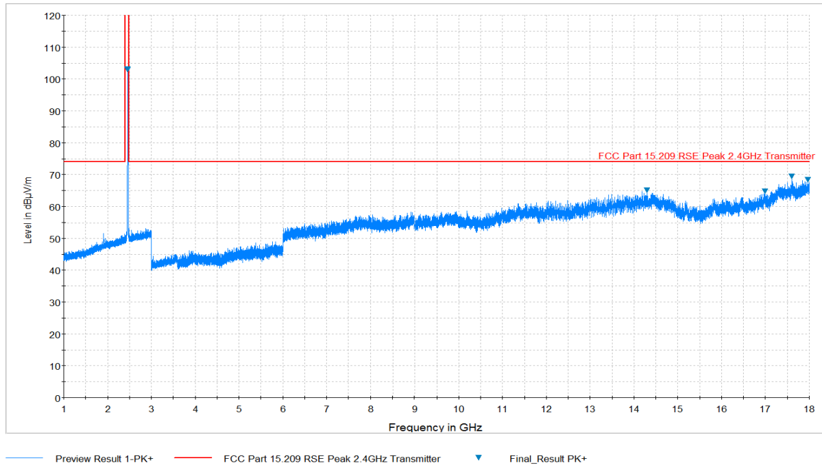
Plot 7-35. Radiated Spurious Plot above 1GHz (802.11b – Ch. 11, Ant. Pol. H)
