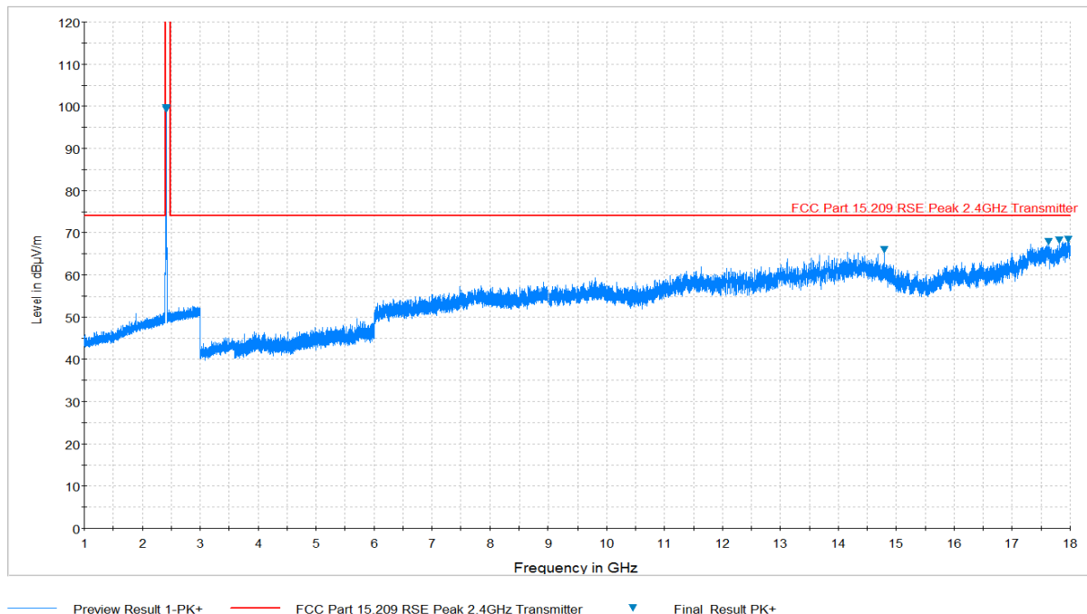
Plot 7-32. Radiated Spurious Plot above 1GHz (802.11b – Ch. 1, Ant. Pol. V)
