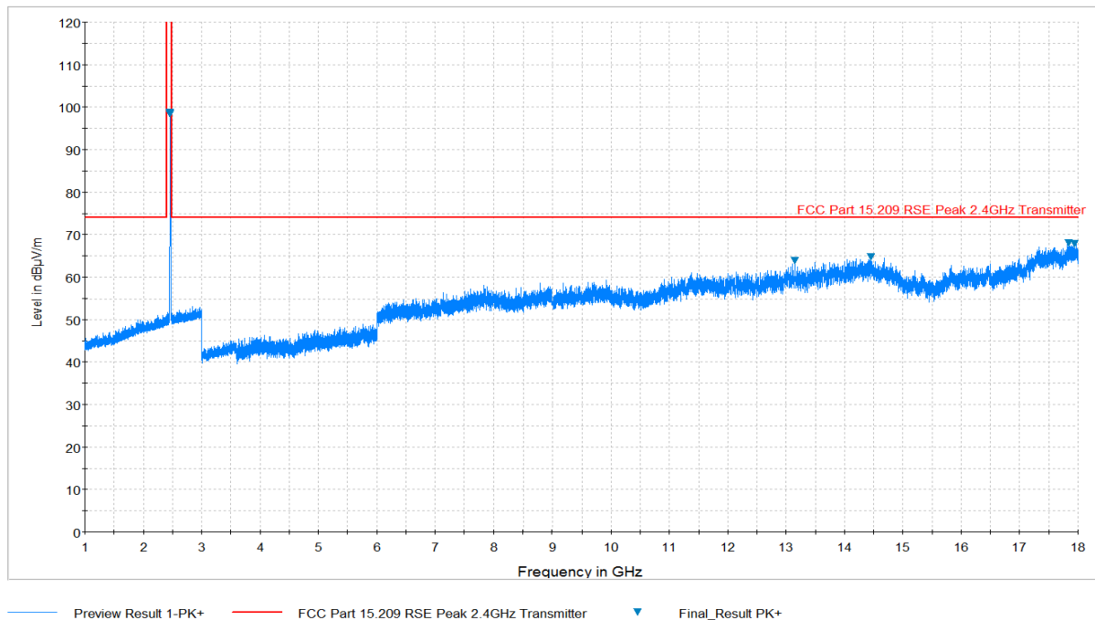
Plot 7-36. Radiated Spurious Plot above 1GHz (802.11b – Ch. 11, Ant. Pol. V)
