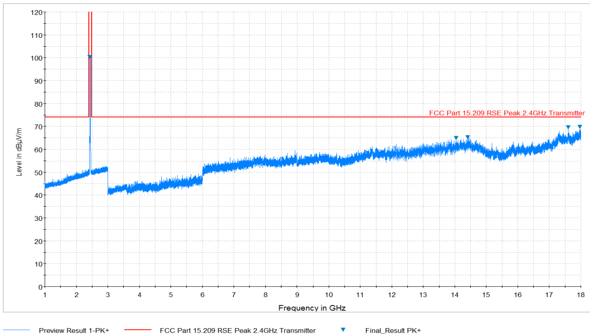
Plot 7-34. Radiated Spurious Plot above 1GHz (802.11b – Ch. 6, Ant. Pol. V)
