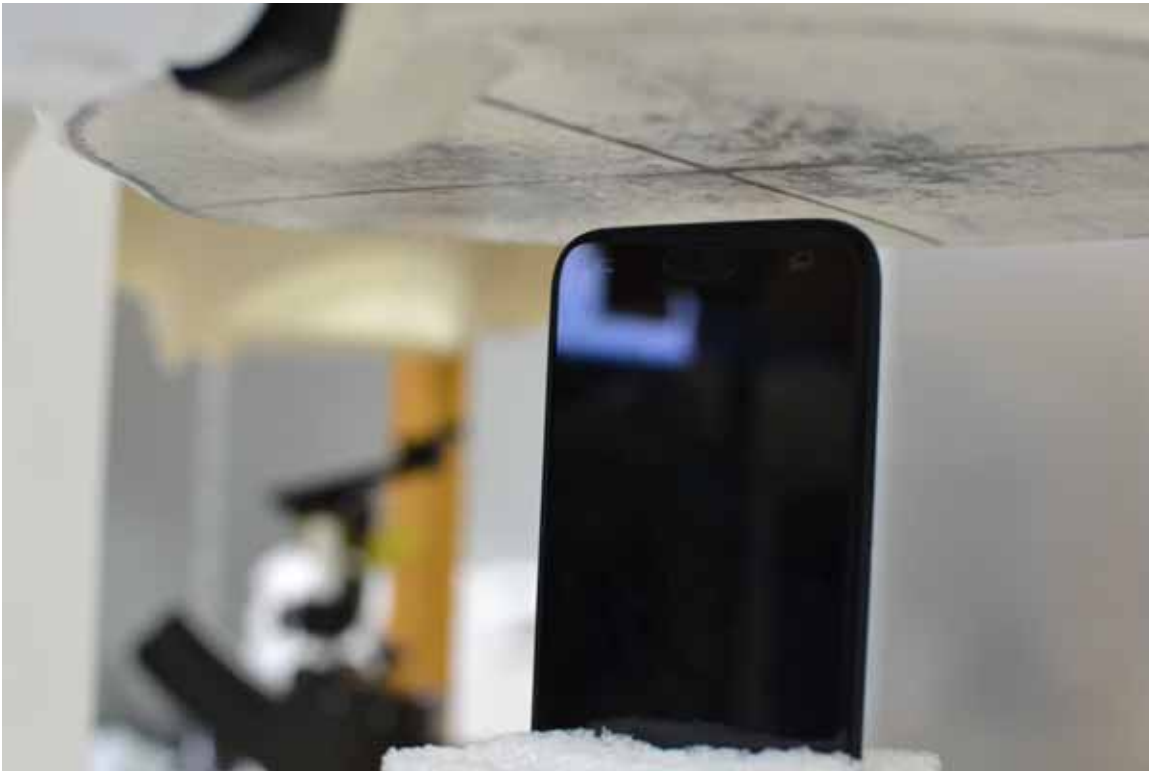
SAR Test Setup Photo 9 – Bottom Edge at 10 mm
